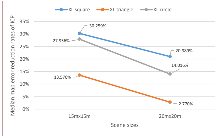
Figure 5-17. Median map error reduction rates of ICP for XL-sized trajectories (square, triangle, circle) across two different scene sizes ( 15m \times 15m , 20m \times 20m ).
