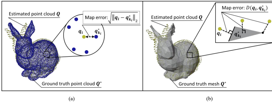
Figure 4-2. Error metrics for evaluating mapping performance. When the estimated map Q is represented as a point cloud, the choice of error metric depends on the representation format of the ground truth map Q^* . (a) If the ground truth map Q^* is also represented as a point cloud, the mapping error metric RMSE_{map\_pointcloud} is computed as the root mean square error of the nearest-neighbour distances. Specifically, for each point q_i in the estimated map Q , the distance to its nearest neighbouring point q_{k_i}^* in the ground truth map Q^* is measured, and the RMSE of all these distances is used as the error metric. (b) If the ground truth map Q^* is represented as a mesh, the evaluation metric RMSE_{map\_mesh} is defined as the root mean square error of the point-to-mesh distances. For each point q_i in the estimated point cloud Q , the distance D(q_i, q_{k_i}^*) to its nearest neighbouring triangle in the ground truth mesh Q^* is computed. The point-to-triangle distance D(q_i, q_{k_i}^*) depends on the spatial relationship between q_i and the triangle. If the projection of q_i onto the triangle's plane falls within the triangle, D(q_i, q_{k_i}^*) is the length of the normal vector. Otherwise, it corresponds to the shortest distance to the closest triangle edge or vertex. (a) When the ground truth map is a point cloud, the error is computed as the RMSE of nearest-neighbour point distances. (b) When the ground truth map is a mesh, the error is computed as the RMSE of point-to-mesh distances.
