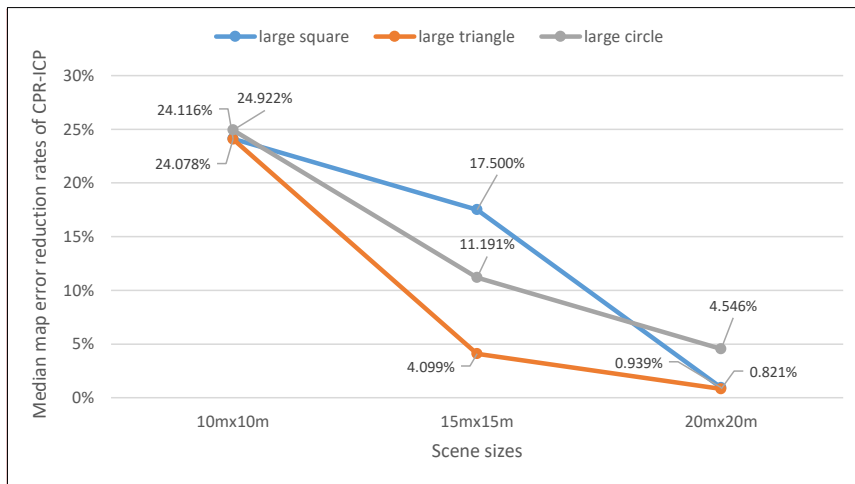
Figure 5-19. Median map error reduction rates of CPR-ICP for large-sized trajectories (square, triangle, circle) across three different scene sizes ( 10m \times 10m , 15m \times 15m , 20m \times 20m ).
