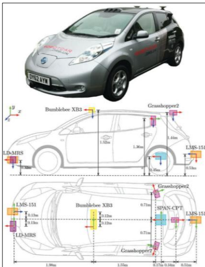
Figure 2-7. Example-h hardware setup used for vision-LiDAR fusion in the Oxford RobotCar dataset [102]. The sensors in this configuration include a Point Grey Bumblebee XB3 (BBX3-13S2C-38) trinocular stereo camera, three Point Grey Grasshopper2 (GS2-FW-14S5C-C) monocular cameras, two SICK LMS-151 2D LiDAR sensors, and one SICK LD-MRS 3D LiDAR sensor.
