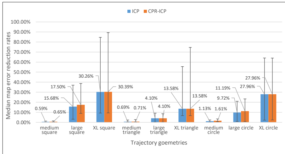
Figure 5-12. Median map error reduction rates of ICP and CPR-ICP operations for each type of trajectory geometry used in 15m \times 15m \times 2m cuboid scene.
