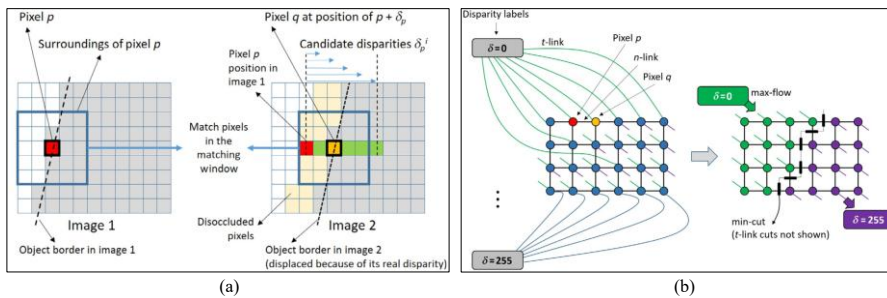
Figure 2-38. Overview of the stereo correspondence methods (Chellappa et al. [167]). (a) Local method using a sliding-window approach. For each pixel p in image 1, its disparity is determined by comparing its intensity with N candidate pixels in image 2 within a sliding window. The candidate pixel in image 2 with the lowest matching cost is assigned as the corresponding match for pixel p . (b) Global method based on the graph-cut technique. A graph is constructed and partitioned into N subgraphs, where each pixel in a subgraph is assigned a disparity label following a specific pattern. This pattern is associated with a matching cost function, and the objective is to determine the disparity labels that minimize the total matching cost function across all subgraphs.
