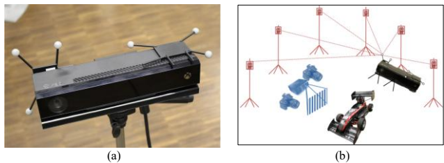
Figure 2-24. Example hardware setup of a MoCap system used in a SLAM benchmark to acquire the ground truth trajectory of a mobile platform (Wasenmüller et al. [108]). (a) Similar to the setup shown in Figure 2-23 (a), a Microsoft Kinect V2 sensor is equipped with multiple markers, enabling MoCap cameras to accurately track its trajectory. (b) Overview of the experimental setup and operational principle of the proposed SLAM benchmark.
