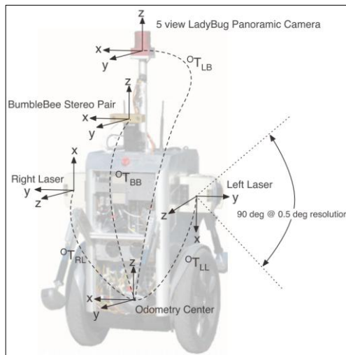
Figure 2-6. Example of a hardware setup for vision-LiDAR fusion used in the New College dataset [93]. This setup includes a LadyBug panoramic camera, a Bumblebee stereo camera, and two SICK LMS 291-S14 2D LiDAR sensors.
