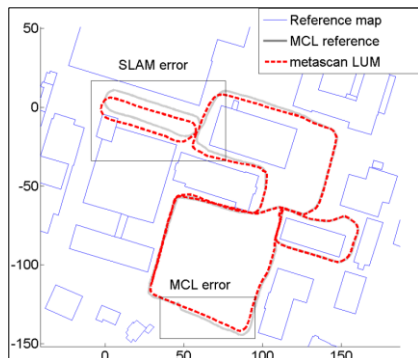
Figure 2-29. Evaluation of the localization performance of the SLAM algorithm using Monte Carlo Localization (MCL) and a reference map (Wulf et al. [100]). The blue line represents the high-precision reference map, the red dotted line indicates the trajectory estimated by the SLAM algorithm, and the grey line shows the ground-truth trajectory obtained using Monte Carlo Localization (MCL) aligned with the high-precision reference map.
