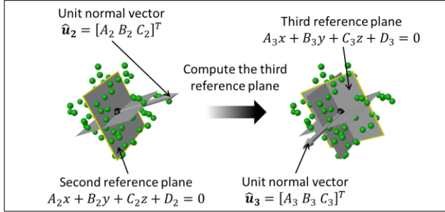
Figure 4-9. Illustration of the process of acquiring the third reference plane based on the first and second reference planes. Since the third reference plane is perpendicular to the first and second reference planes, and the column vectors of matrix U are mutually orthogonal, its unit normal vector \hat{u}_3 = [A_3 \ B_3 \ C_3]^T of the third reference plane can be directly derived from U . As the third reference plane also passes through the point cloud centroid, the final unknown parameter D_3 in the plane equation A_3x + B_3y + C_3z + D_3 = 0 is determined by substituting the centroid coordinates into the equation. This completes the formulation of the third reference plane equation.
