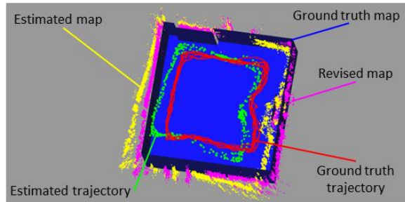
Figure 6-7. Trial outputs and ground truth map for large-scale scene experiments. The outputs include point clouds of the estimated trajectory, ground truth trajectory, estimated map, and the revised map after accuracy improvement. The ground truth map, represented as a pre-constructed CAD mesh model, was readily available for benchmarking.
