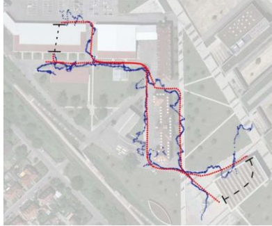
Figure 2-30. Comparison of trajectories obtained using GPS (blue line) and Monte Carlo Localization (MCL) combined with aerial imagery (red line) (Kümmerle et al. [99]). As illustrated, the trajectory estimated by MCL with aerial imagery is notably more accurate than the trajectory obtained solely from GPS data.
