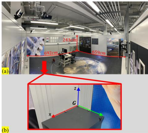
Figure 6-6. Experimental setup and configuration for the large-scale scene. (a) Panoramic view of the large-scale room. (b) Global coordinate frame and ground truth map. Following the same experimental setup as the medium-scale scene, the global coordinate frame G was positioned at the corner where two walls intersect. The room's dimensions and geometry relative to G were manually measured to construct the CAD mesh model used as the ground truth map.
