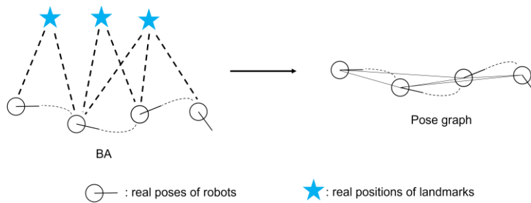
Figure 1-3. Illustration of BA and pose graph. Positions of landmarks are considered as constraints between poses in the pose graph, saving both computational time and resources.
