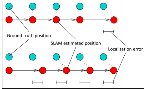
Figure 2-34. Illustration demonstrating why directly comparing elements of the estimated trajectory to the ground-truth trajectory is suboptimal for evaluating localization benchmarks (Kümmerle et al. [99]). As depicted, the upper scenario shows a local error between estimated and ground-truth trajectories occurring near the end, resulting in a relatively small global localization error. Conversely, the lower scenario illustrates the same magnitude of local error occurring near the beginning of the trajectory, which accumulates significantly by the end, causing a much larger global localization error. This indicates that identical local errors can yield substantially different global errors depending on their positions along the trajectory, making direct element-wise comparisons between estimated and ground-truth trajectories unsuitable as an evaluation metric for localization accuracy.
