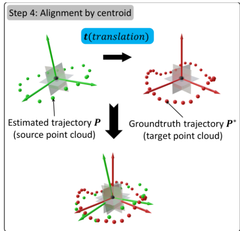
Figure 4-16. Fourth step of trajectory error minimization: aligning the estimated trajectory point cloud P with the ground truth trajectory point cloud P^* by their centroids. The corresponding translation matrix t is then obtained, which will be used in the map error reduction step.
