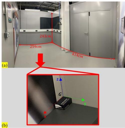
Figure 6-4. Experimental setup and configuration for the medium-scale scene. (a) Panoramic view of the medium-scale room. (b) Global coordinate frame and ground truth map. The global coordinate frame G was established at the corner where two walls meet. The room's relative dimensions and geometry were manually measured with respect to G to construct the CAD mesh model used as the ground truth map.
