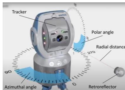
Figure 2-26. Illustration of the working principle of a laser tracker (FARO Vantage model) [136]. The laser tracker measures the 3D coordinates of an object by tracking a retroreflector target attached to it. It emits a laser beam towards the retroreflector target and receives the reflected beam, enabling the calculation of radial distance based on the time difference between emission and reflection. Simultaneously, the tracker measures the polar and azimuth angles of the retroreflector target using two internal angle encoders. These measurements—radial distance, polar angle, and azimuth angle—are combined to accurately determine the 3D position of the retroreflector target within the laser tracker's spherical coordinate system.
