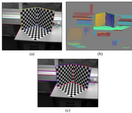
Figure 2-19. Example illustrating a feature-based approach for calibrating cameras and range sensors, as proposed by Moghadam et al. [119]. Linear features (line segments) are extracted from the 3D point cloud obtained by the range sensor and from the 2D image captured by the camera to establish correspondences. (a) Line segments extracted from the camera's 2D image using the Canny edge detector. (b) Line segments (including plane intersections and boundary lines) extracted from the 3D point cloud using a region-growing strategy. (c) Resulting aligned line segments after registration: The blue lines represent matched line segments from the 2D image, while the red lines indicate the projection of corresponding 3D point cloud line segments onto the 2D image.
