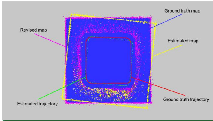
Figure 5-6. Outputs of each trial and the ground truth map. The outputs include the estimated trajectory as a point cloud, the ground truth trajectory, the estimated map, and the revised map after applying the mapping accuracy improvement method. The ground truth map is represented as a mesh model.
