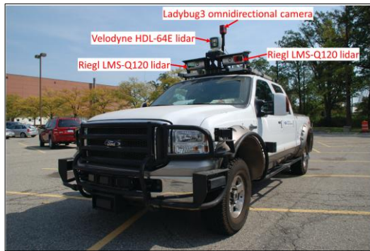
Figure 2-12. Example hardware setup for vision-LiDAR fusion used in the Ford Campus dataset [95]. The sensors in this configuration include a Ladybug3 omnidirectional camera, two Riegl LMS-Q120 2D laser scanners, and a Velodyne HDL-64E 3D LiDAR sensor.
