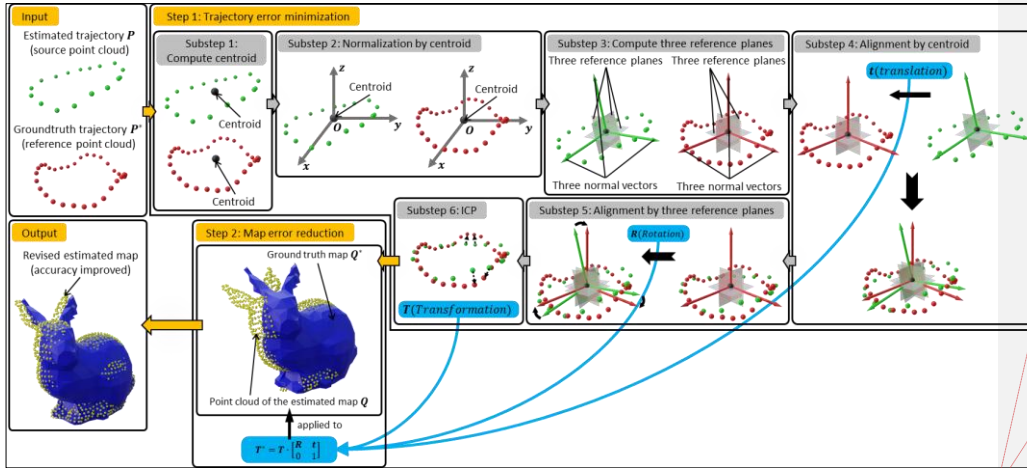
Figure 4-20. Complete workflow for mapping accuracy enhancement. The workflow consists of two main steps: trajectory error minimization and map error reduction. The first step, trajectory error minimization, employs a novel ICP variant called CPR-ICP (Centre Point Registration ICP). This step is divided into six substeps: (1) computing the centroid, (2) centroid-based normalization, (3) computing three reference planes, (4) alignment by centroid, (5) alignment by three reference planes, and (6) classic ICP operation. The first five substeps constitute the CPR operation, followed by the final ICP step. The second step, map error reduction, applies the Euclidean transformations derived from Substeps 4, 5, and 6 of the first step to the estimated map Q , resulting in the refined estimated map \hat{Q} with improved accuracy.
