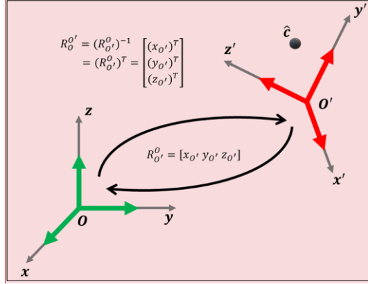
Figure 3-1. Transformation between two coordinate frames.
