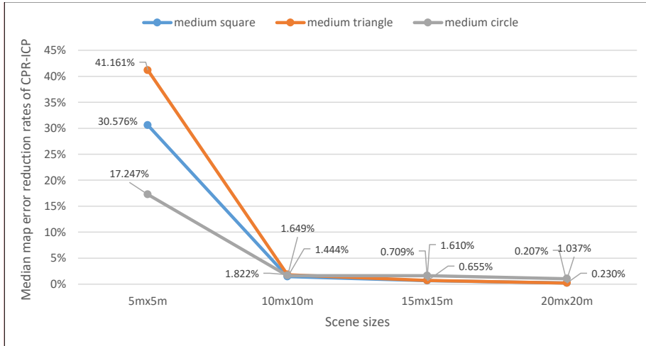
Figure 5-18. Median map error reduction rates of CPR-ICP for medium-sized trajectories (square, triangle, circle) across all four different scene sizes ( 5m \times 5m , 10m \times 10m , 15m \times 15m , 20m \times 20m ).
