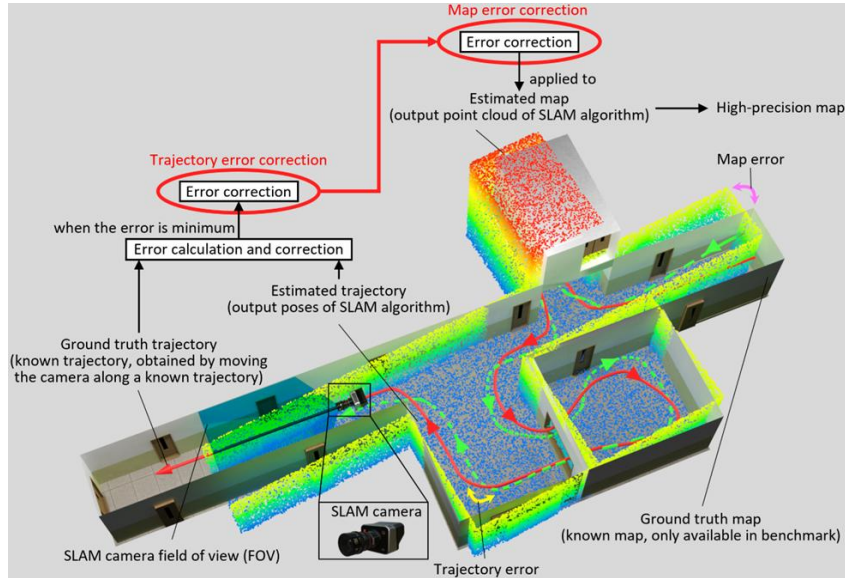
Figure 4-3. Concept of mapping accuracy enhancement. The comprehensive SLAM benchmark introduced in the previous chapter highlights the intrinsic relationship between localization and mapping. The proposed approach to improving mapping accuracy leverages this relationship by directly applying localization error reduction methods to mapping. This is formulated as a numerical optimization problem aimed at minimizing errors in both localization and mapping. The process involves first computing a numerical optimization that minimizes trajectory error (yellow two-way arrow curve) by aligning the estimated trajectory (dashed green arrow) with the ground truth trajectory (solid red arrow). This optimization is then applied directly to the estimated map (colorized point cloud) to refine its accuracy, bringing it closer to the ground truth map (corridor CAD model).
