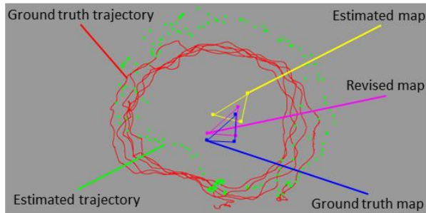
Figure 6-3. Trial outputs and ground truth map for small-scale scene experiments. The outputs include point clouds of the estimated trajectory, ground truth trajectory, estimated map, and the revised map after accuracy improvement. The ground truth map of the small-scale scene was pre-captured using the motion capture system and was readily available for benchmarking.
