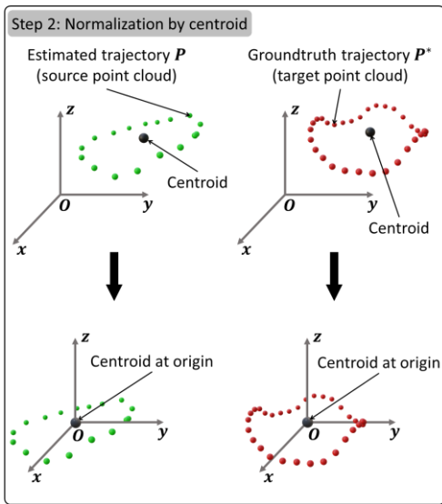
Figure 4-14. Second step of trajectory error minimization: normalizing each trajectory point cloud by its centroid. Each trajectory point cloud is centered at the origin by subtracting the centroid coordinates from the coordinates of all points in the point cloud.
