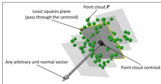
Figure 4-7. Illustration showing that the least squares plane corresponding to any arbitrary unit normal vector must pass through the centroid of the point cloud. Given a point cloud P (represented as a green point set), the plane that minimizes the sum of squared distances between each point in P and the plane must pass through the centroid of P . This plane, known as the least squares plane, is depicted as a solid grey square with a yellow boundary in the figure. In contrast, any parallel planes (shown
