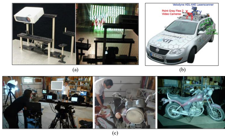
Figure 2-40. Equipment setups used for data collection in two-view stereo. (a) Setup from Scharstein et al. [172]: A digital camera mounted on a translating stage captured image pairs, while a structured-light projector positioned above uniquely labelled each pixel to facilitate correspondence estimation, serving as ground truth data. (b) The data collection platform for the KITTI dataset (Geiger et al. [111]): Designed for outdoor environments, this platform integrates LiDAR and multiple cameras with specialized calibration and registration techniques. (c) The data collection setup for the Middlebury high-resolution stereo dataset (Scharstein et al. [175]): Two DSLR cameras captured high-resolution images, and ground truth disparity images were generated using patterned-light projectors.
