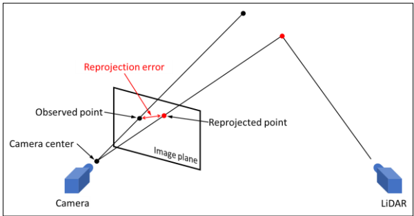
Figure 2-20. Illustration of the reprojection error concept used in camera–LiDAR calibration. A point in 3D space is simultaneously observed by both a camera and a LiDAR sensor. The real position of the point is shown in black, while the position measured by the LiDAR is depicted in red. Due to measurement errors inherent to the LiDAR sensor, there is a slight discrepancy between the measured and actual positions. Consequently, when projected onto the image plane, the LiDAR-measured point position differs from the position directly observed by the camera. The distance between these two positions on the image plane represents the reprojection error.
