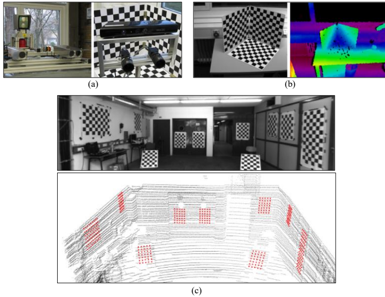
Figure 2-17. Example illustrating the use of checkerboard patterns for calibrating cameras and range sensors, as described by Geiger et al. [117]. (a) Two experimental setups demonstrating different camera and range sensor configurations: on the left, a Velodyne HDL-64E 3D LiDAR paired with a trinocular camera; on the right, a Microsoft Kinect depth camera paired with a binocular camera. (b) A camera image and the corresponding color-coded depth image of a checkerboard captured by the Microsoft Kinect depth camera. (c) Top: A camera image showing multiple checkerboards positioned at various locations; Bottom: Corresponding LiDAR data (3D point cloud) along with the resulting calibration.
