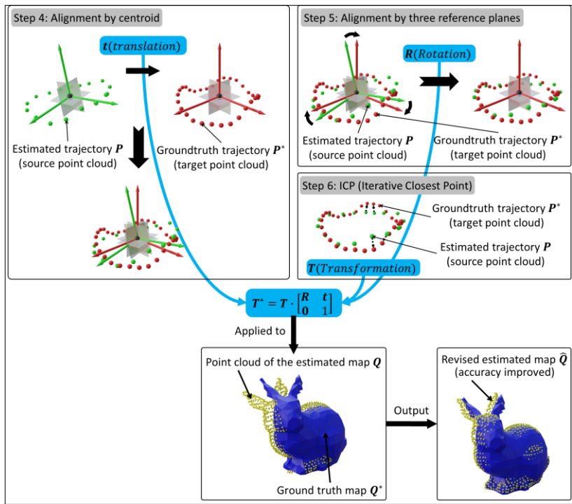
Figure 4-19. Final step: Map error reduction step. This is the final step in the workflow for improving mapping accuracy, following trajectory error minimization. In this step, the Euclidean transformation matrices t , R , and T , obtained in Steps 4, 5, and 6 of trajectory error minimization, are combined to form the transformation matrix T^* . The transformation T^* is then applied to the estimated map Q , producing the refined estimated map \hat{Q} with improved accuracy.
