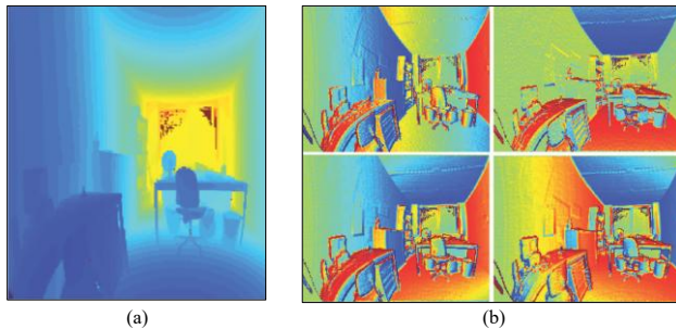
Figure 2-18. Example illustrating a feature-based approach for camera-LiDAR calibration, as presented by Scaramuzza et al. [118]. Correspondences between the 2D camera image and the 3D LiDAR data are established by matching features in the camera image with those in a 2D bearing-angle image (BA image), which is derived from the 3D range data. This approach simplifies the establishment of camera-LiDAR feature correspondences. (a) Color-coded depth image representing the 3D range data of a scene. (b) Bearing-angle images computed from the 3D range data at four different viewing angles, represented as 2D maps.
