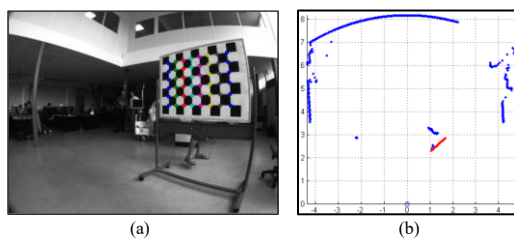
Figure 2-15. Example illustrating the use of a checkerboard pattern for camera-LiDAR spatial calibration, as presented by Kassir et al. [115]. (a) Demonstration of the algorithm extracting checkerboard corners from a camera image, with coloured dots representing the detected corners. (b) Demonstration of the algorithm extracting a straight line (red dotted line) from 2D laser scan data. The proposed extraction algorithms facilitate automatic camera-LiDAR calibration.
