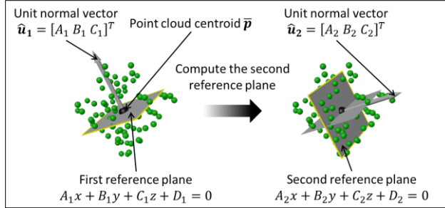
Figure 4-8. Illustration of the process of acquiring the second reference plane based on the first reference plane. Based on the workflow for obtaining the first reference plane shown in Figure 4-6, the unit normal vector \hat{\mathbf{u}}_2 = [A_2 \ B_2 \ C_2]^T of the second reference plane can be directly derived from the orthogonal matrix \mathbf{U} obtained through Singular Value Decomposition (SVD). Since the second reference plane must also pass through the point cloud centroid, the final unknown parameter D_2 in the plane equation A_2x + B_2y + C_2z + D_2 = 0 is determined by substituting the centroid coordinates into the equation. This results in the complete plane equation for the second reference plane.
