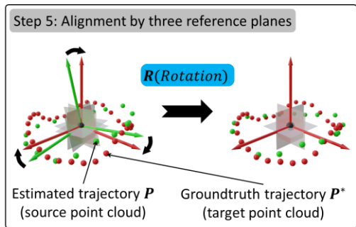
Figure 4-17. Fifth step of trajectory error minimization: rotating the translated point cloud of the estimated trajectory P around its centroid to align its three reference planes with the corresponding reference planes of the ground truth trajectory point cloud P^* . The resulting rotation matrix R is then obtained and will be used in the map error reduction step.
