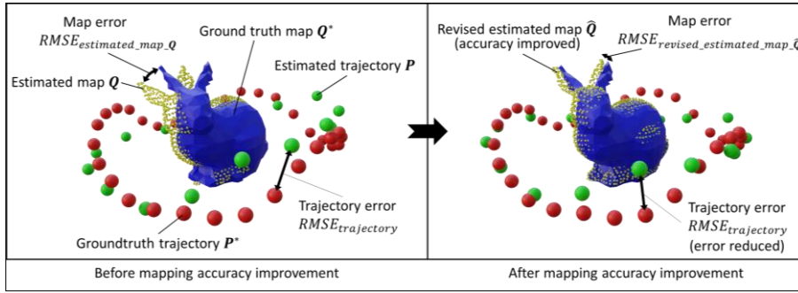
Figure 4-21. Visualization of the effect of mapping accuracy enhancement. The mapping error before and after applying the accuracy enhancement method is represented by RMSE_{estimated\_map\_Q} and RMSE_{revised\_estimated\_map\_Q} , respectively. After implementing the mapping accuracy enhancement process, both the trajectory error RMSE_{trajectory} and the map error are reduced, resulting in RMSE_{revised\_estimated\_map\_Q} < RMSE_{estimated\_map\_Q} . Consequently, a revised map, denoted as \hat{Q} , with improved accuracy is obtained.
