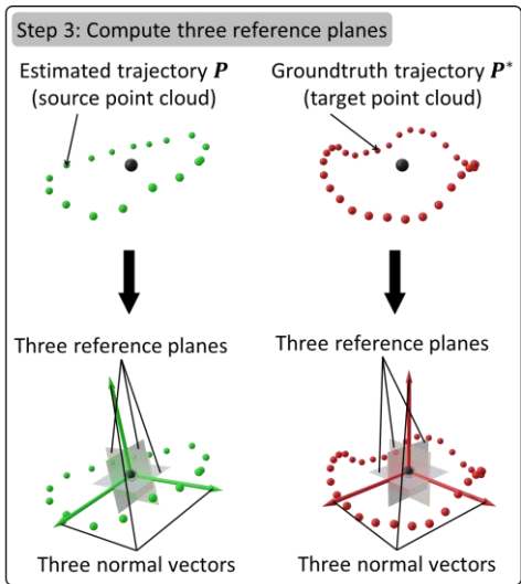
Figure 4-15. Third step of trajectory error minimization: computing the three reference planes of each trajectory point cloud. This is achieved by applying Singular Value Decomposition (SVD) to the normalized trajectory point cloud.
