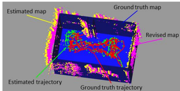
Figure 6-5. Trial outputs and ground truth map for medium-scale scene experiments. The outputs include point clouds of the estimated trajectory, ground truth trajectory, estimated map, and the revised map after accuracy improvement. The ground truth map, represented as a CAD mesh model, was pre-constructed and readily available for benchmarking.
