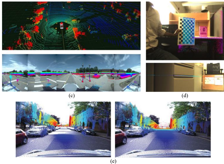
Figure 2-21. Examples illustrating qualitative evaluations of camera-LiDAR calibration accuracy by projecting LiDAR-captured points onto camera images. (a) Projection of edge points extracted from LiDAR data (shown in red), representing depth discontinuities, onto a monocular image using the computed Euclidean transformation to qualitatively assess the accuracy of camera-LiDAR calibration (Scaramuzza et al. [118]). (b) Projection of depth-based, color-coded 3D points captured by a Velodyne LiDAR onto a monocular image using the computed Euclidean transformation to qualitatively assess the accuracy of camera-LiDAR calibration (Geiger et al. [111]). (c) Top: A frame of 3D point cloud captured by the LiDAR; bottom: The corresponding projection of color-coded LiDAR points onto the panorama image using the computed Euclidean transformation to visually assess calibration accuracy with the computed transformation (Pandey et al. [116]). (d) Projection of depth-based, color-coded points from a time-of-flight 3D camera and a 2D LiDAR onto a monocular image using the computed Euclidean transformation It is used for qualitative evaluation of mutual information (MI)-based calibration (Pandey et al. [126]). (e) Comparison between projections of a 3D LiDAR point cloud onto a monocular image using poses estimated by an Inertial Navigation System (INS) and visual odometry, respectively The comparison shows that in regions with weak GPS signals, the INS-based pose estimation suffers interruptions, resulting in inaccurate local 3D point clouds. Visual odometry, on the other hand, provides smoother local pose estimates but exhibits drift over longer distances (Maddern et al. [102]).
