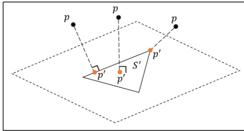
Figure 2-35. Illustration of the distance between a point and a triangle plane in a mesh model. [The distance from a point p to a triangle S' is defined as the shortest distance between p and the closest point p' on the triangle S' . Based on the positional relationship between the point and the triangle, this point-to-triangle distance can be classified into three cases: (1) If the projection of point p onto the plane containing triangle S' lies within the triangle, the distance is measured from p directly to
