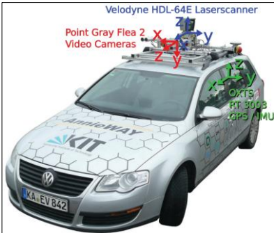
Figure 2-11. Example hH hardware setup for vision-LiDAR fusion used in the KITTI dataset [111]. This setup includes two PointGrey Flea2 grayscale cameras (FL2-14S3M-C), two PointGrey Flea2 color cameras (FL2-14S3C-C), and one Velodyne HDL-64E 3D LiDAR sensor.
