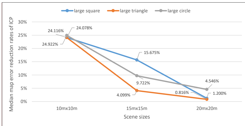
Figure 5-16. Median map error reduction rates of ICP for large-sized trajectories (square, triangle, circle) across three different scene sizes (10m × 10m, 15m × 15m, 20m × 20m).
