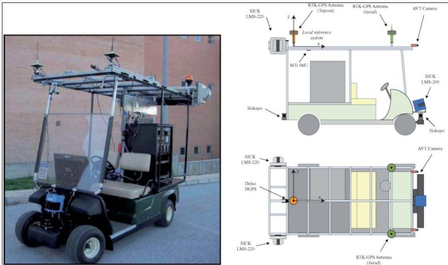
Figure 2-9. Example hardware setup for vision-LiDAR fusion used in the Málaga dataset [94]. This configuration includes two Hokuyo UTM-30LX laser rangefinders, two SICK LMS-220 laser rangefinders, one SICK LMS-200 laser rangefinder, and two AVT Marlin F-131C color cameras.
