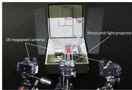
Figure 2-31. The 3D structured-light scanner used in the CoRBS dataset [108] performing a scan of an electrical cabinet. The scanner consists of a structured-light projector and two 18-megapixel cameras. The projector casts a fringe pattern onto the surface of the object, while the two cameras capture distortions in the projected pattern. These captured distortions are then used to reconstruct the object's geometry with high precision through triangulation.
