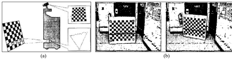
Figure 2-14. Example of using a checkerboard pattern for camera-LiDAR spatial calibration, following the method proposed by Zhang et al. [112]. (a) Illustration of the experimental setup consisting of a camera and a 2D laser range finder. (b) Projection of points acquired by the 2D laser range finder onto images captured by the camera at two different sensor poses. The collected sensor data were subsequently used to impose geometric constraints, enabling the calculation of extrinsic calibration parameters.
