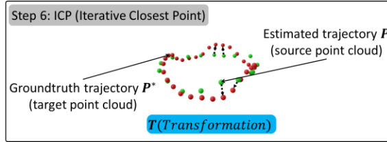
Figure 4-18. The sixth step of trajectory error minimization—applying the classic ICP (Iterative Closest Point) algorithm to the point cloud of the estimated trajectory P to further reduce the error between it and the point cloud of the ground truth trajectory P^* . The transformation matrix T is also acquired in this step and it will be used in the step of map error reduction.
