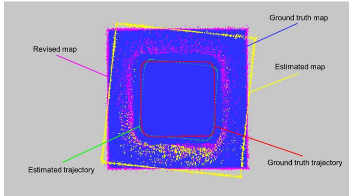
Figure 5-6. Outputs of each trial and the ground truth map. The outputs include the estimated trajectory as a point cloud, the ground truth trajectory, the estimated map, and the revised map after applying the mapping accuracy improvement method. The ground truth map is represented as a mesh model.
