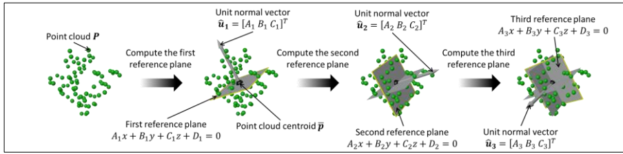
Figure 4-10. Workflow for acquiring the three mutually orthogonal reference planes. Eq. (5.5), Eq. (5.6) and Eq. (5.7) show that for any arbitrary normal vector, the cost function in Eq. (5.3) reaches its minimum when the corresponding plane passes through the point cloud centroid. This implies that all three reference planes must pass through the centroid. Therefore, by applying centroid normalization and Singular Value Decomposition (SVD) to the point cloud, the mathematical computations can be simplified. The unit normal vector of the first reference plane, \hat{u}_1 = [A_1 \ B_1 \ C_1]^T , is obtained first and corresponds to the last column vector of the orthogonal matrix U produced by the SVD factorization. Next, based on \hat{u}_1 , the unit normal vector of the second reference plane, \hat{u}_2 = [A_2 \ B_2 \ C_2]^T , is determined, which corresponds to the second-to-last column vector of U . Since the three reference planes are mutually orthogonal, the unit normal vector of the third reference plane, \hat{u}_3 , is computed as the cross product of \hat{u}_1 and \hat{u}_2 , which corresponds to the first column vector of U . Once the unit normal vectors of all three reference planes are obtained, the final unknown parameters D_1 , D_2 and D_3 are determined by substituting the centroid coordinates into their respective plane equations. This process results in the complete formulation of the equations for all three reference planes.
