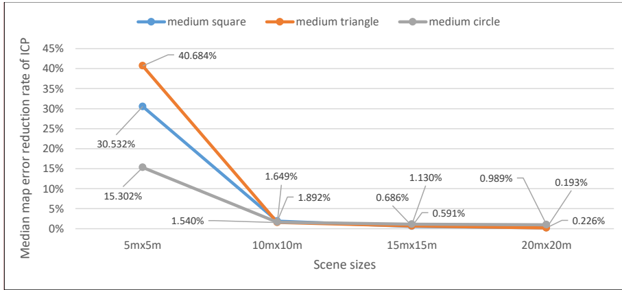
Figure 5-15. Median map error reduction rates of ICP for medium-sized trajectories (square, triangle, circle) across all four different scene sizes (5m × 5m, 10m × 10m, 15m × 15m, 20m × 20m).
