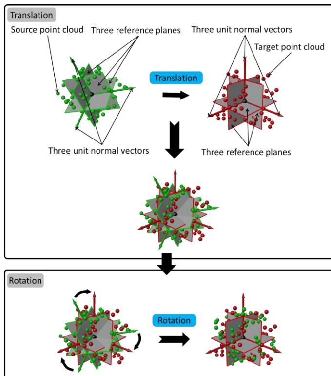
Figure 4-11. Alignment of the source point cloud to the target point cloud using their three reference planes. The alignment is performed through a translation followed by a rotation. First, the source point cloud is translated so that its centroid aligns with that of the target point cloud. Then, it is rotated around its centroid until its three reference planes coincide with the corresponding reference planes of the target point cloud.
