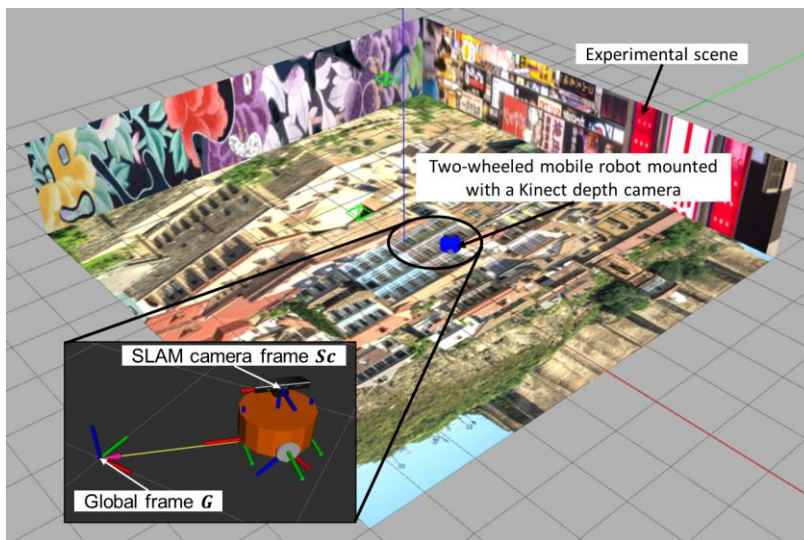
Figure 5-1. Simulation setup in Gazebo.
