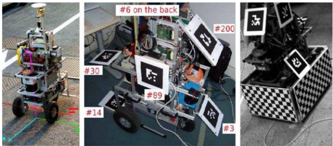
Figure 2-25. Example hardware setup illustrating the use of fiducial markers for acquiring the ground truth trajectory of a robotic platform (RAWSEEDS project [135]). The robot is equipped with multiple fiducial markers, continuously observed by a network of stationary video cameras to determine marker poses relative to the camera reference frame. By establishing the relationships between the camera reference frame, the world reference frame, and the robot's marker reference frame, the Perspective-N-Point (PnP) technique is applied to calculate the pose of the robot with respect to the global (world) reference frame.
