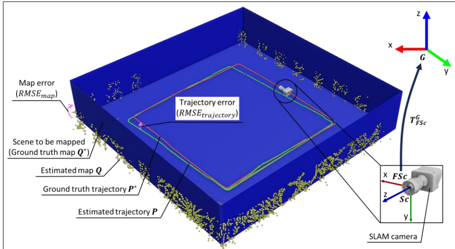
Figure 4-1. Illustration of the benchmark methodology. The estimated trajectory P and estimated map Q are generated by the SLAM algorithm and are initially defined within the SLAM camera frame ( Sc ) of the first image in the captured sequence, denoted as FSc . For benchmarking, they must be transformed into the global frame G using the Euclidean transformation T_{FSc}^G . Similarly, the ground truth trajectory P^* and ground truth map Q^* are recorded in their respective reference frames and must also be transformed into the global frame G to enable direct comparison with P and Q .
