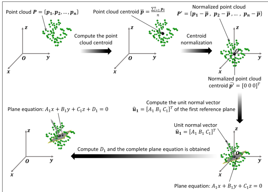
Figure 4-6. Workflow for acquiring the first reference plane of the point cloud P . First, the centroid \bar{p} of the point cloud is computed, and centroid normalization is applied. This step reduces the number of unknowns in the cost function f(\hat{u}_1, D_1) from two (\hat{u}_1, D_1) to one (\hat{u}_1) , simplifying the mathematical calculations. Next, the unit normal vector \hat{u}_1 = [A_1 \ B_1 \ C_1]^T of the first reference plane is determined by applying Singular Value Decomposition (SVD) to the centroid-normalized point cloud. Finally, since the reference plane must pass through the point cloud centroid, the last unknown D_1 in the plane equation A_1x + B_1y + C_1z + D_1 = 0 is computed by substituting the centroid coordinates into the equation. This results in the final equation of the first reference plane.
