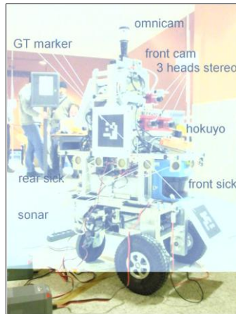
Figure 2-8. Example h1 hardware setup for vision-LiDAR fusion used in the RAWSEEDS project [88]. This setup consists of an omnidirectional camera, a trinocular stereo camera, a HOKUYO laser range scanner, and a SICK laser range scanner.
