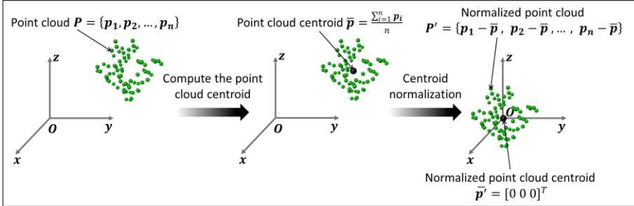
Figure 4-5: Centroid normalization of the point cloud P . The point cloud P is normalized by subtracting its centroid \bar{p} = \frac{\sum_{i=1}^n p_i}{n} from each point p_i , resulting in a normalized point cloud P' with a centroid p' positioned at the origin [0 \ 0 \ 0]^T . When the partial derivative of the cost function f(\hat{u}_1, D_1) with respect to D_1 equals zero, the variable D_1 satisfies D_1 = \hat{u}_1^T \bar{p} . This indicates that regardless of the unit normal vector \hat{u}_1 of the first reference plane, the least-squares plane of the point cloud must pass through its centroid. Consequently, normalizing the point cloud by its centroid \bar{p} translates the least-squares plane to pass through the origin [0 \ 0 \ 0]^T . This transformation reduces the number of unknowns in the cost function f(\hat{u}_1, D_1) from two variables to a single variable \hat{u}_1 , thereby simplifying the mathematical operations.
