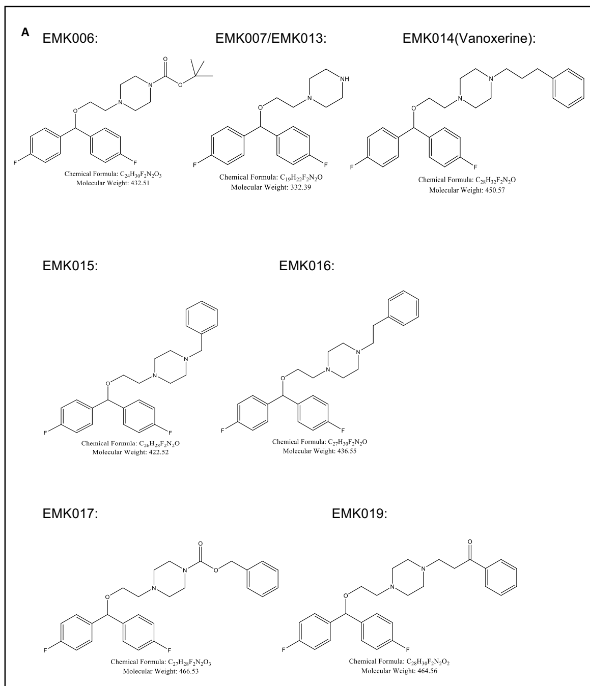
Figure 11. Chemical structures of vanoxerine analogues. Also referred to as "EMK compounds".
