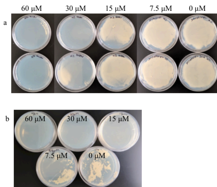
Figure 9. Attempts to generate vanoxerine-resistant mutants in M. bovis BCG. Plates contained 60 \mu M, 30 \mu M, 15 \mu M, 7.5 \mu M and 0 \mu M vanoxerine as the MIC used was determined in a previous study as 7.5 \mu M (Christopher Burke, University of Birmingham).
