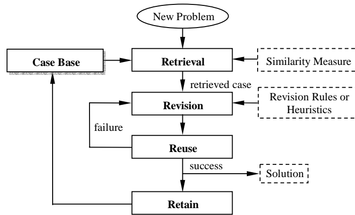
Figure 1 A Case-Based Reasoning Framework
