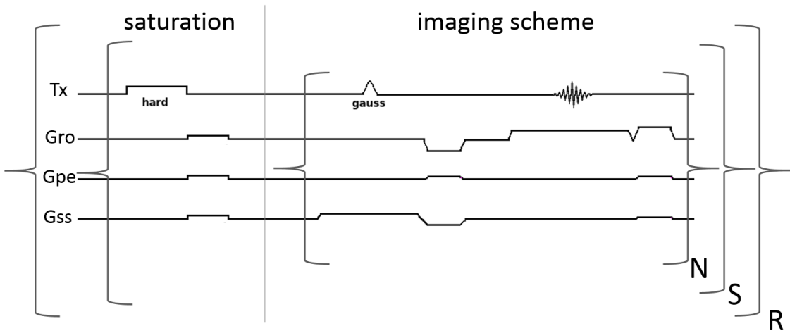
Figure 5.7: Diagram of the CEST sequence.: The saturation consisted of a single hard pulse (1.6 s, 0.9 \mu\text{T} ). After this pulse, a crusher gradient was applied to spoil the residual transverse magnetization. Following the first saturation module, N=64 lines of k space were acquired with a single slice gradient echo (CINE) imaging scheme. Centric encoding, RF and gradient spoiling were used, with S being the number of segments (2). This process was then repeated for R=40 CEST images (40 offsets between \pm 4 ppm). 15^\circ flip angle, \text{TE} = 1.57 ms, \text{TR} = 3.15 ms, 8 dummy scans, \text{FOV} = 20 \times 20 mm, 2 mm slice thickness.
