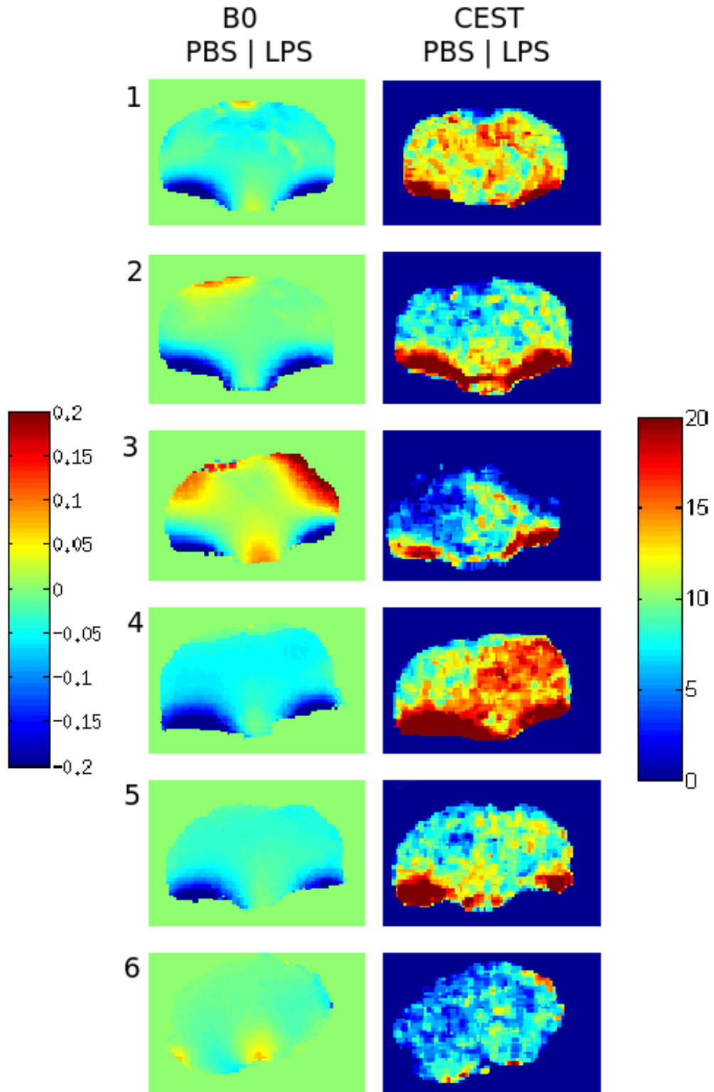
Figure 5.13: Individual data from the pilot study, CEST contrast with LPS (n=6).
