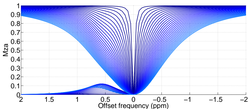
Figure 4.10: Z spectra and MTR_{asym} dependence on B_1 power, for a CW saturation of 7 s. B_1 power range: 0 to 3 \mu\text{T} .
