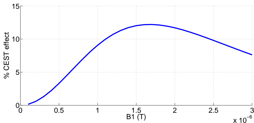
Figure 4.11: % CEST effect dependence on B_1 power, for a CW saturation of 7 s. Like in Figure 4.1, there is a trade off between saturation of the bound protons and spillover effects, with the optimum B_1 value being 1.7 \mu\text{T} .
