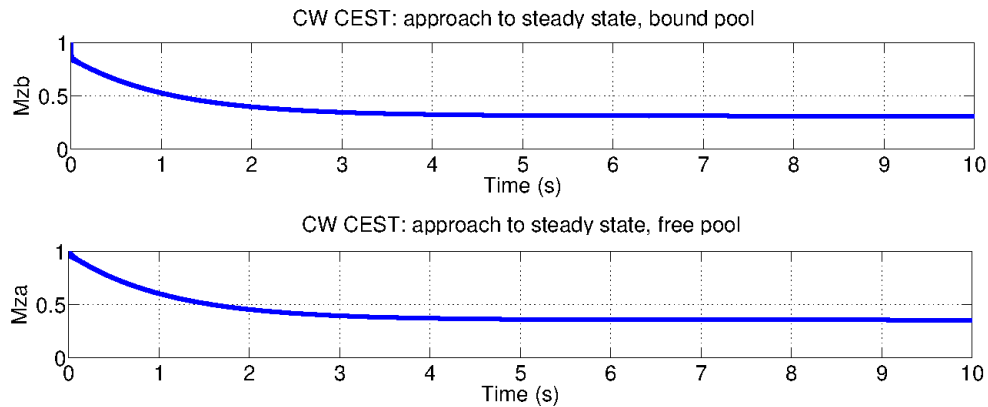
Figure 4.14: Evolution of the magnetization of the myo-inositol and water protons during a B_1 saturation power of 0.9 \mu T. From the top, the two graphs represent the z (longitudinal magnetization) component of myo-inositol (bound pool) and water (free pool). Since B_1 is smaller than in the long T_2 model, the hydroxyl protons get even less saturated in this case. The bottom graph represents the source of MRI signal, getting saturated through chemical exchange with the bound protons. The steady state is reached faster than in the long T_2 model, but the saturation is smaller (short T_2 model).
