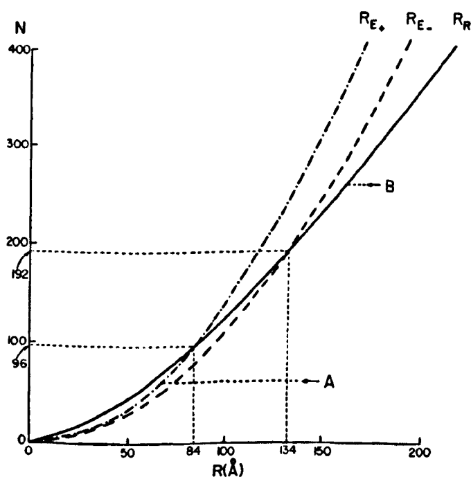
Figure 1.1.6 Critical droplet radius ( R_{E+} for large clusters, R_{E-} for small clusters) and Rayleigh instability ( R_R ). N : the number of elementary charges in the drop; A : the evaporating drop reaches ion evaporation limit first; B : the evaporating drop reaches Rayleigh limit first and therefore is disrupted. Adapted from [28].
