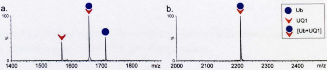
Figure 4.2.2 ESI mass spectra of quadrupole isolated Ub•UQ1-UBA complex charge states (a) 8+ and (b) 6+ of Ub (0.5 \mu M ) and UQ1-UBA (4 \mu M ) complex
