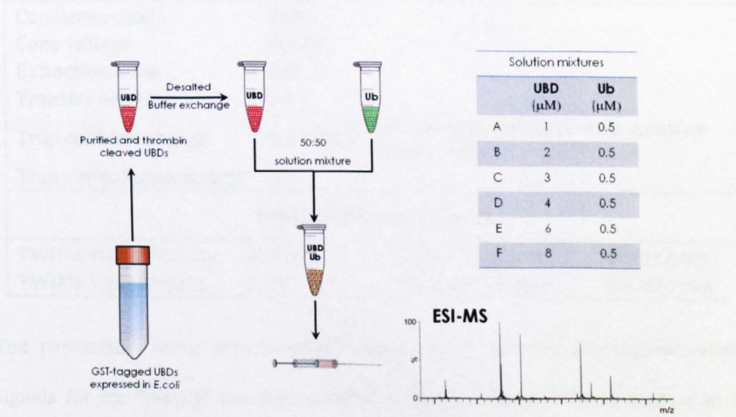
Figure 2.2.3 Procedure flowchart of the titration MS experiments
