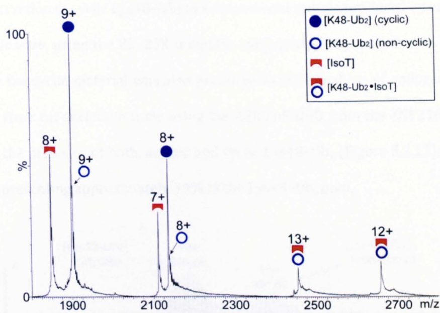
Figure 5.2.11 ESI-MS of 1 \mu M Lys48-Ub 2 (Lot#3291529) and 2 \mu M IsoT-ZnF sprayed from 25 mM ammonium acetate, showing that only the acyclic population of Lys48-Ub 2 is capable of forming complex.
