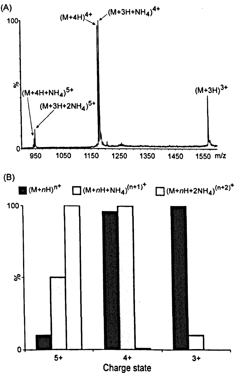
Figure 6.2.1 The charge state distribution of protonated and ammonium adducted ions (A) ESI mass spectrum of UQ1-UBA domain sprayed form 25 mM ammonium acetate and (B) graphical representation of the relative intensity of protonated and ammonium adducted ions at each charge state
