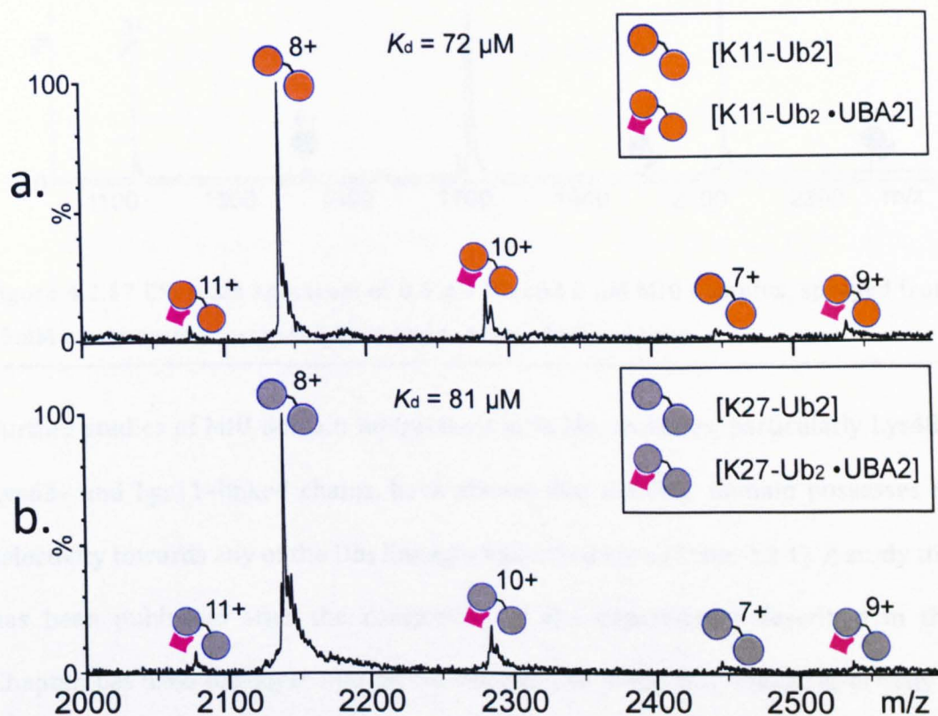
Figure 4.2.16 ESI mass spectra of UBA2 (4 \mu\text{M} ) with: a) Lys11-linked Ub 2 (0.5 \mu\text{M} ), b) Lys27-linked Ub 2 (0.5 \mu\text{M} ), sprayed from 25mM ammonium acetate solution.
