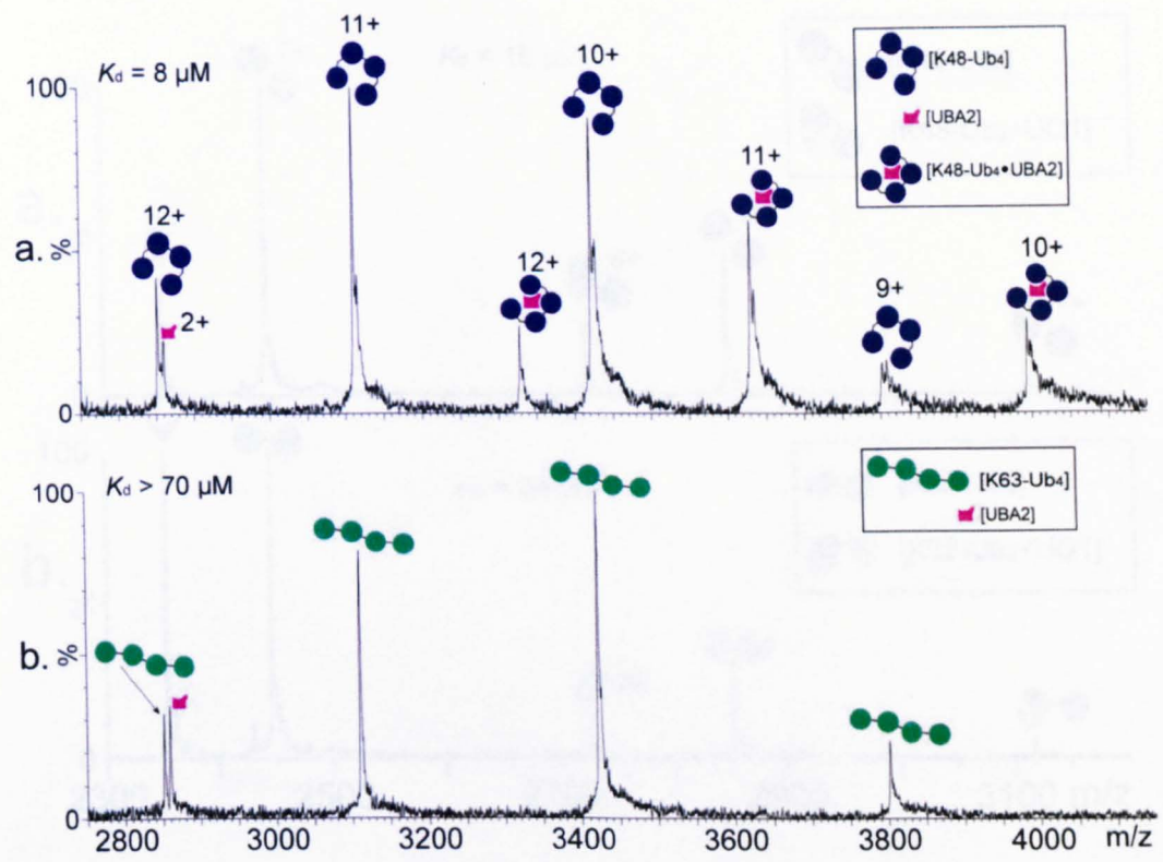
Figure 4.2.12 ESI mass spectra of UBA2 (4 μM) with: a) Lys48-linked Ub 4 (0.5 μM), b) Lys63-linked Ub 4 (0.5 μM), sprayed from 25 mM ammonium acetate solution under acetonitrile vapour
