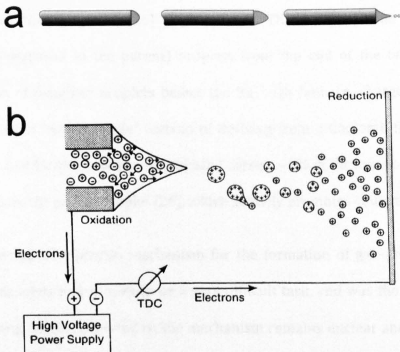
Figure 1.1.4 a) Effect of electrospay potential on the drop at the tip of the capillary as the voltage is increased from left to right. At the end the shape of the drop changes to a Taylor cone and small droplets are released. Adapted from reference [3]. b) Charge flow is maintained by an electrochemical oxidation reaction at the positive electrode in contact with the solution. Adapted from reference [25].
