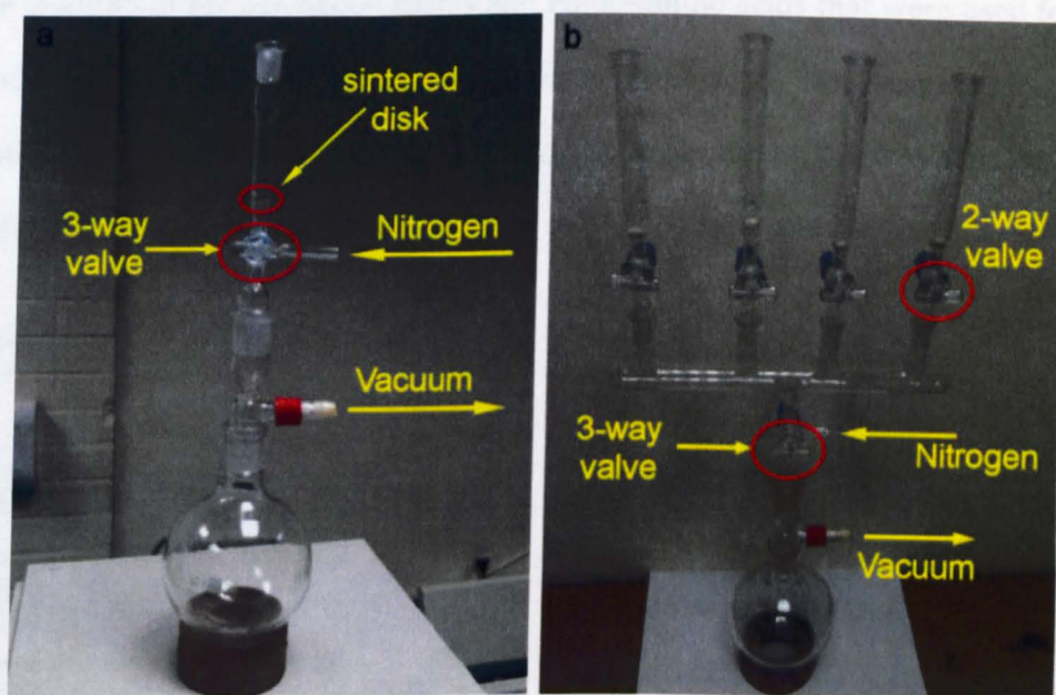
Figure 2.2.7 a) The apparatus that was used in manual peptide synthesis, b) the home-build 4-positions glass manifold.
