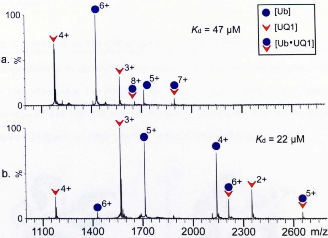
Figure 4.2.1 a) ESI mass spectra of Ub (0.5 \mu M ) and UQ1-UBA (4 \mu M ) complex, sprayed from 25mM ammonium acetate solution, b) ESI mass spectra of Ub (0.5 \mu M ) and UQ1-UBA (4 \mu M ) complex, sprayed from 25mM ammonium acetate solution in the presence of acetonitrile vapour.
