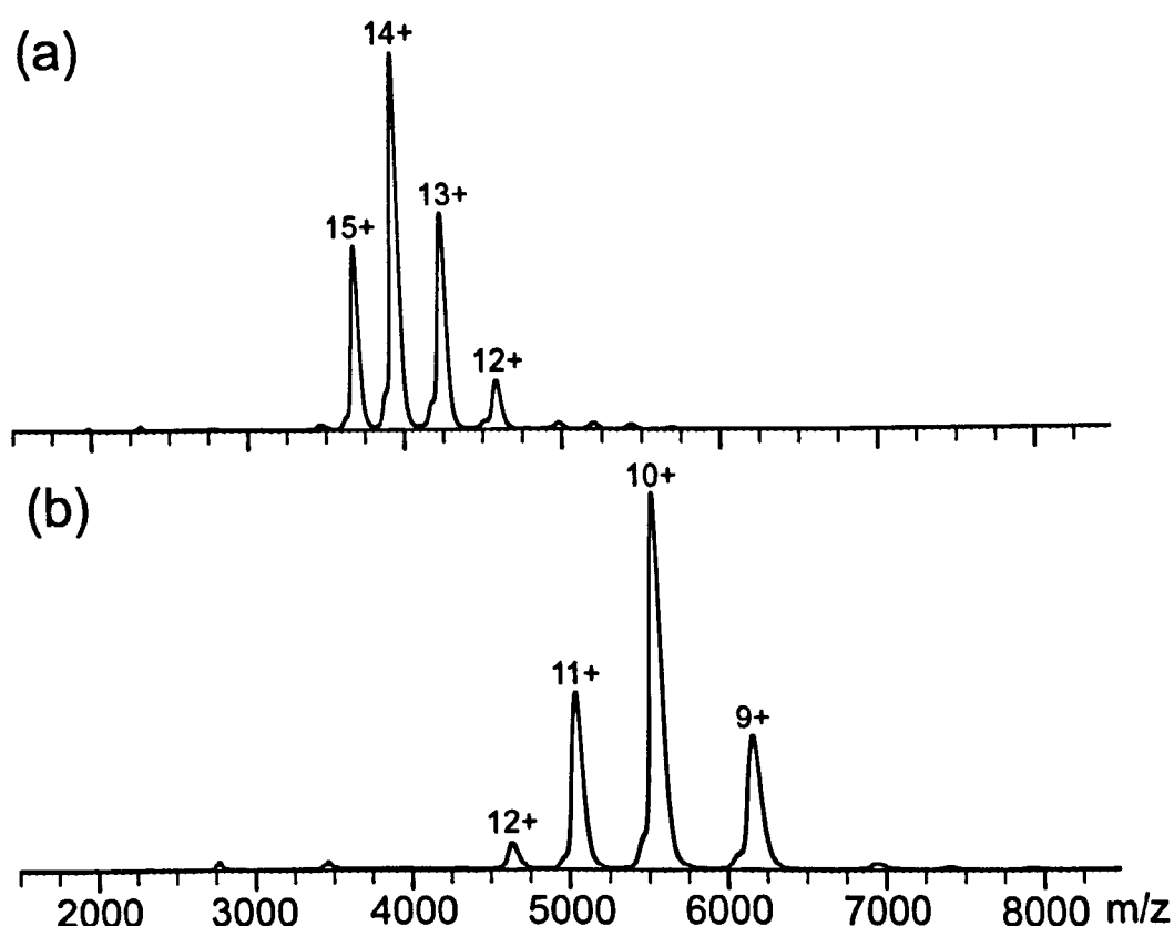
Figure 3.2.6 NanoESI spectra of hTTR (2.5 μM) sprayed from 25 mM ammonium acetate (a) under atmospheric conditions and (b) in the presence of acetonitrile vapour
