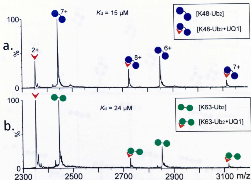
Figure 4.2.13 ESI mass spectra of 4 μM UQ1 with: a) Lys48-linked Ub 2 (0.5 μM) and b) Lys63-linked Ub 2 (0.5 μM), sprayed from 25 mM ammonium acetate solution under acetonitrile vapour.
