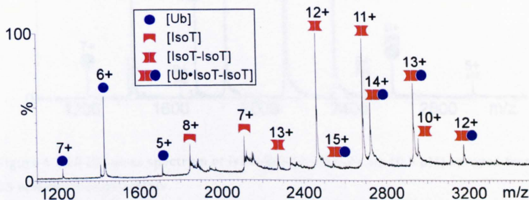
Figure 4.2.19 ESI mass spectrum of 0.5\text{ }\mu\text{M} ubiquitin (blue) and 2\text{ }\mu\text{M} IsoT-ZnF (red and orange) complex, sprayed from 25\text{ mM} ammonium acetate solution.
