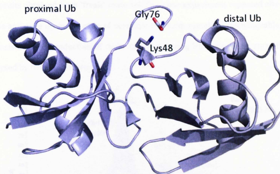
Figure 5.2.8 NMR structure of compact Lys48-Ub 2 (PDB ID: 2BGF) showing the close spatial proximity of Gly76 (proximal Ub) and Lys48 (distal Ub) residues.
