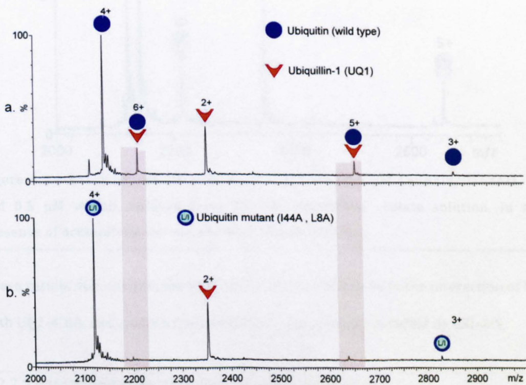
Figure 4.2.5 ESI mass spectrum of UQ1-UBA (2 μM) complex with a) wt-Ub (1 μM ) and b) Leu8Ala/Ile44Ala (1 μM) double mutant, sprayed from 25mM ammonium acetate solution under acetonitrile vapour.
