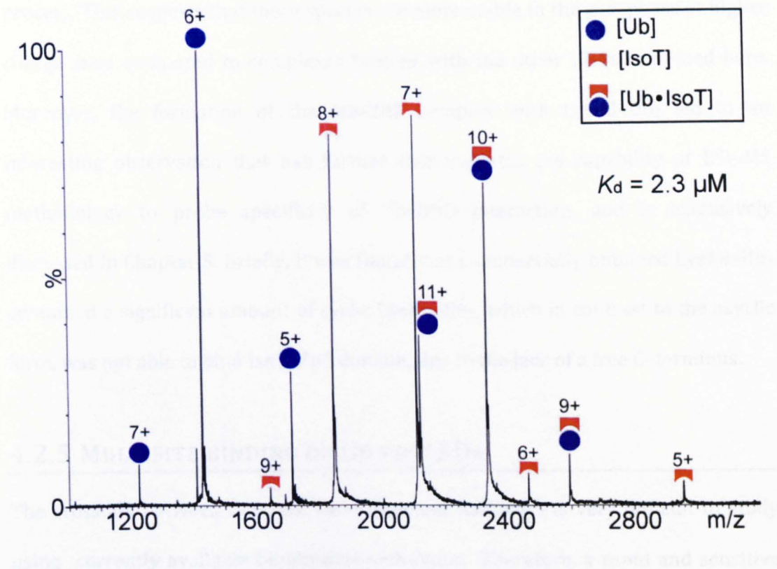
Figure 4.2.20 ESI mass spectrum of IsoT–ZnF (2 μM) and Ub (0.5 μM) sprayed from 25 mM ammonium acetate.
