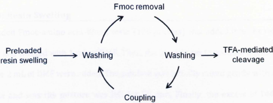
Figure 2.2.8 Diagram showing the Fmoc SPPS process
