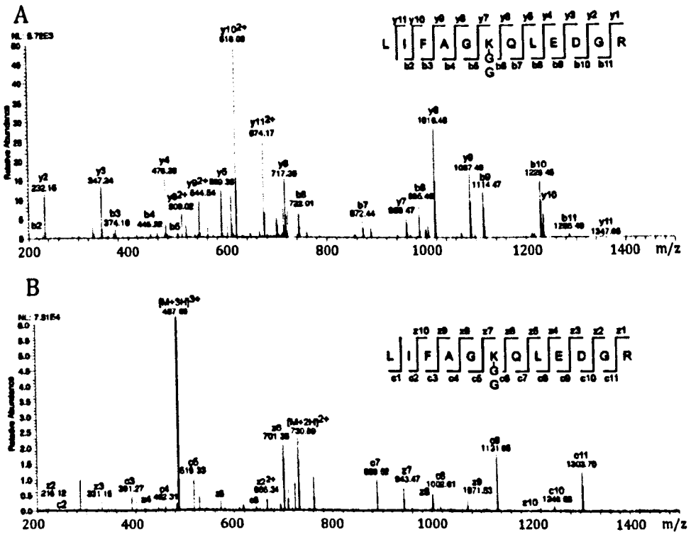
Figure 5.2.3 LC-ESI-MS/MS spectra of tryptic peptide 43–54 from Ub 2 purified from rat skeletal muscle resulting from (A) CID of the [M+2H] 2+ at m/z 731.0 and (B) ECD of the [M+3H] 3+ at m/z 487.7, clearly locating the linkage site to Lys48.
