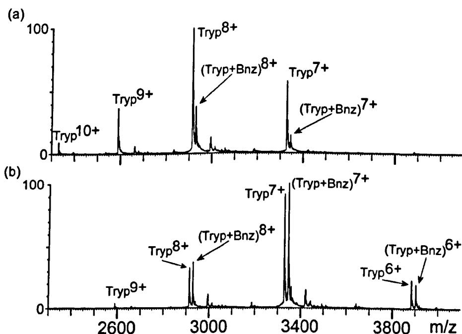
Figure 3.2.9 NanoESI spectra of 12 \mu M trypsin (Tryp) and 52 \mu M benzamidine (Bzn) sprayed from 10 mM ammonium acetate in an open laboratory atmosphere conditions (a) and under exposure to acetonitrile vapour (b).
