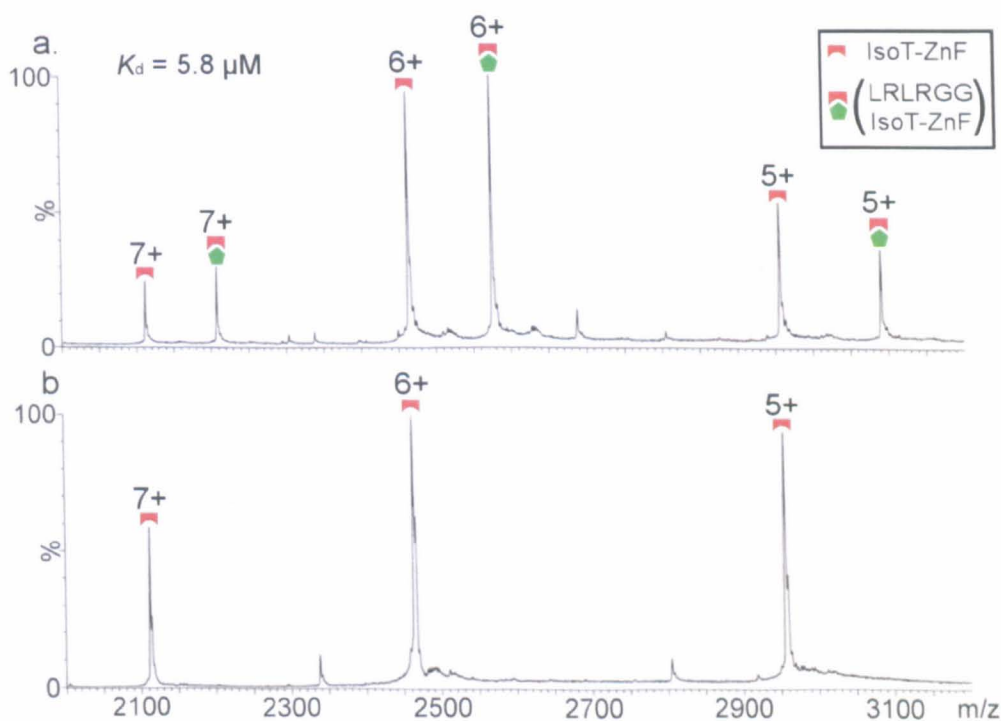
Figure 7.2.4 ESI–MS spectra of IsoT–ZnF ( 4 \mu\text{M} ) complex with a) LRLRGG peptide ( 7.5 \mu\text{M} ) and b) LRLRGV peptide ( 7.5 \mu\text{M} ), sprayed from 25 mM ammonium acetate solution in the presence of acetonitrile vapour
