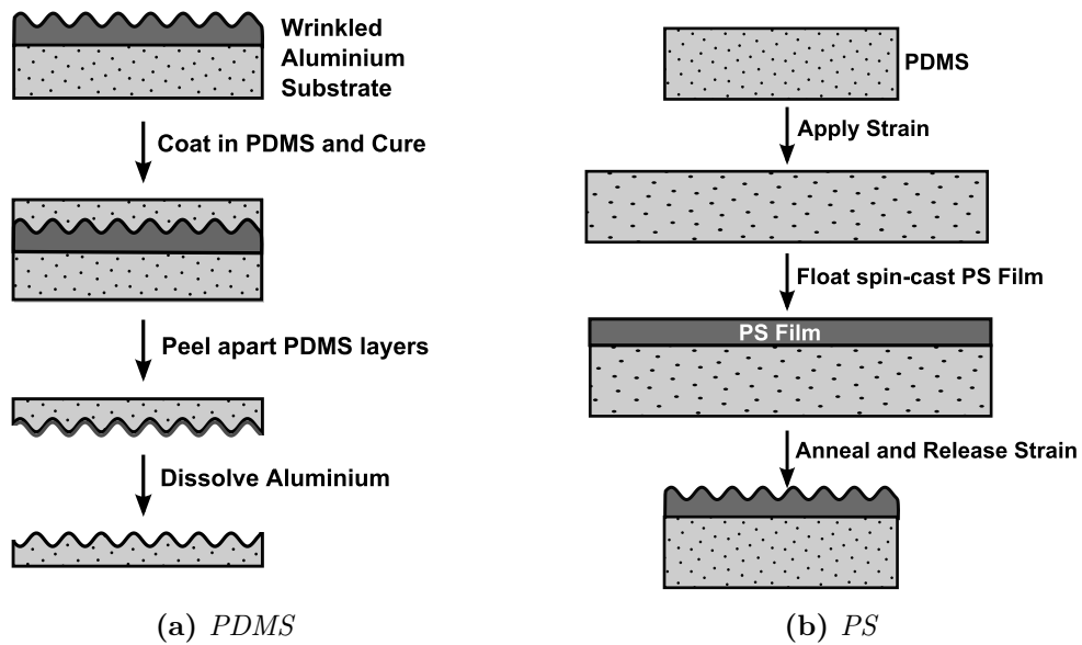
Figure 3.10: The processes used to make wrinkled PDMS (Polydimethylsiloxane) and PS (Polystyrene) substrates. (a) Wrinkled aluminium substrates (Al on PDMS) were used as a mould for another layer of PDMS. Once applied, it was cured at 150^{\circ}\text{C} before separating the two PDMS layers. Residue aluminium was dissolved using a sodium hydroxide solution. (b) Wrinkled PS substrates were made by floating a PS film onto a PDMS substrate that was under strain. After annealing, the strain was removed causing the PS to wrinkle.
