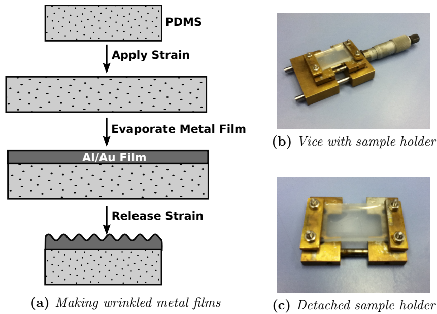
Figure 3.7: (a) shows the method used to wrinkle metal films. PDMS was moulded into sheets with a thickness of \sim 2\text{mm} . A home built device, pictured in (b), was used to apply a strain of 50 % to the PDMS. The top part of this device could be locked off and detached as shown in (c) and was then placed in a thermal evaporator where \sim 100\text{nm} of aluminium or gold was deposited. When the strain was released, wrinkles with height and periodicity \sim \text{microns} were formed.
