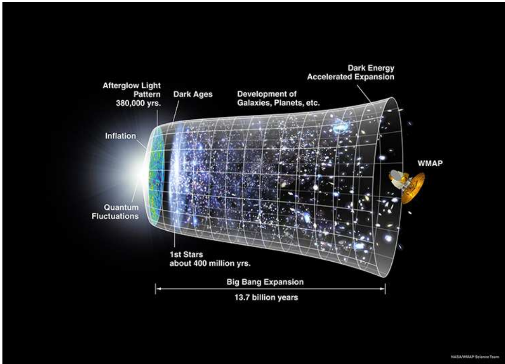
Figure 1.2: Schematic representation of the growth of structure in the Universe, from quantum fluctuations following the big bang (far left), being magnified through Inflation (Guth 1981) resulting in the CMB emitted from the last scattering surface; the first stars which reionised the Universe, and the evolution of galaxies stretching through to the present day. Image credit: NASA/WMAP Science Team.
