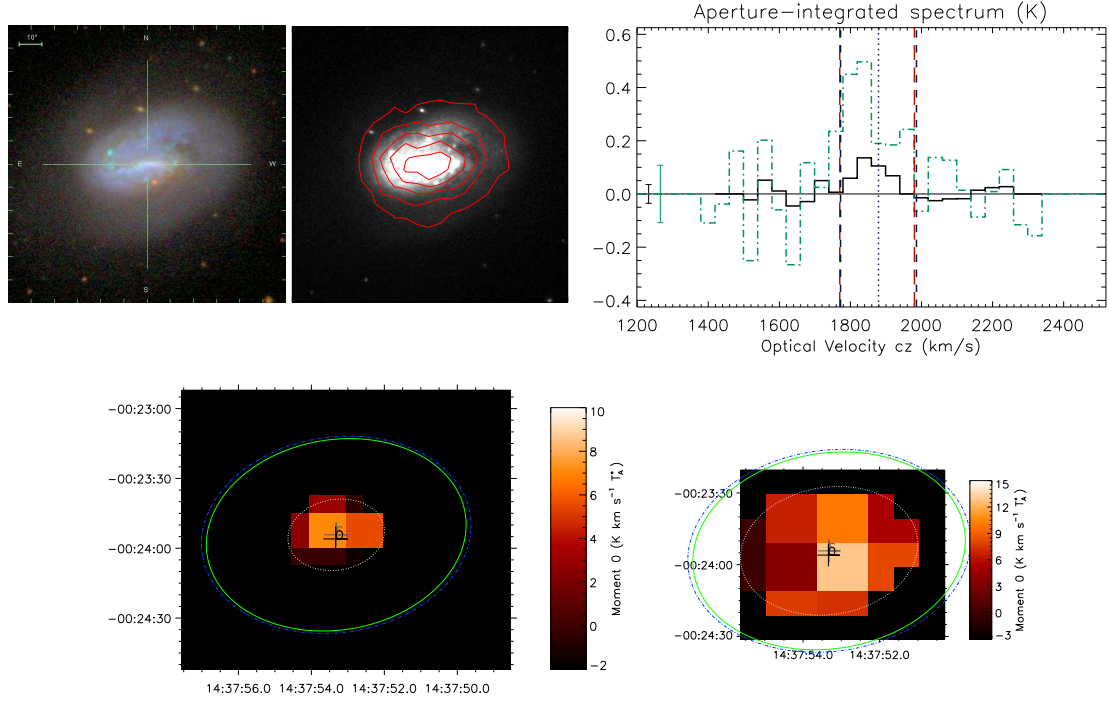
Figure D.8: NGC 5691. Top: SDSS image, 250 \mu\text{m} contours, and aperture-integrated spectra in HARP (black) and RxA (green). Blue lines = H I line width from HIPASS; red = CO width integrated over for moment maps. Below: rebinned moment maps in HARP (left) and RxA (right). ‘O’ marks the optical centroid and ‘S’ the SPIRE centroid; the green line is the SPIRE Kron ellipse and blue is the B -band D_{25} isophote. The white line marks the aperture within which the total flux was integrated.
