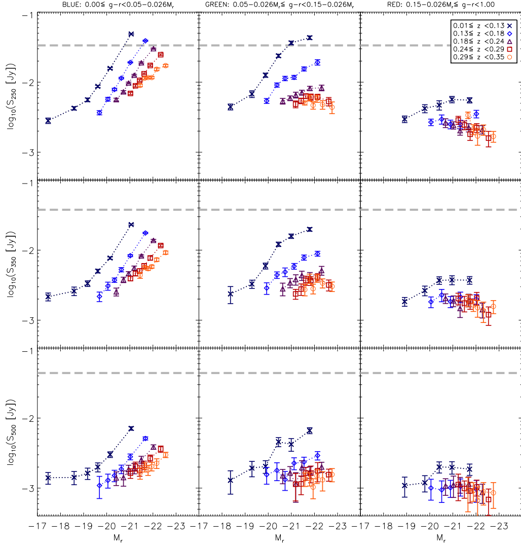
Figure 3.7: Stacked SPIRE fluxes (not k -corrected) as a function of g - r colour, redshift and absolute magnitude M_r . Top: 250\,\mu\text{m} , middle: 350\,\mu\text{m} , bottom: 500\,\mu\text{m} . Galaxies are binned by optical colour from blue to red (shown in panels from left to right) and by redshift (shown by plot symbols) and stacked fluxes in each bin are plotted against M_r . Error bars are the statistical 1\sigma errors in the bins as described in Section 3.3.3, and also include errors due to background subtraction. The horizontal dashed lines at 33.5, 39.5 and 44.0 mJy in 250, 350 and 500\,\mu\text{m} , represent the 5\sigma point-source detection limits as measured in the PSF-convolved Phase 1 maps.
