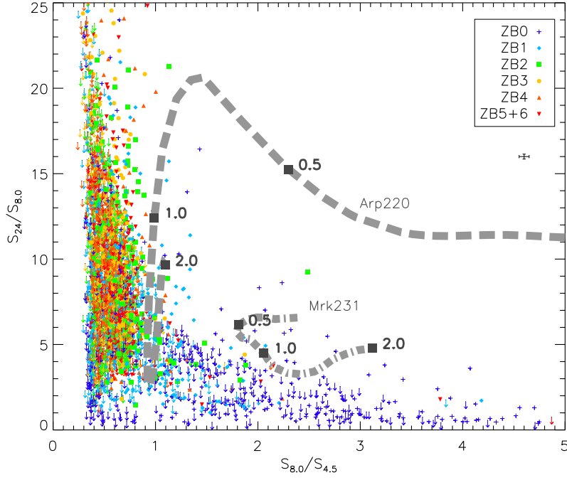
Figure 2.9: Observed-frame S_{8.0 \mu\text{m}}/S_{4.5 \mu\text{m}} - S_{24 \mu\text{m}}/S_{8.0 \mu\text{m}} colour-colour plot of all objects in the sample, coloured by redshift bin (for ranges see Table 2.1). The 24 \mu\text{m} aperture fluxes are used where they are \geq 5\sigma (roughly 30% of the positions). For the positions without a 5\sigma detection at 24 \mu\text{m} , I use the 5\sigma upper limit (indicated by arrows). IRAC fluxes are from the SIMPLE catalogue. The representative error bar in the top right shows the median 1\sigma errors. Some scatter in the vertical axis is introduced by confusion at 24 \mu\text{m} , but positions in the horizontal axis are reliable as signal-to-noise is good in both 4.5 \mu\text{m} and 8.0 \mu\text{m} and confusion noise is much lower. Tracks of starburst (Arp220) and AGN (Mrk231) SEDs are overlaid in grey, showing the locus of each on the diagram as a function of redshift between 0 and 2. The horizontal scatter in the data in bin ZB0 is attributed to the strong PAH emission feature at 7.7 \mu\text{m} contributing to the 8 \mu\text{m} band at low redshifts.
