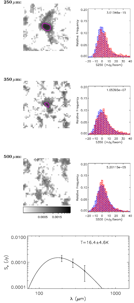
Figure C.4: A stack of galaxies with red g - r colours, median M_r = -22.5 , median z = 0.27 . This stack has among the faintest sub-mm fluxes, and contains 1002 objects. Plots are as in Figure C.1 except that the postage stamps are plotted on a logarithmic greyscale between 0.0001 - 0.004 \text{ Jy beam}^{-1} .
