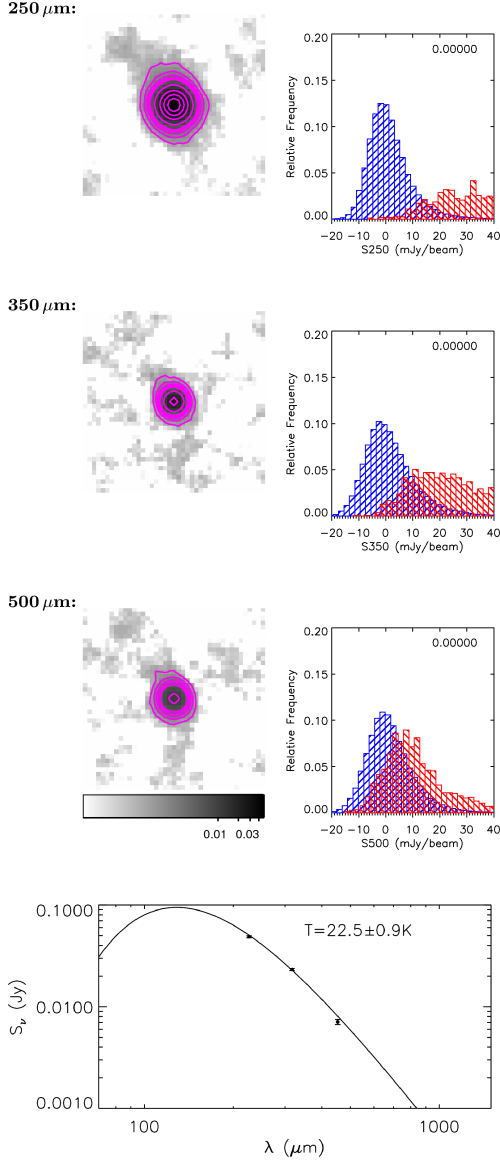
Figure C.1: A stack of galaxies with blue g - r colours, median M_r = -21.1 , median z = 0.11 . This stack is one of the brightest in sub-mm flux, and contains 1567 objects. Stacked, PSF-filtered postage stamps are shown with a logarithmic greyscale between 0.0001 - 0.05 \text{ Jy beam}^{-1} and signal-to-noise contours at 5, 10, 15, 20, 25, 50, 100, 150, 200, 250. Histograms of the measured fluxes in the stack (red) and in a random background stack (blue) are shown with the KS probability that they were drawn from the same distribution. Also plotted is the rest-frame SED fit with the temperature indicated, assuming \beta = 2 . More details are given in the text above.
