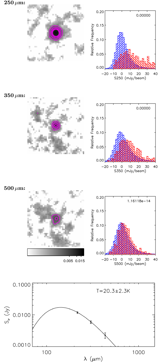
Figure C.2: A stack of galaxies with green g - r colours, median M_r = -21.1 , median z = 0.15 . This stack has moderate sub-mm flux, and contains 570 objects. Plots are as in Figure C.1 except that the postage stamps are plotted on a logarithmic greyscale between 0.0001 - 0.02 \text{ Jy beam}^{-1} .
