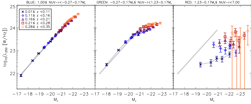
Figure 3.10: Stacked 250 \mu\text{m} luminosities as a function of NUV - r colour, redshift and M_r . Error bars are the statistical 1\sigma errors in the bins as described in Section 3.3.3. Data and errors in the red bin incorporate the correction for lensing. The thick grey line is the same from left to right, and is the linear least-squares fit to the results for the lowest-redshift blue galaxies.
