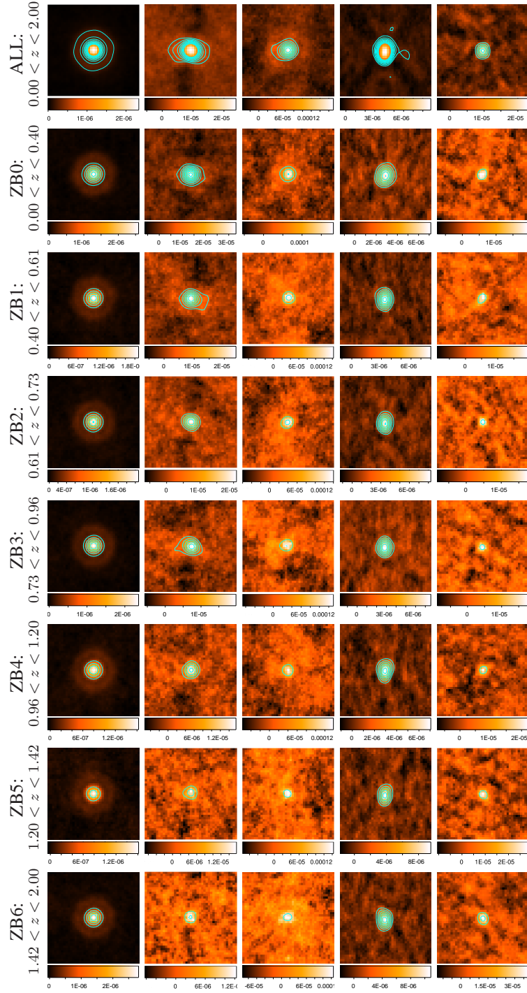
Figure 2.3: Postage-stamp images of the stacked targets in (from left to right) 24 \mu\text{m} , 70 \mu\text{m} , 160 \mu\text{m} , 1.4 GHz, 610 MHz. The top row is the stacked full sample; other rows are the stacks of redshift bins ZB0–ZB6 (from top to bottom) as described in the text. Images are coloured by flux in \text{Jy pixel}^{-1} units (MIPS) and \text{Jy beam}^{-1} units (radio), and colour scales are included below each. Contours of [3, 5, 7, ... 19] times the pixel noise are overlaid. Each tile is a square 41 pixels on a side, which corresponds to 49.2, 164, 328, 20.5 and 61.5 arcsec for the five bands respectively.
