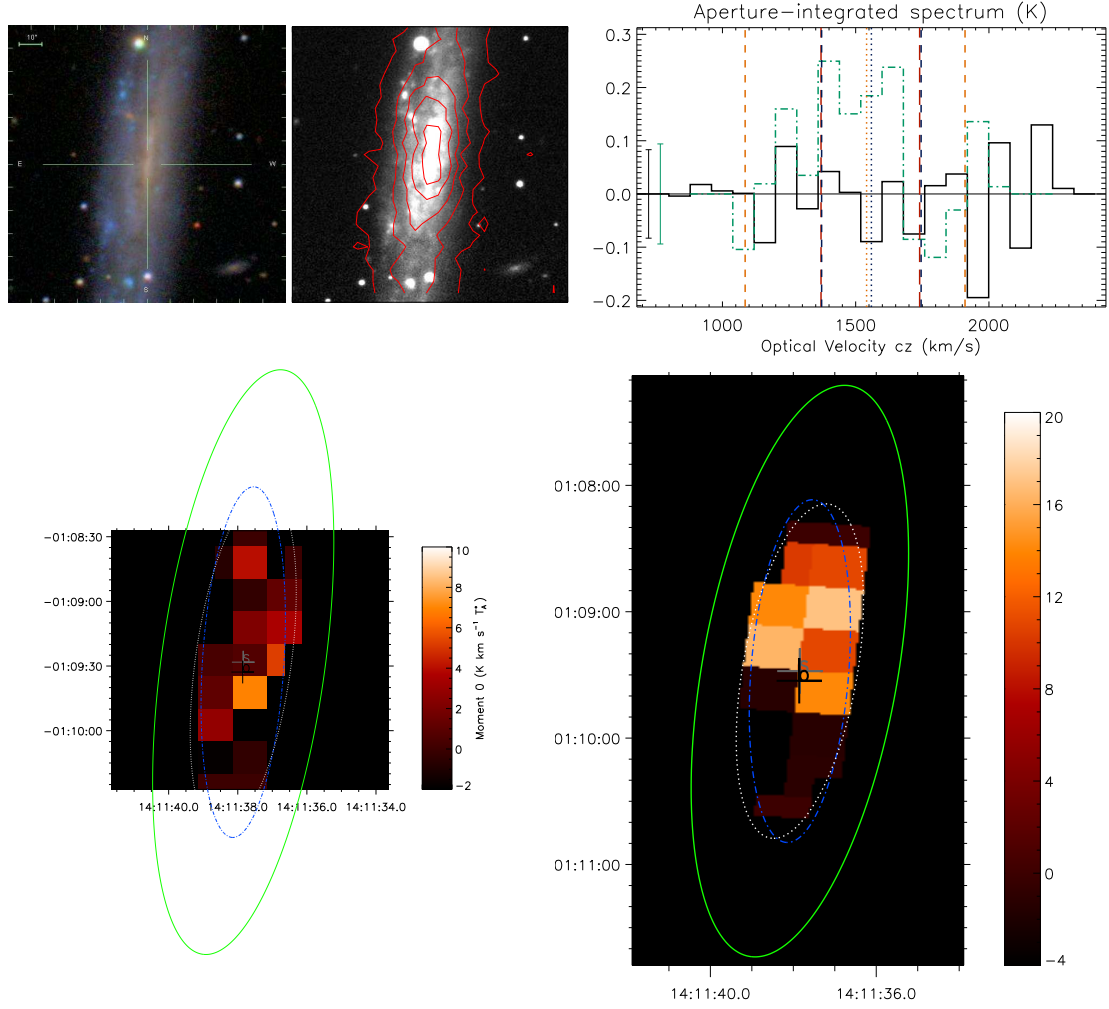
Figure D.6: NGC 5496. Top: SDSS image, 250 \mu\text{m} contours, and aperture-integrated spectra in HARP (black) and RxA (green). Blue lines = H I line width from HIPASS; orange = CO line width from literature; red = CO width integrated over for moment maps. Below: rebinned moment maps in HARP (left) and RxA (right). ‘O’ marks the optical centroid and ‘S’ the SPIRE centroid; the green line is the SPIRE Kron ellipse and blue is the B -band D_{25} isophote. The white line marks the aperture within which the total flux was integrated.
