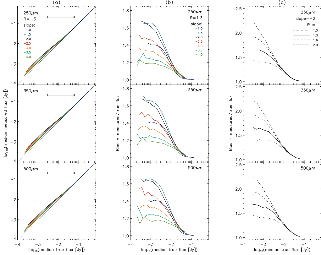
Figure B.1: Results of a set of stacking simulations: (a) Comparing median measured flux and median true flux, for distributions in various flux ranges. The range in each simulation is given by R = \log_{10}(S_{\text{max}}/S_{\text{min}}) = 1.3 (the length of the grey horizontal bar), and the simulations were run 16 times with different S_{\text{min}}, S_{\text{max}} values to produce distributions with a range of median (true) fluxes. Each coloured line in the Figure connects 16 data points, one point from each simulation, showing how the median measured flux (after adding noise) varies as the median true flux is varied. Noise is drawn from a Gaussian distribution centred on zero, with \sigma = 6.7, 7.9, 8.8 \text{ mJy beam}^{-1} at 250, 350, 500 \mu\text{m} respectively. Different coloured lines correspond to sets of simulations with different slopes of dN/dS between -1 and -4 . (b) Bias factor (ratio of median measured to median true flux) as a function of median true flux, for the same set of simulations, showing how the bias depends on the slope of dN/dS for R = 1.3 . Note that bias does not vary monotonically with slope for fixed R , but is greatest for a slope of -1.5 in this case. (c) Bias factor as a function of median true flux, showing the effect of increasing the range of true fluxes. Different lines correspond to sets of simulations with different values of R between 1 and 2; in each of these the slope of dN/dS is -2 .
