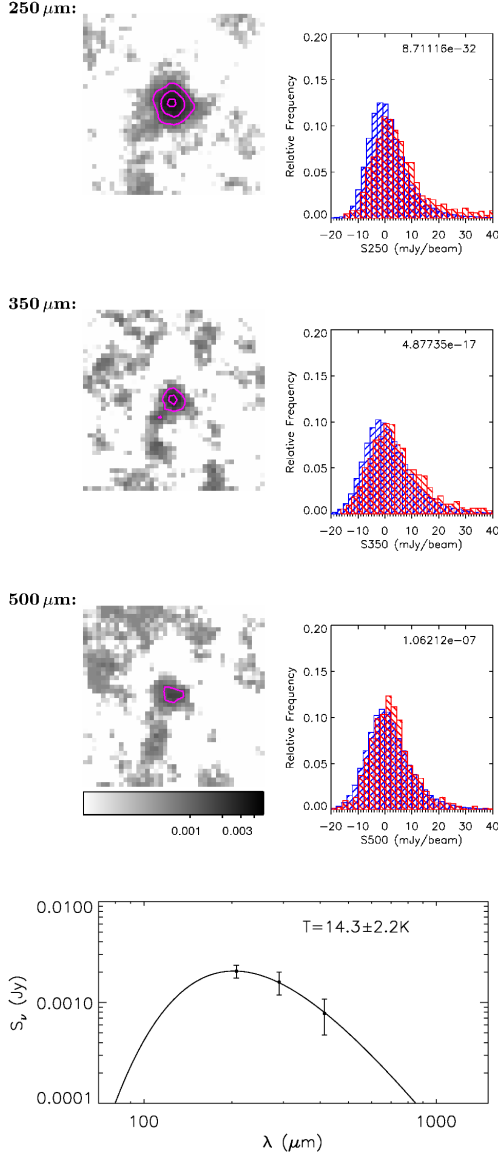
Figure C.3: A stack of galaxies with red g - r colours, median M_r = -21.7 , median z = 0.21 . This stack has among the faintest sub-mm fluxes, and contains 1111 objects. Plots are as in Figure C.1 except that the postage stamps are plotted on a logarithmic greyscale between 0.0001 - 0.005 \text{ Jy beam}^{-1} .
