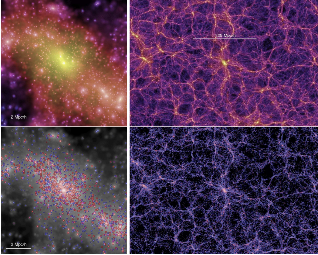
Figure 1.4: Snapshots from the Millennium Simulation (Springel et al. 2005) at z = 0 . The upper two images show the dark matter distribution on the scale of an individual galaxy cluster (left) and a larger volume encompassing the large-scale structure of filaments and voids (right). Intensity represents surface density and colour represents local velocity dispersion. The lower two images show the galaxy light distribution in the same volumes from the SAM of Croton et al. (2006). Intensity and colour represent that of the optical light, with redder galaxies being more concentrated in the denser regions. Credit: Volker Springel and the Max-Planck-Institute for Astrophysics.
