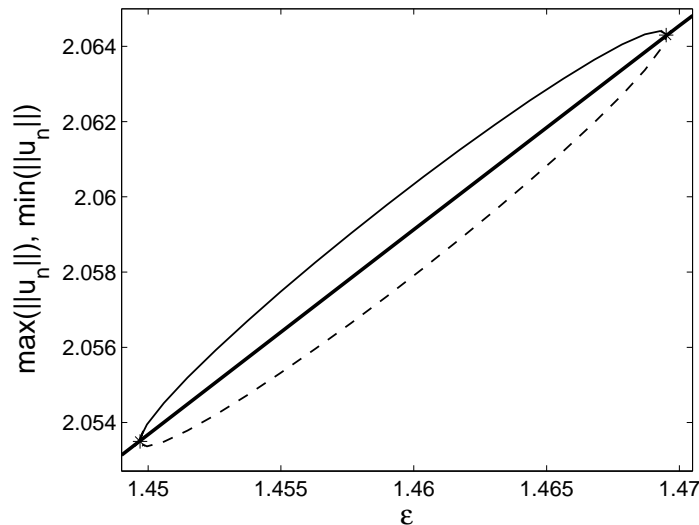
Figure 3.19: As Fig. 3.18(a) but for \alpha = 0.492642 . Two Hopf points (stars) in the neighbourhood of the degenerate point (the white-filled circle in Fig. 3.4) are shown to be connected by a branch of limit cycles.
