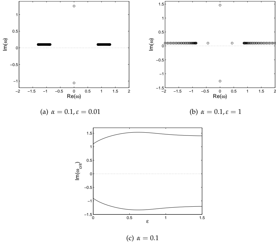
Figure 3.6: The top panels show the eigenvalue structure of onsite bright solitons type II for \alpha = 0.1 and two values of \varepsilon as indicated in the caption. The bottom panel depicts the imaginary part of the critical eigenvalues as a function of \varepsilon .
