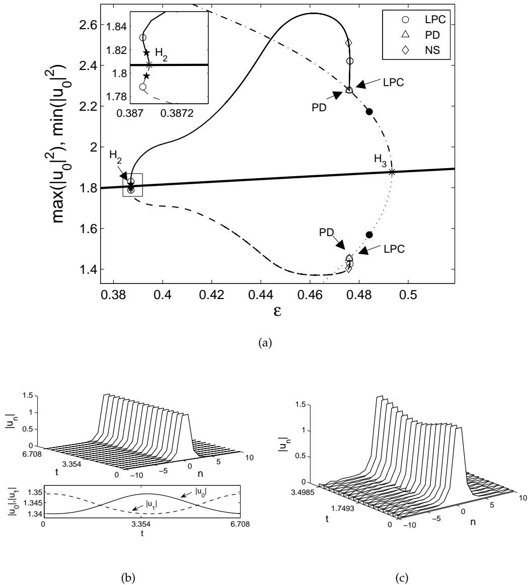
Figure 3.21: (a) As Fig. 3.20(a) but for H_2 and H_3 , where the inset gives the zoom-in for the corresponding region showing that H_2 and H_3 are supercritical and subcritical, respectively. The bold solid line is the same as that shown in Fig. 3.17, i.e., representing the value of |u_0|^2 for the stationary intersite soliton. The solid (dashed) and dash-dotted (dotted) lines shows the maximum (minimum) value of |u_0|^2 for the periodic soliton which bifurcates from, respectively, H_2 and H_3 . (b,c) The profile of periodic solitons over one period T \approx 6.708 and T \approx 3.4985 which corresponds, respectively, to the star and the black-filled circle in panel (a).
