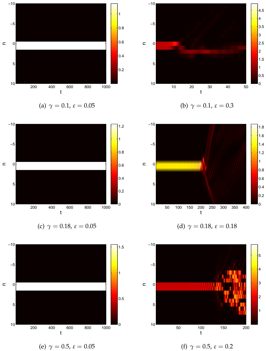
Figure 2.7: The numerical evolution of the time-dependent Eq. (2.1.1) for an intersite bright soliton (the contour plot shows the square modulus |\phi_n|^2 ). The parameter values are indicated in the caption of each panel which are the same as those in Fig. 2.5. The left and the right panels exhibit the dynamics of stable and unstable solitons, respectively.
