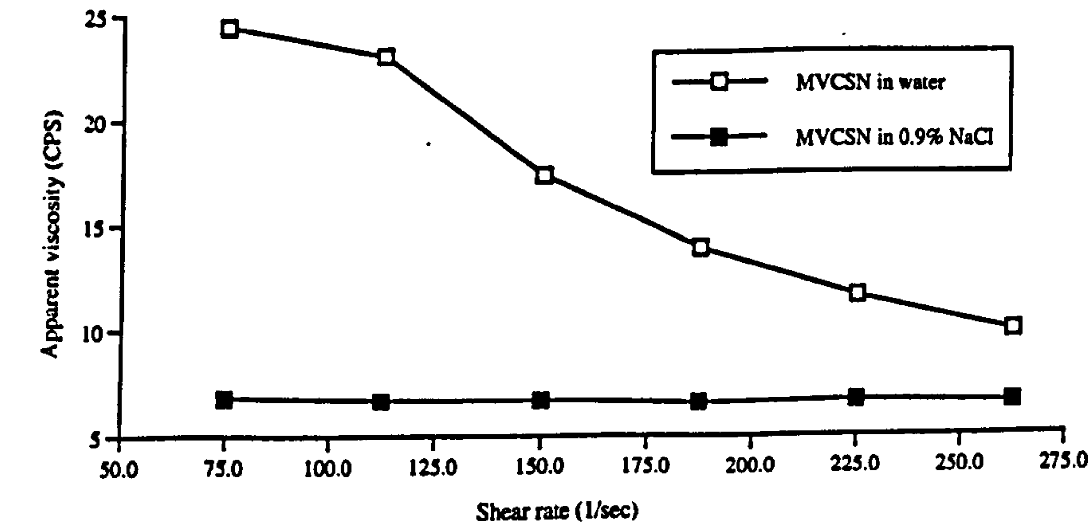
Figure 10.10 Effect of shear rate on the apparent viscosity of MVCSN solutions
