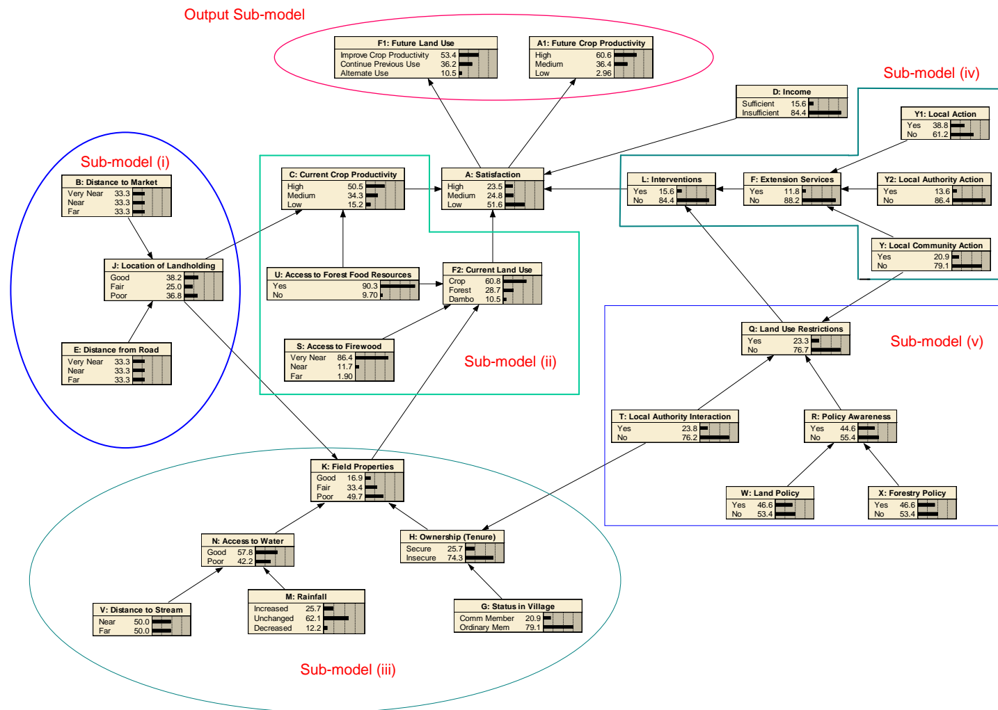
Figure 8.10: BN model showing sub-model divisions
