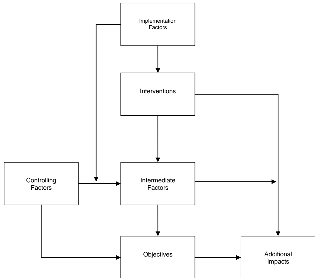
Figure 7.1: The general structure of a BN model (Cain, 2001)
