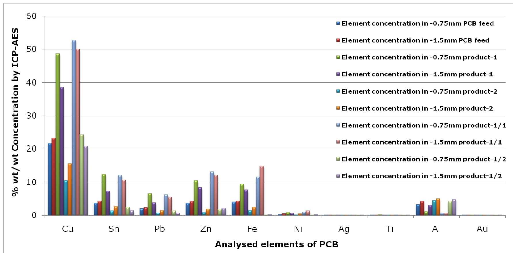
Figure C.1: Concentration of major WEEE-PCB elements before and after vertical vibration separation.
