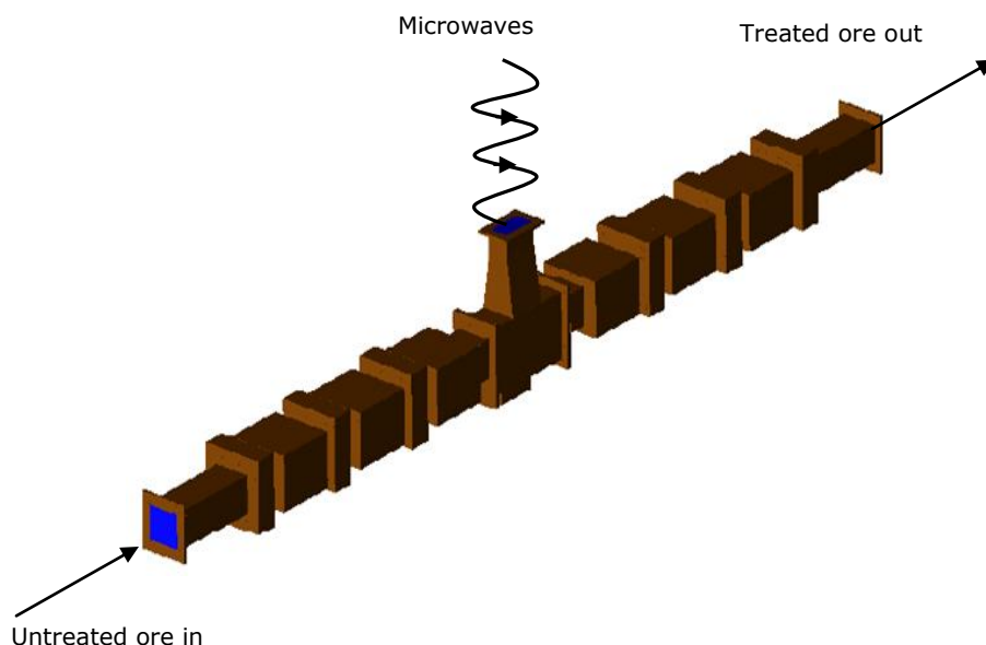
Figure 5.6 Configuration of applicator design for continuous microwave treatment of ores
