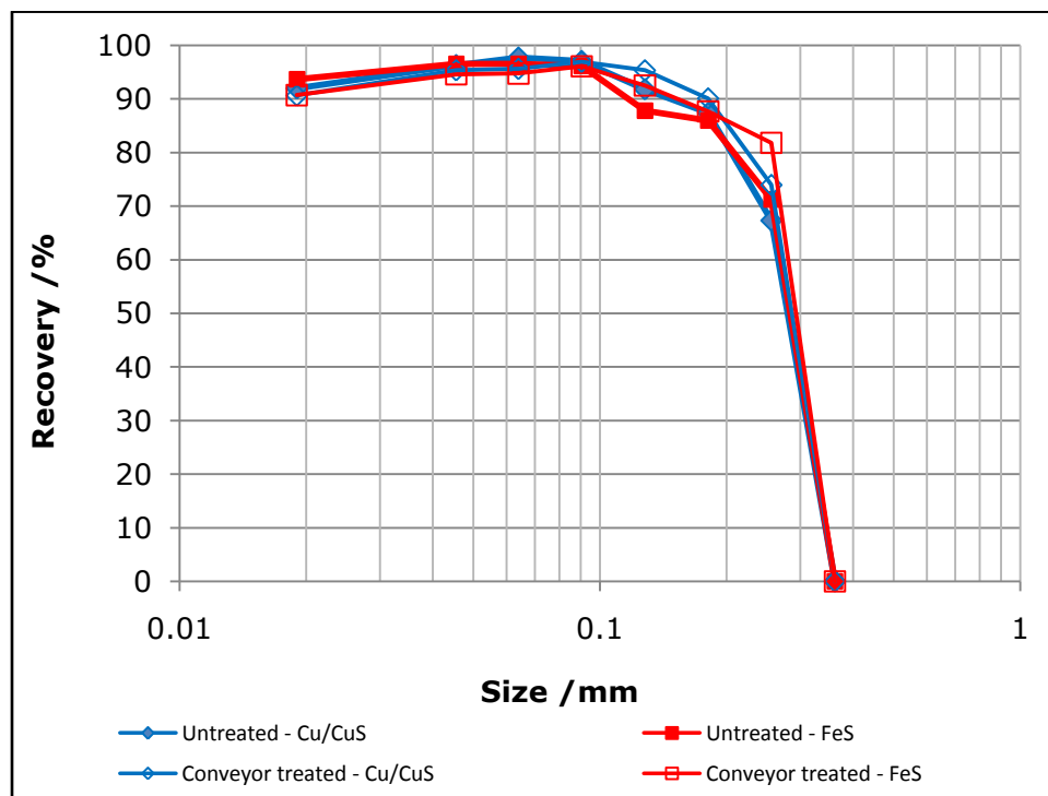
Figure 5.27 Sulphides recovery by size from Copper II fine grind
