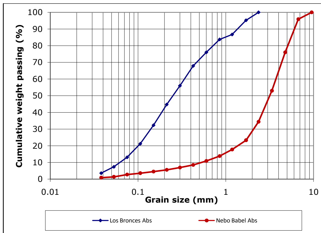
Figure 4.5 Size distribution of microwave absorbent mineral grains in Nebo Babel and Los Bronces ores
