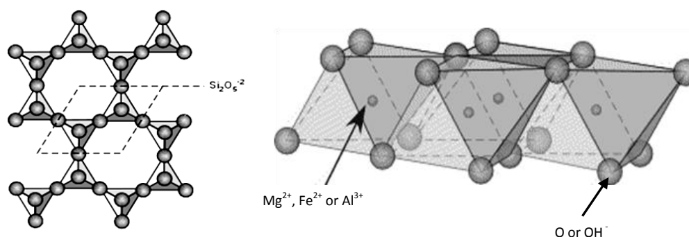
Figure 4.7 The basic tetrahedral building block for phyllosilicate minerals (left). Illustration of phyllosilicate sheet coordination (right) (Nelson, 2008)
