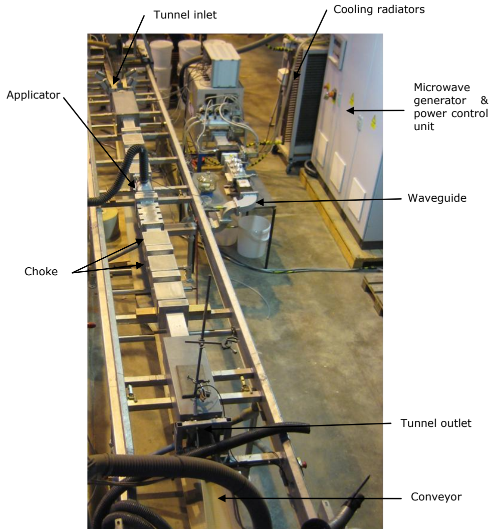
Figure 5.7 Microwave system used for continuous process ore treatment
