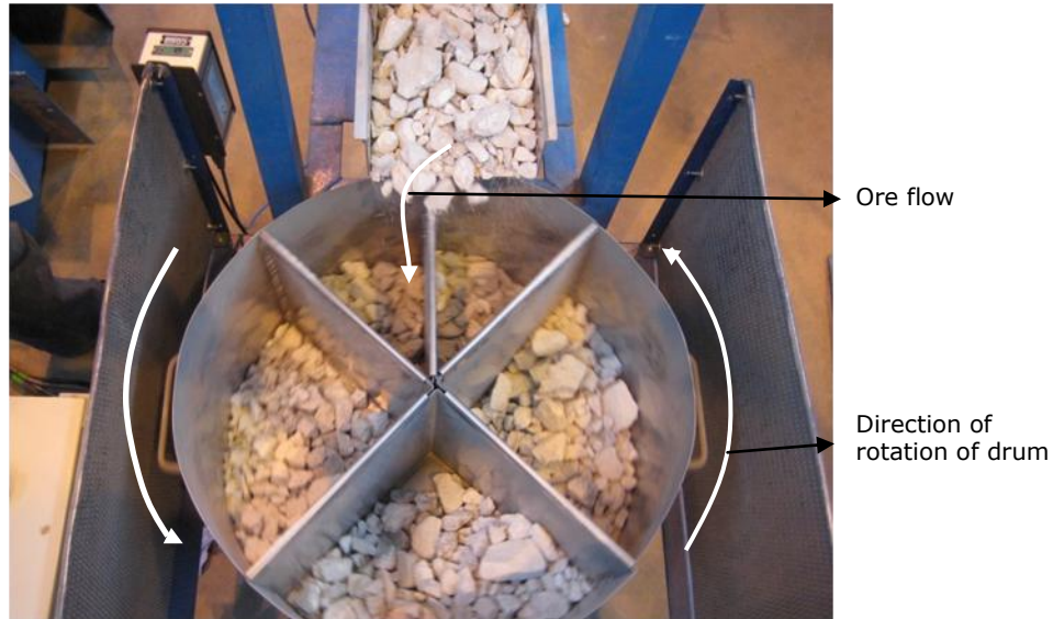
Figure 4.2 Rotary sample divider (RSD) used for ore sampling
