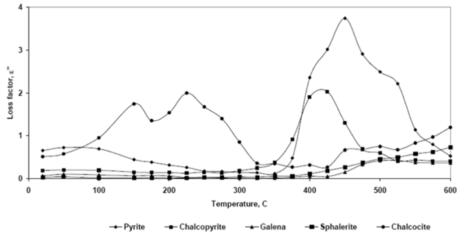
Figure 2.7 Variation of loss factor with temperature for selected minerals (Cumbane, 2002)
