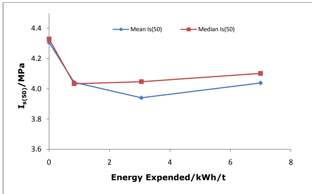
Figure 4.36 Variation of Strength with energy input- Los Bronces Cu ore
