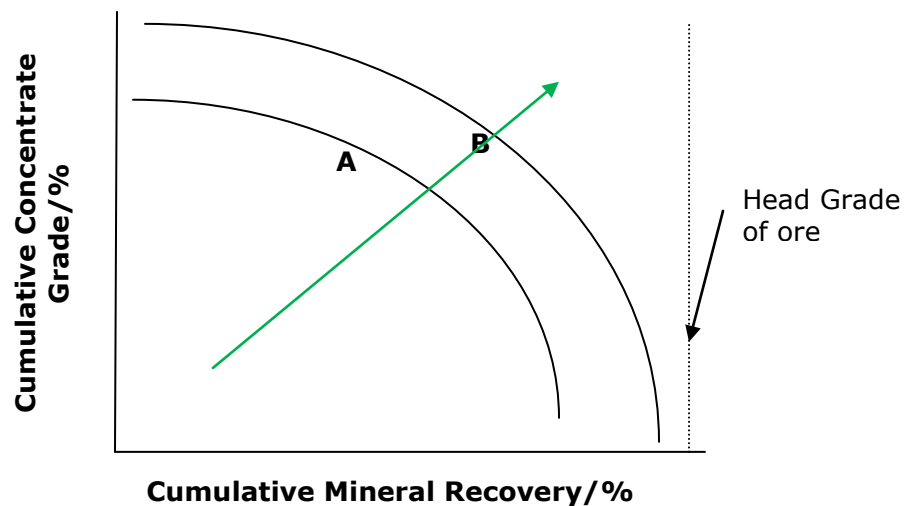
Figure 5.17 A Typical Grade-Recovery curve
