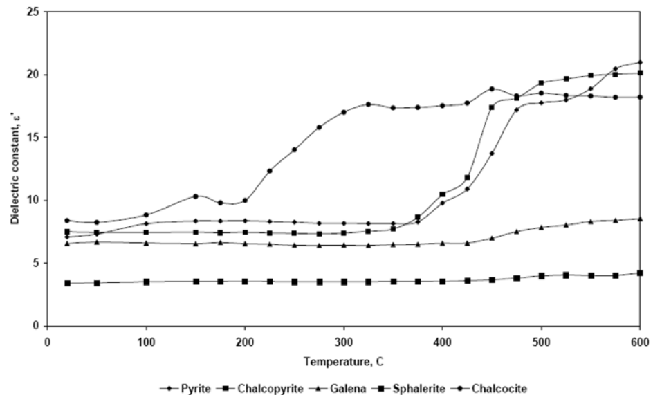
Figure 2.6 Variation of dielectric constant with temperature for selected minerals (Cumbane, 2002)
