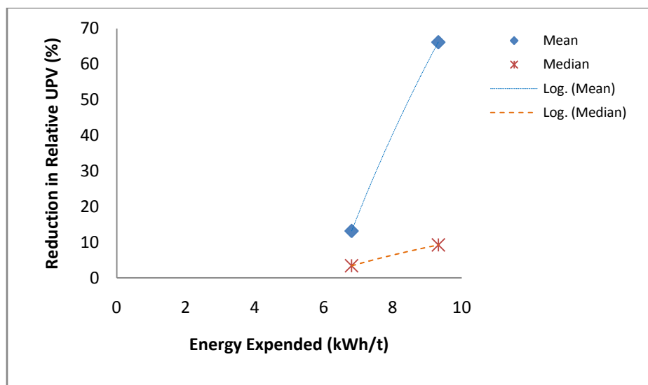
Figure 4.52 Variation of UPV with energy expended in treating Kimberlite I ore samples
