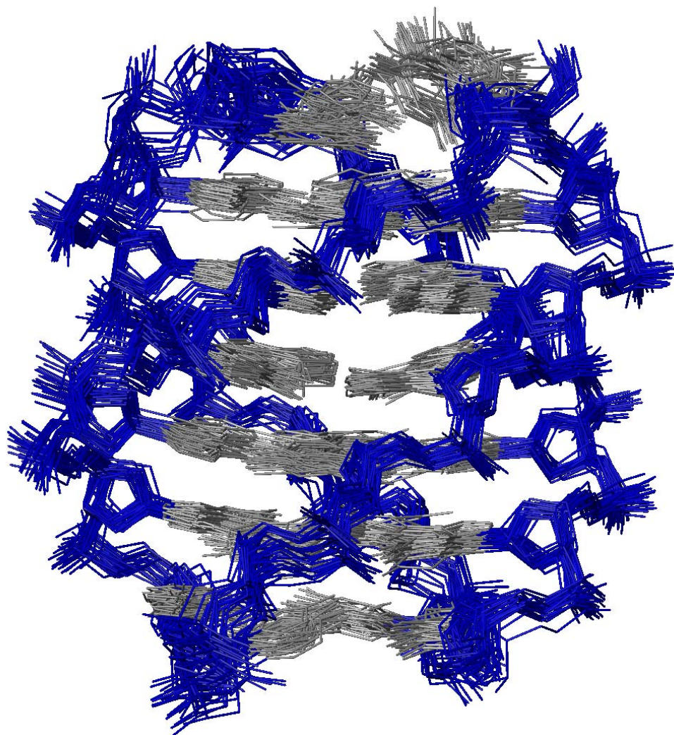
Fig.4.32: 25 randomly chosen structures from the last 500 ps of a 2ns rMD simulation of d(TGGAGGC) 4
