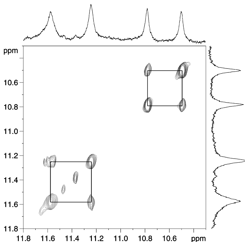
Fig.4.17: ^1\text{H} NMR and NOESY spectra (600 MHz) of \text{d}(\text{TGGAGGC})_4 at 279K (90% \text{H}_2\text{O} , 10% \text{D}_2\text{O} ), expanded to highlight the imino region (10.3-11.8 ppm). Imino resonances are evident for each of the four G-tetrads. NOE crosspeaks are clearly evident between adjacent tetrads G2 (11.6 ppm) & G3 (11.2 ppm), and G4 (10.7 ppm) & G5 (10.5 ppm).
