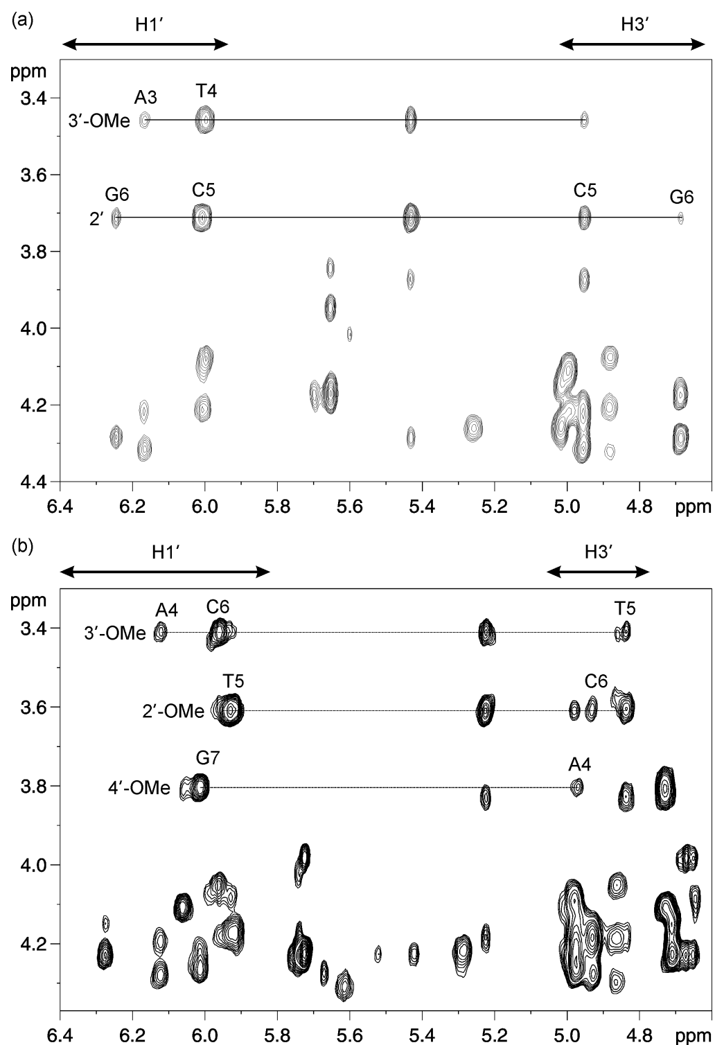
Fig.2.17: Portion of the NOESY spectra (298 K, 300 ms) of (a) d(CGATCG) 2 and (b) d(TCGATCGA) 2 , highlighting interactions between nogalose methoxy protons and H1' protons on the floor of the minor groove in the conserved central portion of each oligomer.
