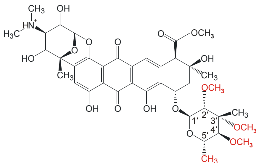
Fig.3.36: Nogalamycin, highlighted to emphasise Nog-2'-OCH 3 , Nog-3'-OCH 3 , Nog-4'-OCH 3 & Nog-5'-CH 3 protons on the nogalose sugar.
