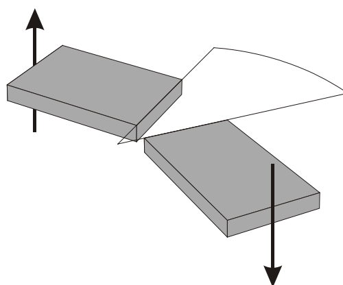
Fig.3.49: Schematic representation of base pair opening ( \sigma ).
