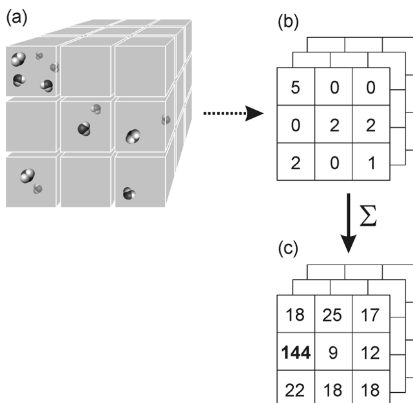
Fig.5.1: Schematic representation of the method used to determine water occupancy from rMD simulation: The periodic box is divided into 1 \text{ \AA}^3 cubes (a). The number of water molecules in each cube is summed for each snapshot of the simulation (b), and the values from each snapshot are subsequently added to give a figure for total water occupancy (c). Using this method, higher occupancy sites can readily be identified.
