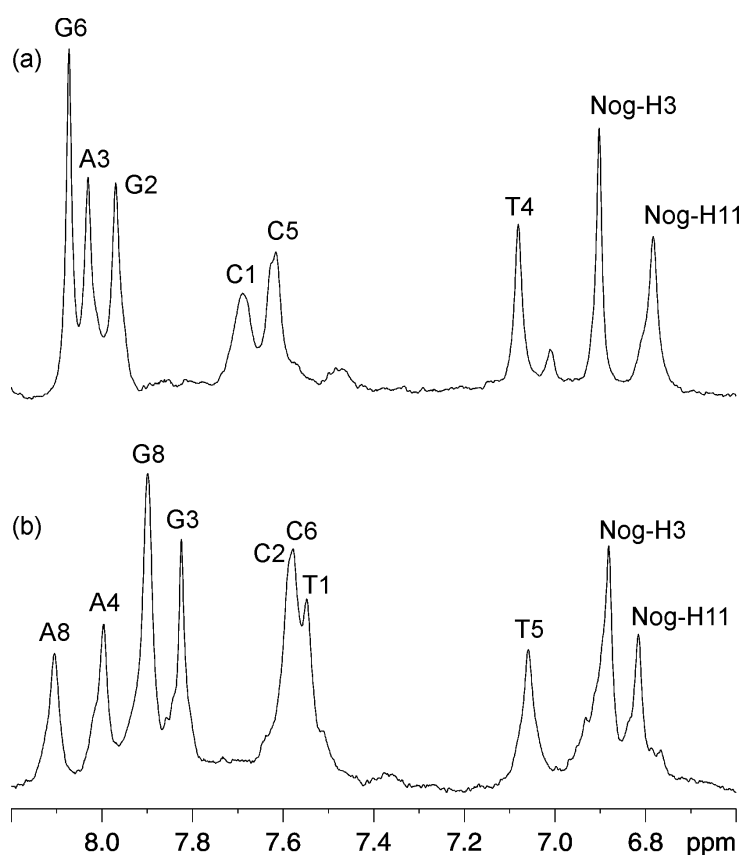
Fig.2.15: Aromatic region (ppm) of the 1D ^1\text{H} spectra of (a) nogalamycin-d(CGATCG) 2 and (b) nogalamycin-d(TCGATCGA) 2 .
