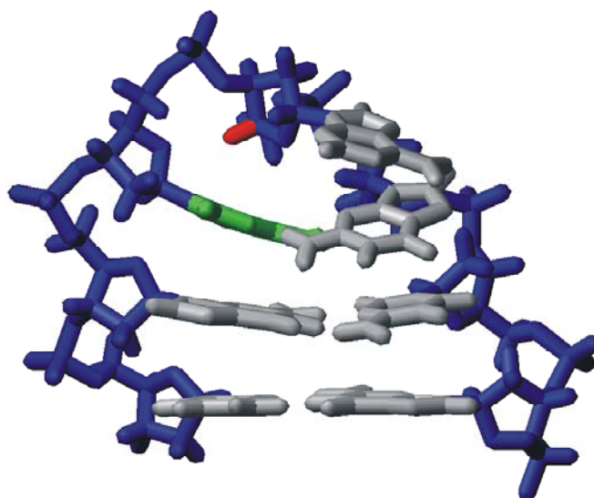
Fig.3.16: Stick model of the d(GCGAAGC) hairpin loop, viewed from the major groove and illustrating the proximity of the A6H4' (red) to the A5 ring system (green). Structure solved by Hirao et al. (98).
