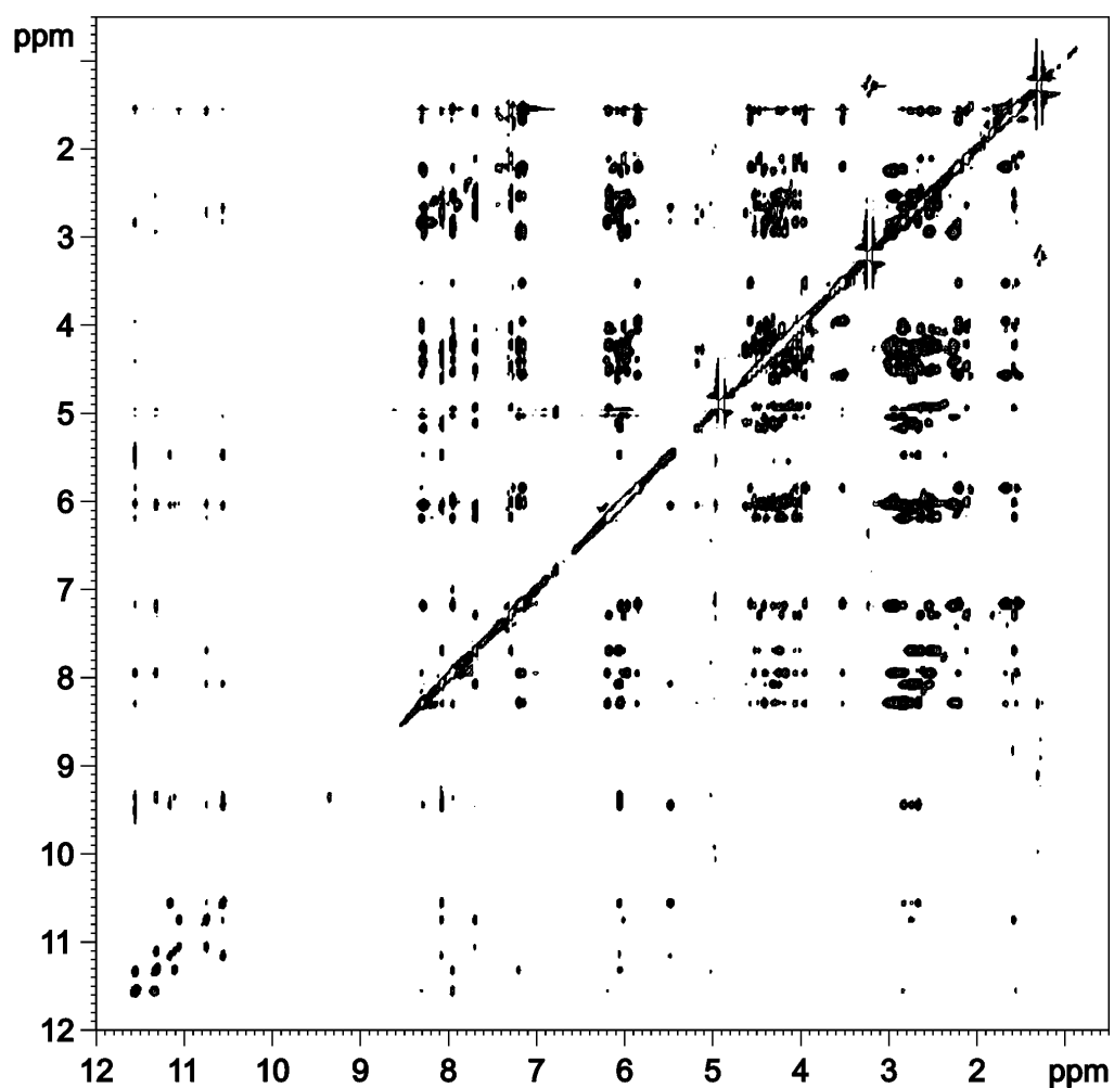
Fig.4.13: NOESY spectrum of d(TAGGAGGT) 4 in H 2 O solution, recorded at 273 K with a mixing time of 300 ms.
