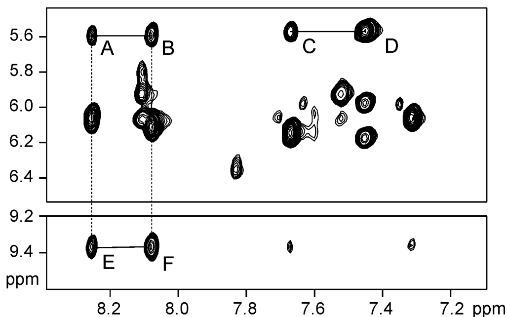
Fig.4.22: Portion of the NOESY spectrum of d(TGGAGGC) 4 showing amino-base proton interactions in the conserved central portion. NOEs, labeled (A)-(F), are assigned as follows: (A) G5NH2-A4H8, (B) G5NH2-G5H8, (C) C7H6-G6H8, (D) C7H5-H6, (E) G5NH2*-A4H8 and (F) G5NH2*-G5H8.
