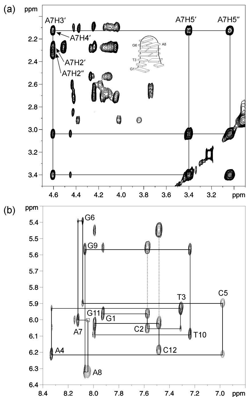
Fig.3.17: Expanded region of the 500 MHz NOESY spectrum of d(GC + ACGAAGTGC) (288 K, D 2 O, 300 ms) showing (a) the H4'-H2'/H2'' interactions of the loop nucleotide, and (b) sequential H1'-H6/H8 connectivity, typical of B-like DNA, along the oligonucleotide chain.
