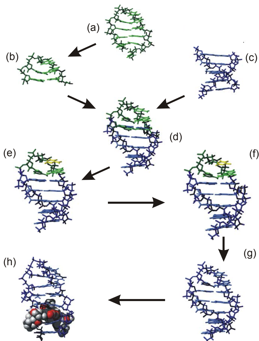
Fig.3.41: Steps involved in generating a model for the sequence d(GCCCGTAGTGC) containing a mismatched C-T base pair and bound to nogalamycin.
