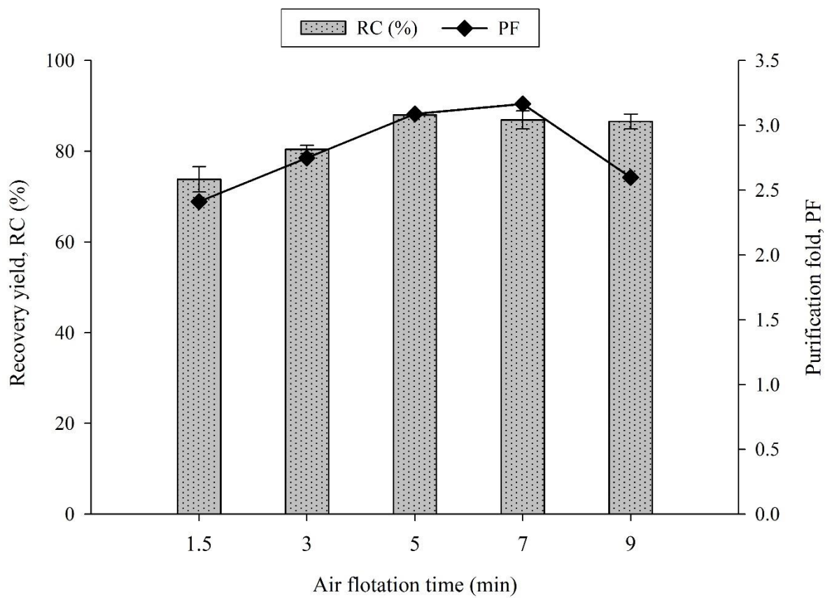
Figure 4: Effect of air flotation time (min) on the C-PC recovery yield and purification fold from S. platensis .
