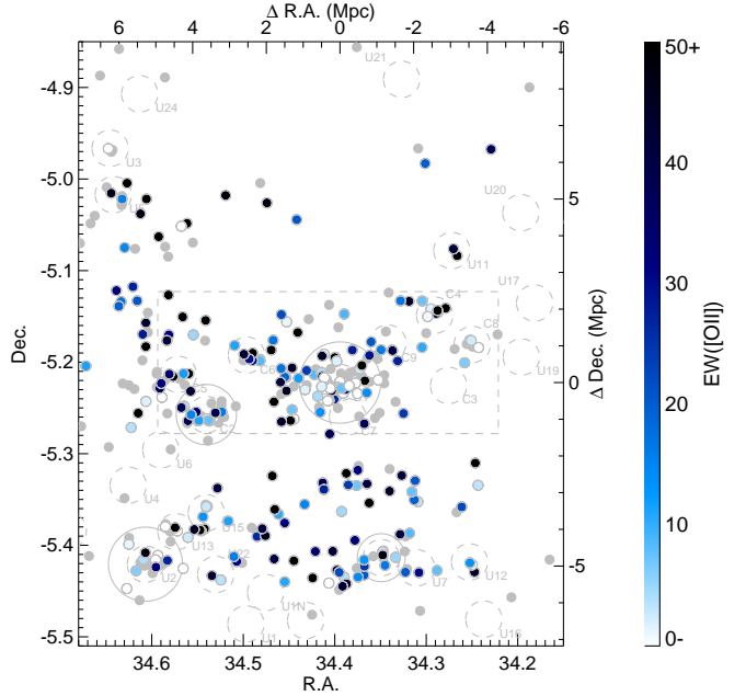
Figure 19. [OII] equivalent widths of structure members. The EW([OII]) scale is shown to the right. For visualisation purposes, sources with \text{EW}([\text{OII}]) < 0 are shown with the same colour as \text{EW}([\text{OII}]) = 0 . Similarly, sources with \text{EW}([\text{OII}]) > 50 are shown as sources with \text{EW}([\text{OII}]) = 50 . As in Figures 16 and 18, we only plot sources within |\Delta v| < 2000 \text{ km s}^{-1} of C1’s redshift; members with no spectral type information are shown in grey; the cluster candidates are marked by dashed circles of radius 500 kpc at z = 0.65 ; the virial radii of C1, C2, U2 and U9 are indicated by solid grey circles and the CANDELS footprint is shown by the dashed rectangle.
