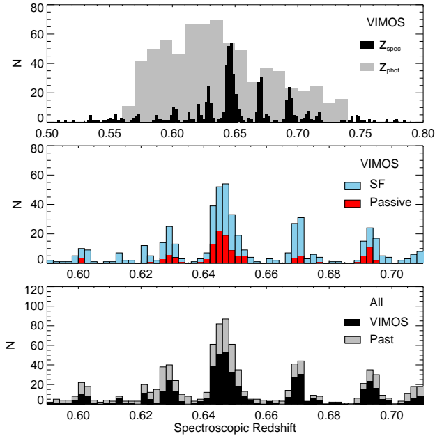
Figure 7. Spectroscopic redshifts in UDS. Top: Distribution of sources with new VIMOS redshifts (quality flag ‘A’ or ‘B’; black histogram) overlapped on top of the initial photometric redshift distribution of z \sim 0.65 targets (grey). Middle: Same as the black histogram of the top panel but this time with sources segregated by their spectral type flag i.e. passive sources (‘E’ and ‘E/SF’) in red and star-forming (‘SF’) in blue. Bottom: Combined redshifts from the present VIMOS follow-up (black) and past literature in the field (grey).
