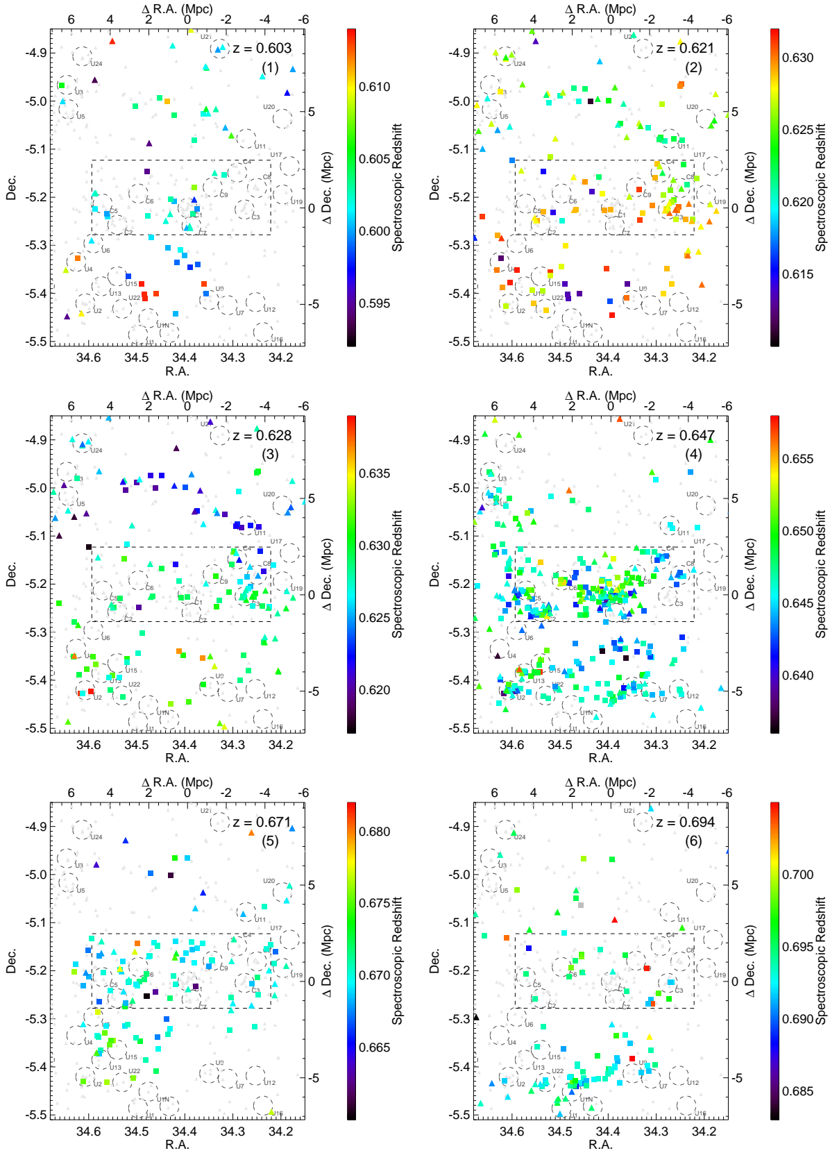
Figure 10. Spatial distribution of sources in UDS in redshift ranges of |\Delta v| < 2000 km/s centred at z = 0.603, 0.621, 0.628, 0.647, 0.671 and 0.694 (indicated on the panel top right), zoomed on the area covered by VIMOS. Sources with 0.59 < z_{\text{spec}} < 0.71 but beyond the studied redshift range are shown by the grey symbols. As in Figure 9, the new VIMOS redshifts are shown by squares and past spectroscopy by triangles. The redshift range and scale are indicated on the right of each panel. Cluster candidate are shown by dashed grey circles of radius 500 kpc at z = 0.65 and the CANDELS field of view is shown by the dashed rectangle.
