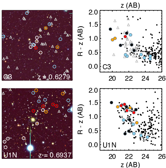
Figure 14. Same as Figure 13 for the two spectroscopically confirmed foreground and background galaxy structures C3 at z \sim 0.63 and U1N at z \sim 0.69 .
