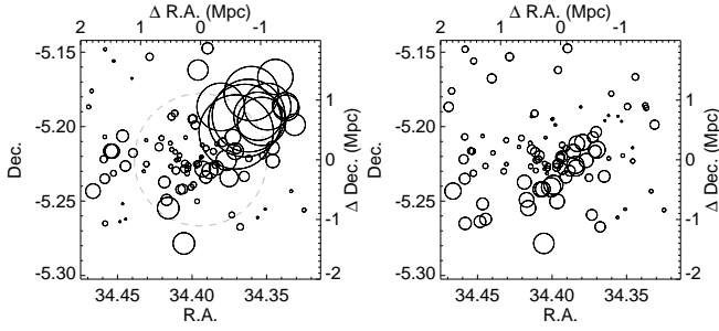
Figure 12. Dressler-Shectman bubble plot for cluster C1. Each galaxy with z_{spec} within \pm 1300 \text{ km s}^{-1} of the cluster redshift is represented with a circle whose radius is proportional to e^\delta (see text). Left: Galaxies are scaled by their deviation \delta . The dashed grey circle indicates C1 virial radius. Right: Galaxies’ velocities are randomly shuffled via 1000 Monte Carlo simulations and the \Delta statistic is recalculated. The right panel shows an example of one realisation with a median value of \Delta over the 1000 Monte Carlo random simulations.
