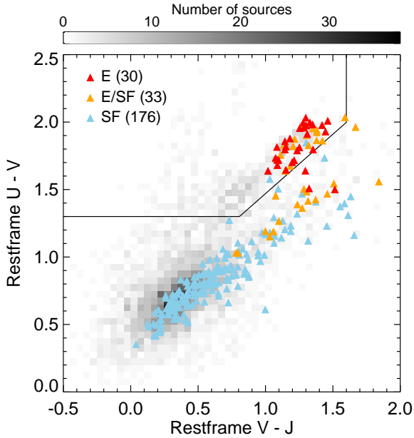
Figure 5. Restframe UVJ diagram for sources with new VIMOS spectroscopic redshifts within the CANDELS UDS field coloured by their spectral type: passive ‘E’, star-forming ‘SF’ and passive with little star formation ‘E/SF’ (with the number of sources per type into parenthesis). The black line shows the classically adopted selection criterion used to separate quiescent and star-forming galaxies at 0.5 < z < 1.0 from Williams et al. (2009). The underlying grey density map indicates the distribution in colours and density of sources with 0.56 < z_{phot} < 0.74 in CANDELS UDS.
