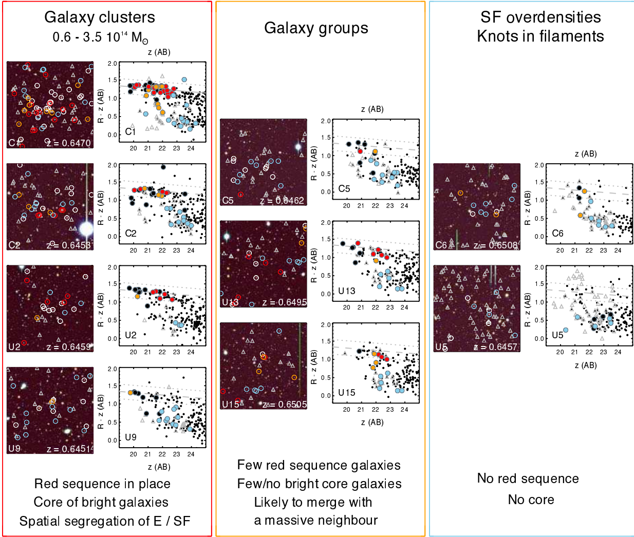
Figure 13. 3-colour images and R - z versus z colour-magnitude diagrams of the structures confirmed at z \sim 0.65 . Clump Id. are indicated at the bottom left. The structures are classified between ‘Galaxy clusters’, ‘Galaxy groups’ and ‘Star-forming galaxy overdensities’ (see section 7.4 for details). In the left panels, the ‘blue’, ‘green’ and ‘red’ images correspond to Subaru/Suprime-Cam B , R and z -band respectively. Each image is 4' on a side. Circles show galaxies with |\Delta v| < 2000 \text{ km s}^{-1} of the structure redshift (and within 1 Mpc of the structure centre for the colour-magnitude diagrams). Red, orange and blue symbols correspond to galaxies with spectral types ‘E’, ‘E/SF’ and ‘SF’ respectively. White (left) / black large (right) symbols designate sources with redshifts collected from past surveys for which spectral type information is lacking. Grey triangles show confirmed foreground and background sources. The colour-magnitude diagrams also show all sources within 1 Mpc of the cluster centre (small black dots) tracing the location of the bulk of the population along the line of sight, independently of redshift. C1’s red sequence of passive members was linearly fit (solid line; \pm 2 times scatter shown by dotted lines) and propagated through all colour-magnitude diagrams (dashed lines) to guide the eye.
