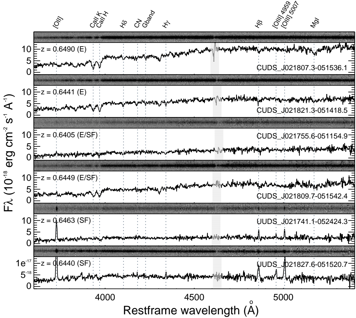
Figure 4. VIMOS spectra of galaxies with different spectral types: passive (spectral type ‘E’; two top rows), passive with little on-going star formation (spectral type ‘E/SF’; two middle rows) and star-forming (‘SF’; two bottom rows). The labels on the top left of each panel indicate the spectroscopic redshift and spectral type. The source identification number is shown on the right. The main detected emission/absorption lines are indicated by the vertical dotted lines. The dashed grey area marks the part of the spectrum strongly affected by atmospheric absorption. The corresponding 2D spectrum is shown at the top of each panel.
