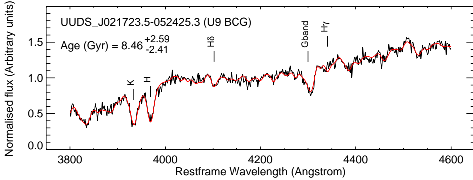
Figure 17. Example of a (normalised) galaxy spectrum (black) and best-fit stellar population model (red) for one confirmed passive structure member, UUDS_J021723.5-052425.3, U9 BCG. Spectral absorption features are indicated to guide the eye. Stellar age estimate and uncertainties are indicated in the top left corner.
