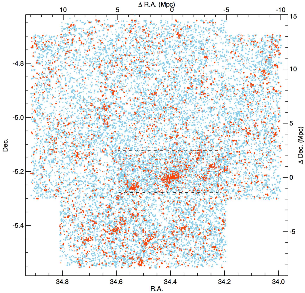
Figure 1. Spatial distribution of sources with 0.56 < z_{phot} < 0.74 in the UDS field. Galaxies with R - z > 1 (the ‘passive’ candidates) and with R - z < 1 (the ‘star-forming’ candidates) are shown in red and blue dots respectively. Sources brighter (fainter) than R = 24 are shown by large (small) dots. The CANDELS HST field is shown by the dashed rectangle.
