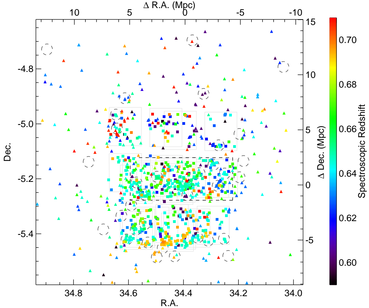
Figure 9. Spatial distribution of sources in UDS with 0.59 < z_{\text{spec}} < 0.71 coloured according to their redshifts. New VIMOS measurements and past spectroscopy are shown by squares and triangles respectively. The probed redshift range and colour scale are indicated to the right of each panel. Cluster candidate are shown by dashed grey circles of radius 500 kpc at z = 0.65 . The CANDELS field of view is specified by the dashed rectangle. The VIMOS masks are overplotted in light grey to guide the eye on the spectroscopic coverage of the structure.
