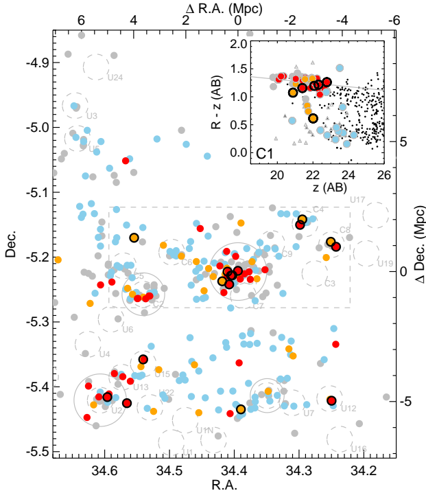
Figure 16. Spatial distribution of post-starburst galaxies (black circles) across the structure. Red, orange and blue symbols correspond to the spectral types ‘E’, ‘E/SF’ and ‘SF’ respectively. Members lacking spectral type information (i.e. from past literature) are shown in grey. We only consider sources within |\Delta v| < 2000 \text{ km s}^{-1} of C1’s redshift. Cluster candidates are marked by dashed circles of radius 500 kpc at z = 0.65 . The virial radii of C1, C2, U2 and U9 are indicated by solid grey circles. The CANDELS footprint is displayed by the rectangle. The inset shows the location of post-starburst galaxies within C1’s virial radius in a colour-magnitude diagram.
