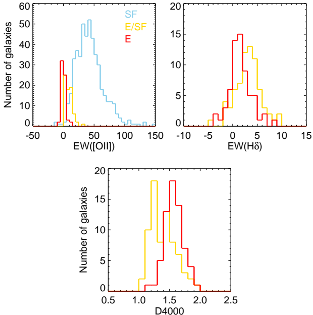
Figure 8. Distribution of spectral index measurements for galaxies with spectroscopic redshifts. Top Left: Equivalent width EW([OII]) for all galaxies colour-coded by their spectral type (‘E’ in red, ‘E/SF’ in orange and ‘SF’ in blue). Top Right & Bottom: EW(H\delta) and D4000 respectively for passive galaxies (‘E’ and ‘E/SF’).
