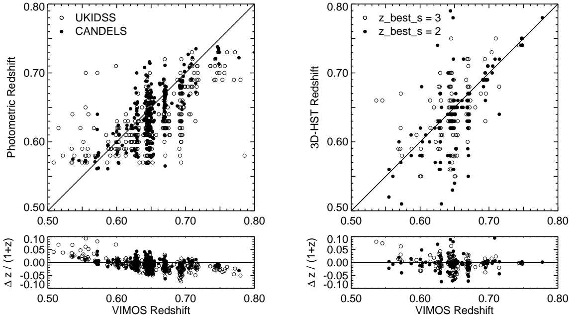
Figure 6. Comparison of VIMOS spectroscopic redshifts (flags A & B) with past redshift estimates from the literature. Left: Comparison with photometric redshifts ( z_{\text{phot}} ) for sources within the CANDELS field of view (filled symbols; Santini et al. 2015) and outside (open symbols; Hartley et al. 2013). Right: Comparison with grism redshifts ( z_{\text{grism}} ) for sources in the CANDELS footprint from the 3D-HST survey (Momcheva et al. 2016, flag ‘z_best_s’ = 2). Photometric redshifts derived by the 3D-HST team (Skelton et al. 2014) are shown by the open symbols for sources in 3D-HST with no grism redshift (‘z_best_s’ = 3). The bottom panels show the difference \Delta z = z_{\text{phot or grism}} - z_{\text{spec}} rescaled by (1+z) .
