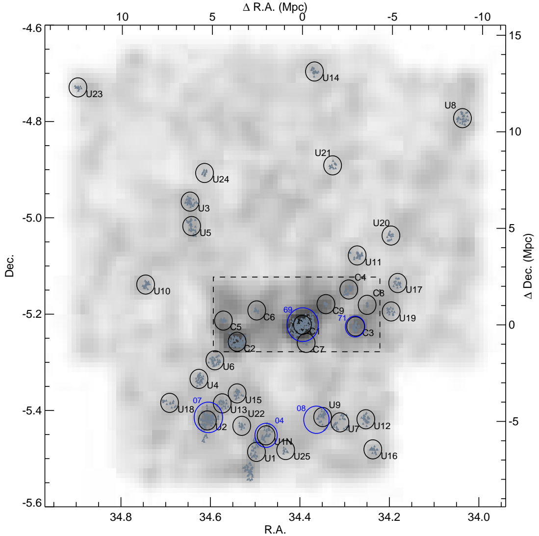
Figure 2. Spatial distribution of the galaxy cluster candidates at z \sim 0.65 (black circles) and associated cluster member candidates (grey triangles) detected by the cluster search algorithm. The distribution is plotted over the density map of sources with 0.56 < z_{phot} < 0.74 . The map is derived from the density of ‘red’ + ‘blue’ dots from Figure 1 in area of 0.01 \times 0.01 degree smoothed by a gaussian kernel with radius r = 3 (i.e. 0.03 deg) and standard deviation \sigma = r/2 . The circles are centred at the cluster centre estimates; their radii correspond to 0.5 Mpc at z = 0.65 . The F10 X-ray-detected structures at 0.6 < z_{phot} < 0.7 are shown by the blue circles, along with their F10 ID number; the circle radius corresponds to the F10 R_{200} estimate.
