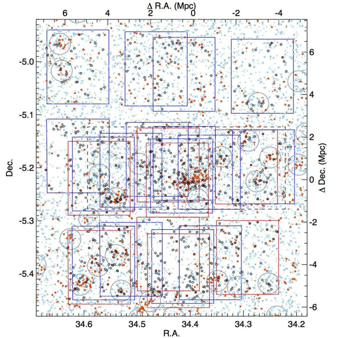
Figure 3. Coverage of the VIMOS masks on top of the distribution of sources with 0.56 < z_{phot} < 0.74 (colour coding as in Fig. 1). The layouts of the so-called 'deep' ( \sim 2 hrs of exposure time) and 'shallow' ( \sim 1 hr) 4-quadrant VIMOS masks are indicated in red and blue respectively. The observed targets are shown by the black open circles. The cluster candidates at z_{phot} \sim 0.65 are shown by the grey circles.
