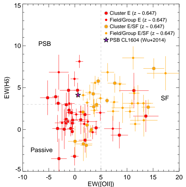
Figure 15. EW(H\delta) versus EW([OII]) for the passive sources (spectral types ‘E’ and ‘E/SF’ in red and orange circles respectively) confirmed at the large-scale structure redshift i.e. |\Delta v| < 2000 km/s from z = 0.647 . The selection criterion used to isolate post-starburst systems (‘PSB’; EW(H\delta) > 3\text{\AA} and EW([OII]) < 5\text{\AA} ) is shown by the grey lines i.e. PSB galaxies are located in the upper left quadrant. Passive galaxies classically have EW(H\delta) < 3\text{\AA} and EW([OII]) < 5\text{\AA} while star-forming galaxies (‘SF’) have EW([OII]) > 5\text{\AA} . Sources within the virial radius of clusters ‘C1’, ‘C2’, ‘U2’ and ‘U9’ (our ‘cluster’ sample) are indicated by larger symbols. For comparison, the average spectral indices derived from a composite spectrum of post-starburst galaxies in the large-scale structure CL 1604 at z \sim 0.9 are indicated by the purple star (Wu et al. 2014, ‘O5 sample’).
