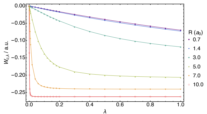
FIG. 2. The correlation adiabatic connection integrand values (a.u.) of Eq. (42), calculated using the optimization of Eq. (9), lines, and Eq. (31), point markers, for the \text{H}_2 molecule at internuclear separations R = 0.7, 1.4, 3.0, 5.0, 7.0 and 10.0 a.u.
