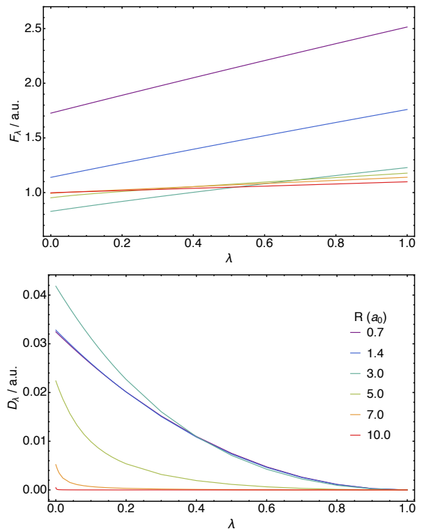
FIG. 1. F_\lambda of Eq. (9), upper panel, and D_\lambda of Eq. (31), lower panel (a.u.) as functions of the interaction strength \lambda for the H 2 molecule at internuclear separations R = 0.7, 1.4, 3.0, 5.0, 7.0 and 10.0 a.u.
