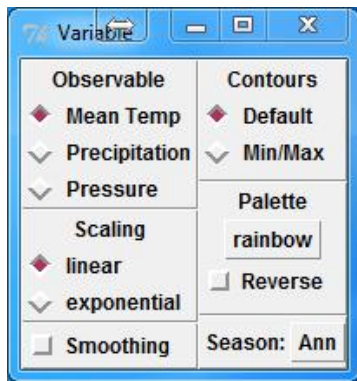
Figure A-5 SCENGEN variables
