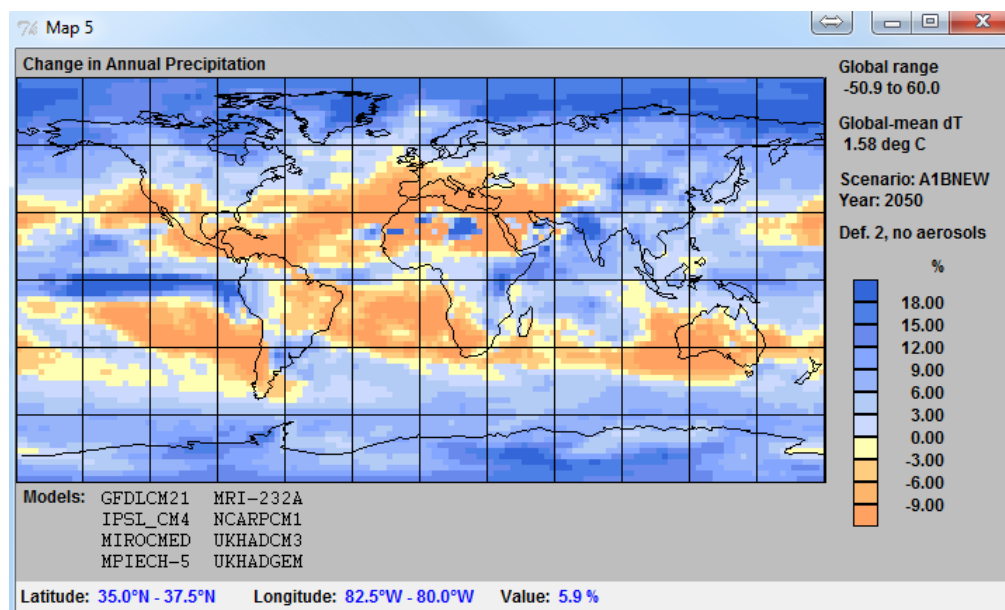
Figure A-22 SCENGEM: local precipitation change projection under A1B scenario for 2050
