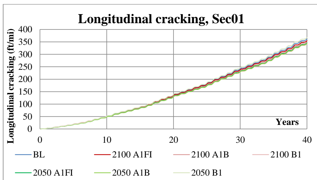
Figure A-35 Longitudinal cracking prediction under various emission scenarios for Sec01
