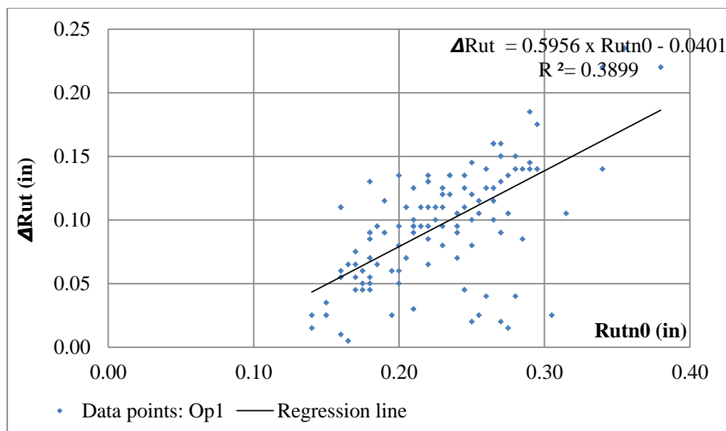
Figure A-48 Regression analysis: maintenance effect of Op1 on rutting
