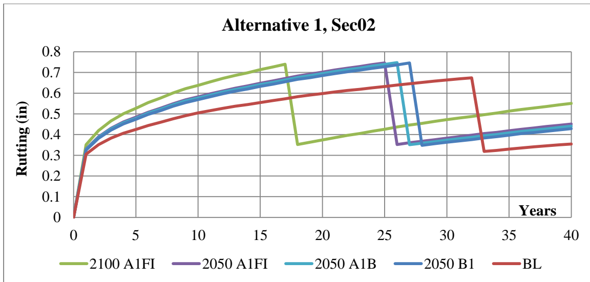
Figure A-63 Rutting curve, Alternative 1, Sec02
