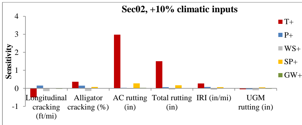
Figure A-32 Sensitivity of pavement performance to climatic factors (inputs +10%, Sec02)
