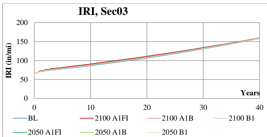
Figure A-46 IRI prediction under various emission scenarios for Sec03
