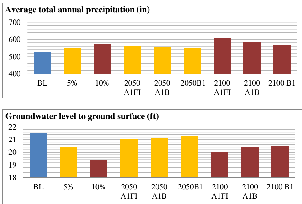
Figure 3-13 Modified climatic factors comparison under BL, 5% increase, 10% increase, and some emission scenarios for Sec02 (BL = baseline, 1 in = 25.4 mm, and 1 foot \approx 0.3 m)
