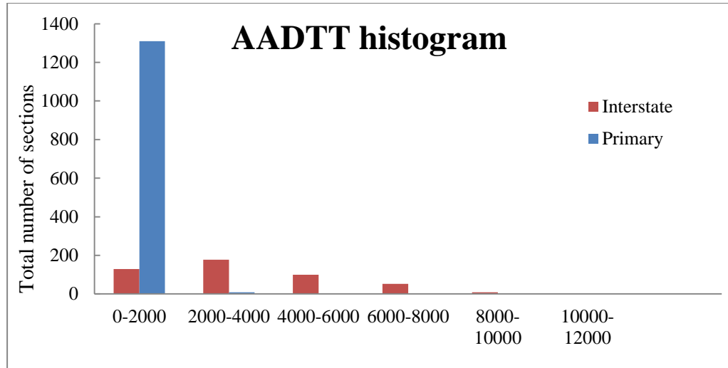
Figure 3-4 A histogram of sections' AADTT for interstate and primary roads in Bristol, Salem, and Richmond
