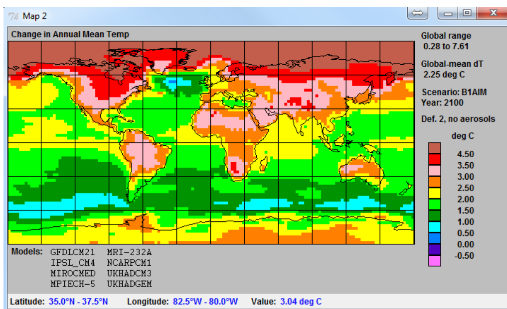
Figure A-19 SCENGEM: local temperature change projection under B1 scenario for 2100
