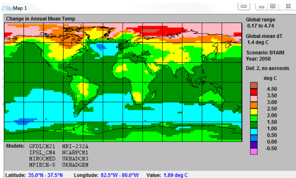
Figure A-18 SCENGEM: local temperature change projection under B1 scenario for 2050
