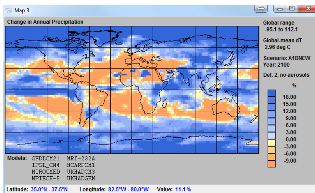
Figure A-23 SCENGEM: local precipitation change projection under A1B scenario for 2100
