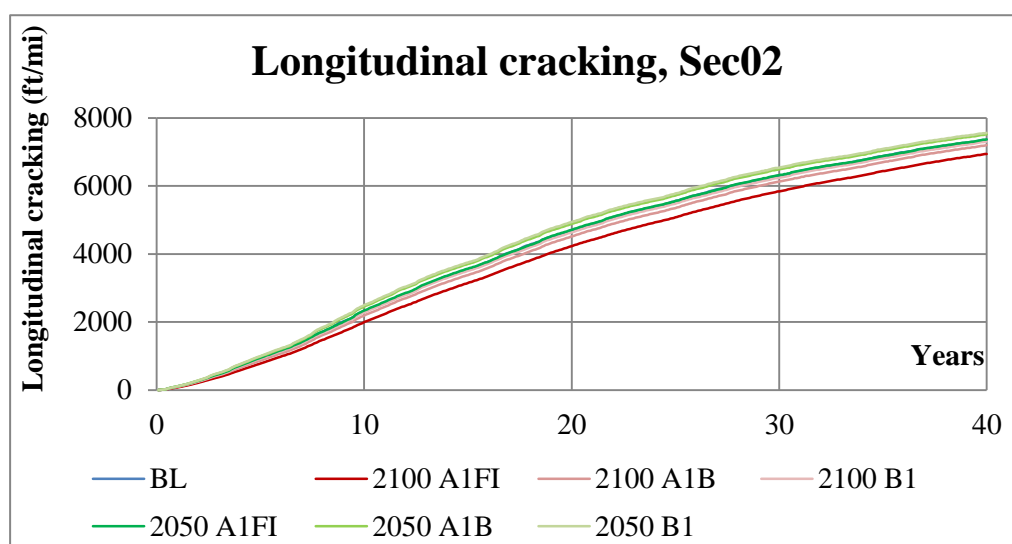
Figure A-39 Longitudinal cracking prediction under various emission scenarios for Sec02
