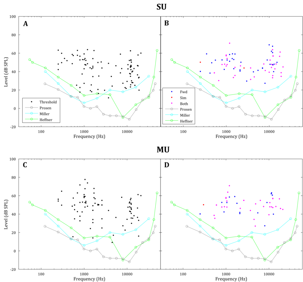
Figure 2.7 A & C Threshold of units derived from rate level functions plotted against CF, for SU and MU respectively. B & D Fixed level of signal for each notched noise experiment; blue = units yielding just a forward masked ERB, red = just simultaneous, and magenta = both. Audiograms of the guinea pig taken from Miller and Murray (1966), Heffner et al. (1971) and Prosen et al. (1978).
