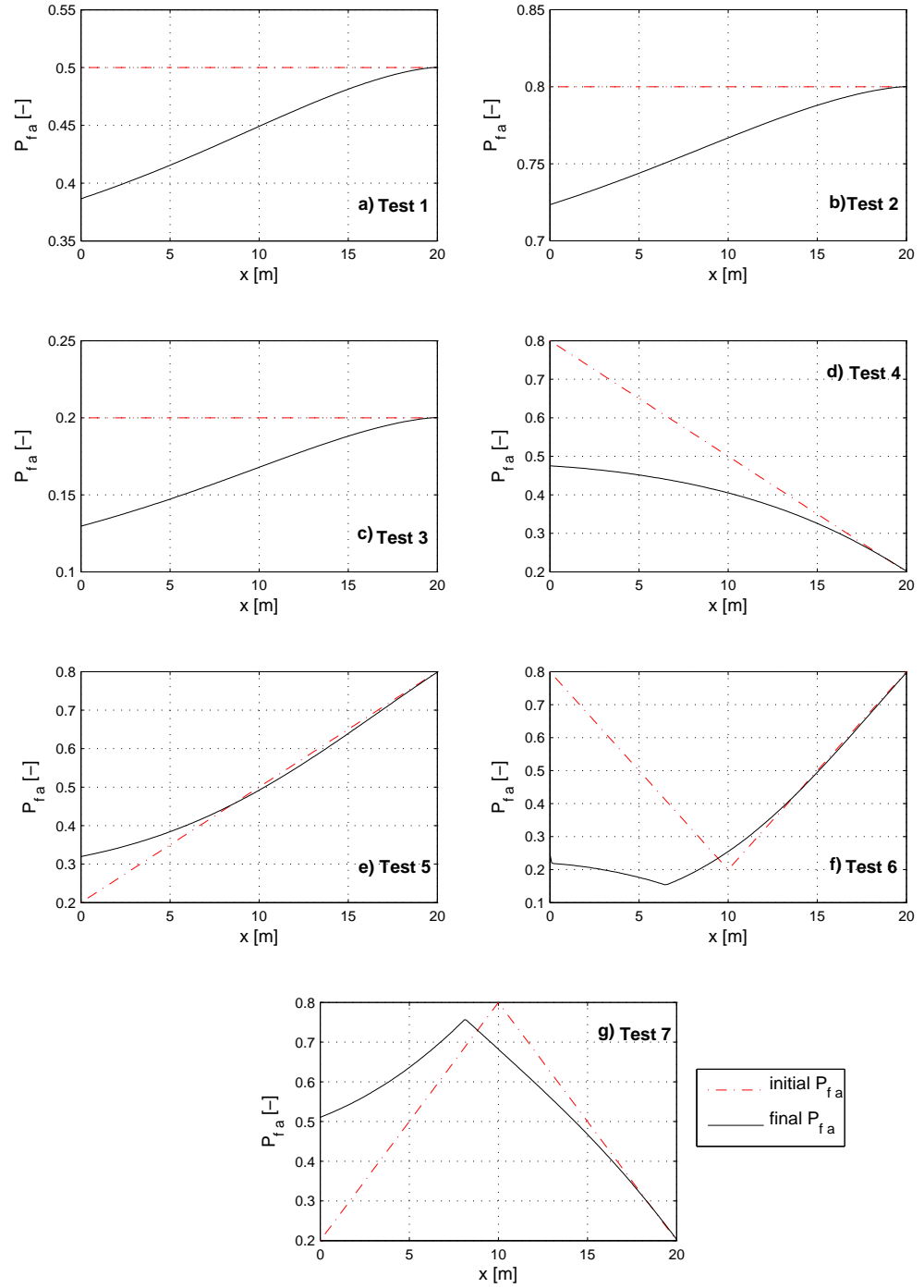
Figure 7.4: Comparison of the final fine volume fraction for all the PW01 numerical tests. Initial P_{fa} --- , final P_{fa} —
