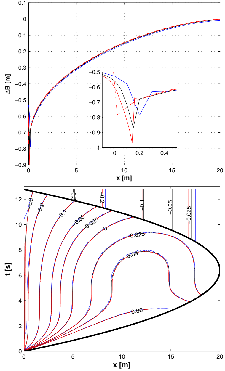
Figure B.2: Top: Convergence in change in bed \Delta B relative to the initial bed profile at the end of the simulation; — PH05 solution. Bottom: Convergence of contours for \Delta B . For both graphs: — \Delta x = 0.1 m and \Delta t = 0.004 s; — \Delta x = 0.05 m and \Delta t = 0.002 s; — \Delta x = 0.02 m and \Delta t = 0.001 s.
