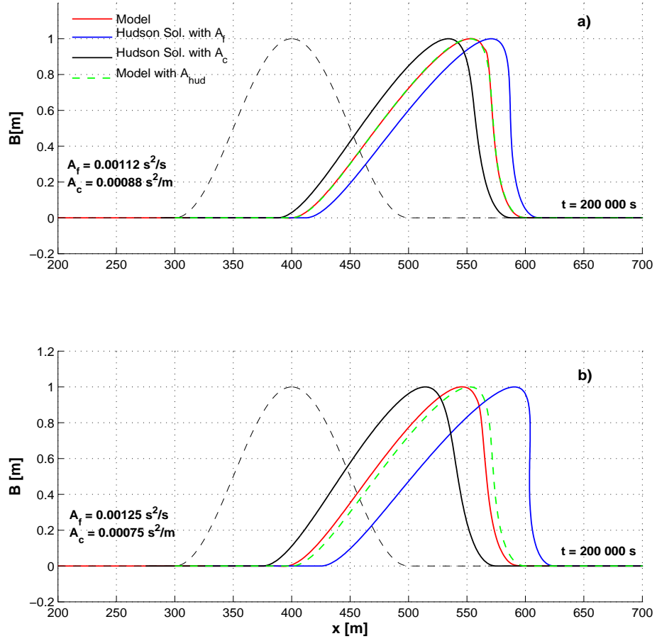
Figure 4.12: Bed level results at t = 200\,000 s for a) Test 7 and b) Test 8. - - Initial condition.
