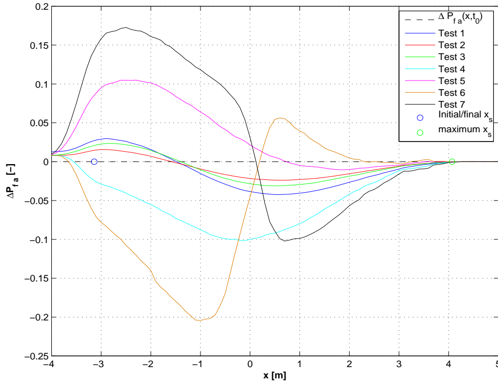
Figure 7.10: Compraison of the final \Delta P_{fa} for the non-breaking wave numerical tests
