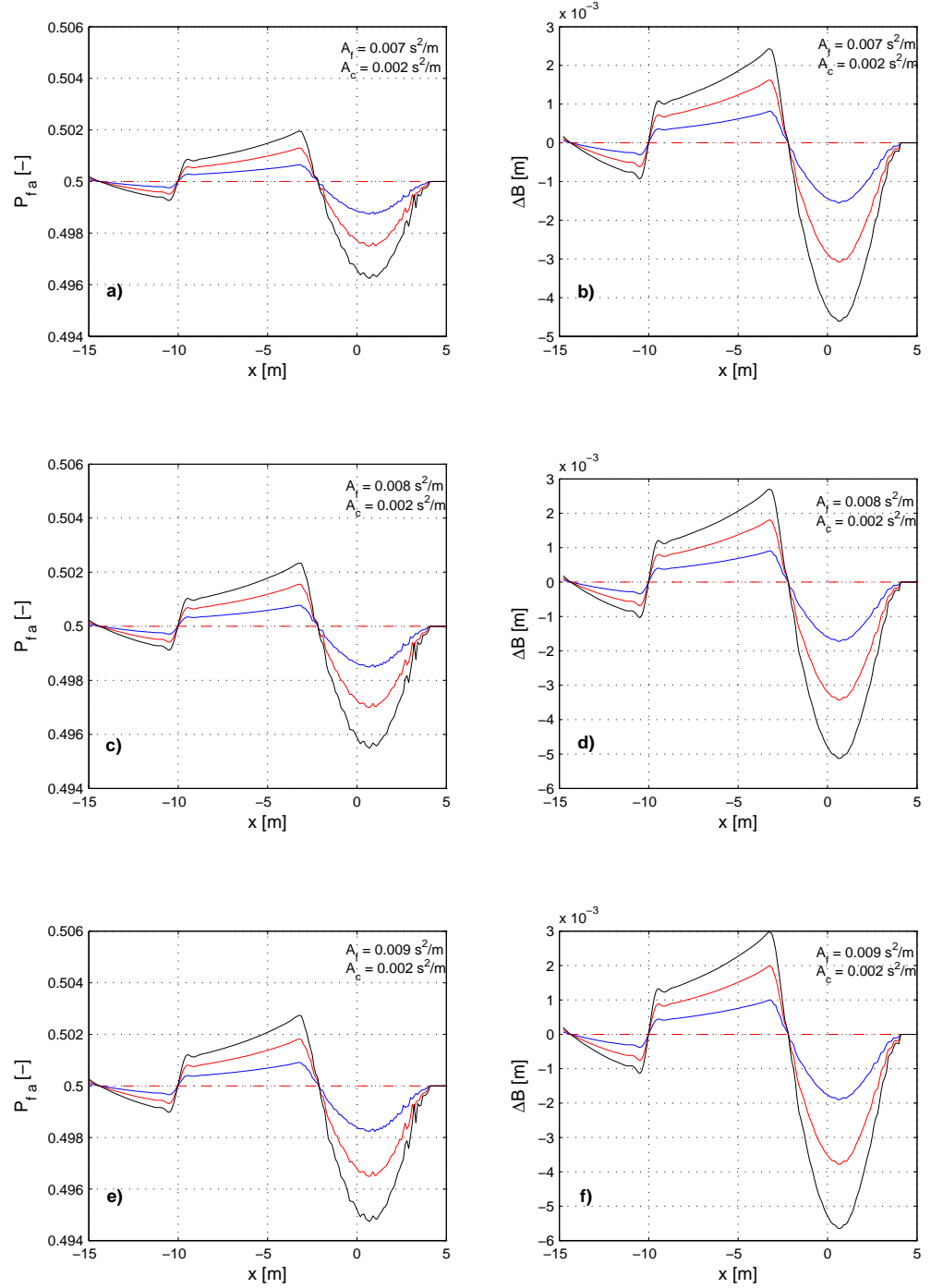
Figure 6.18: Final P_{fa} and bed change after one, two and three swash events. a) and b) A_f = 0.007 \text{ s}^2/\text{m} A_c = 0.002 \text{ s}^2/\text{m} ; c) and d) A_f = 0.008 \text{ s}^2/\text{m} A_c = 0.002 \text{ s}^2/\text{m} ; and e) and f) A_f = 0.009 \text{ s}^2/\text{m} A_c = 0.002 \text{ s}^2/\text{m} ; — 1 st swash; — 2 nd swash; — 3 rd swash
