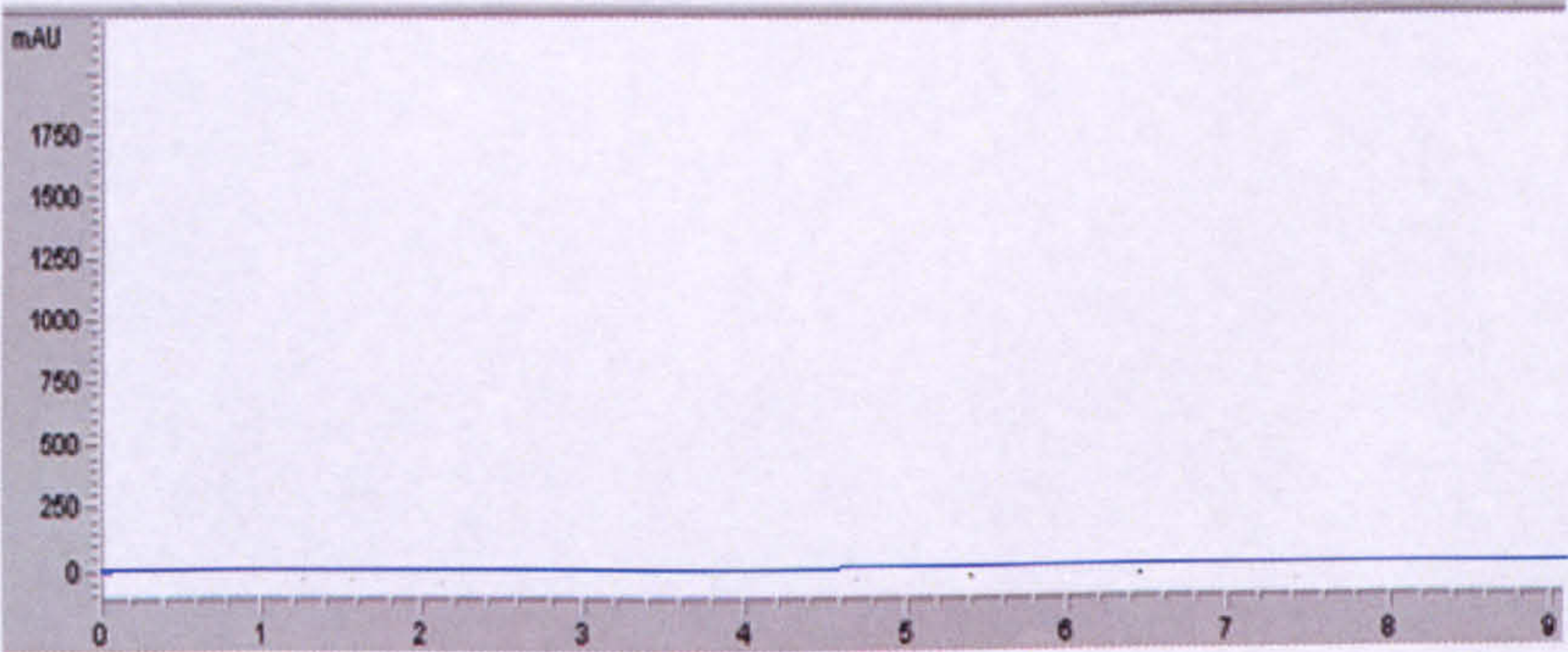
Figure 3.6: Chromatogram showing the absence of ergosterol in healthy roots. The retention time for ergosterol is 5.5-5.8 min.
