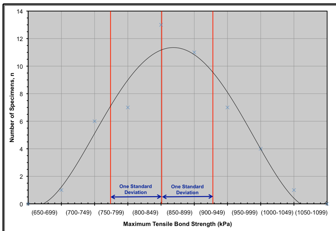
Figure 5.16 Distribution of maximum tensile bond strength
