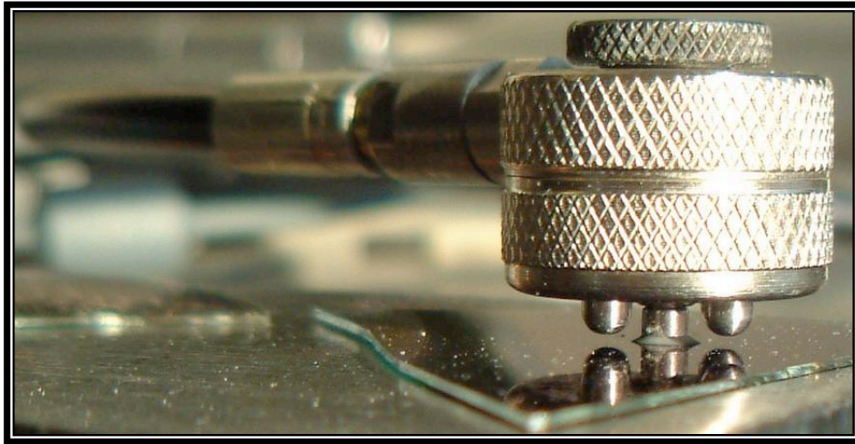
Figure 2.15 Pull off test developed by DFD® Instruments (Source: DFD® Instruments n.d.)
