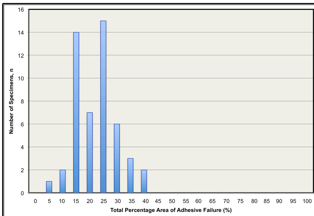
Figure 5.14 Histogram of total percentage area of adhesive failure
