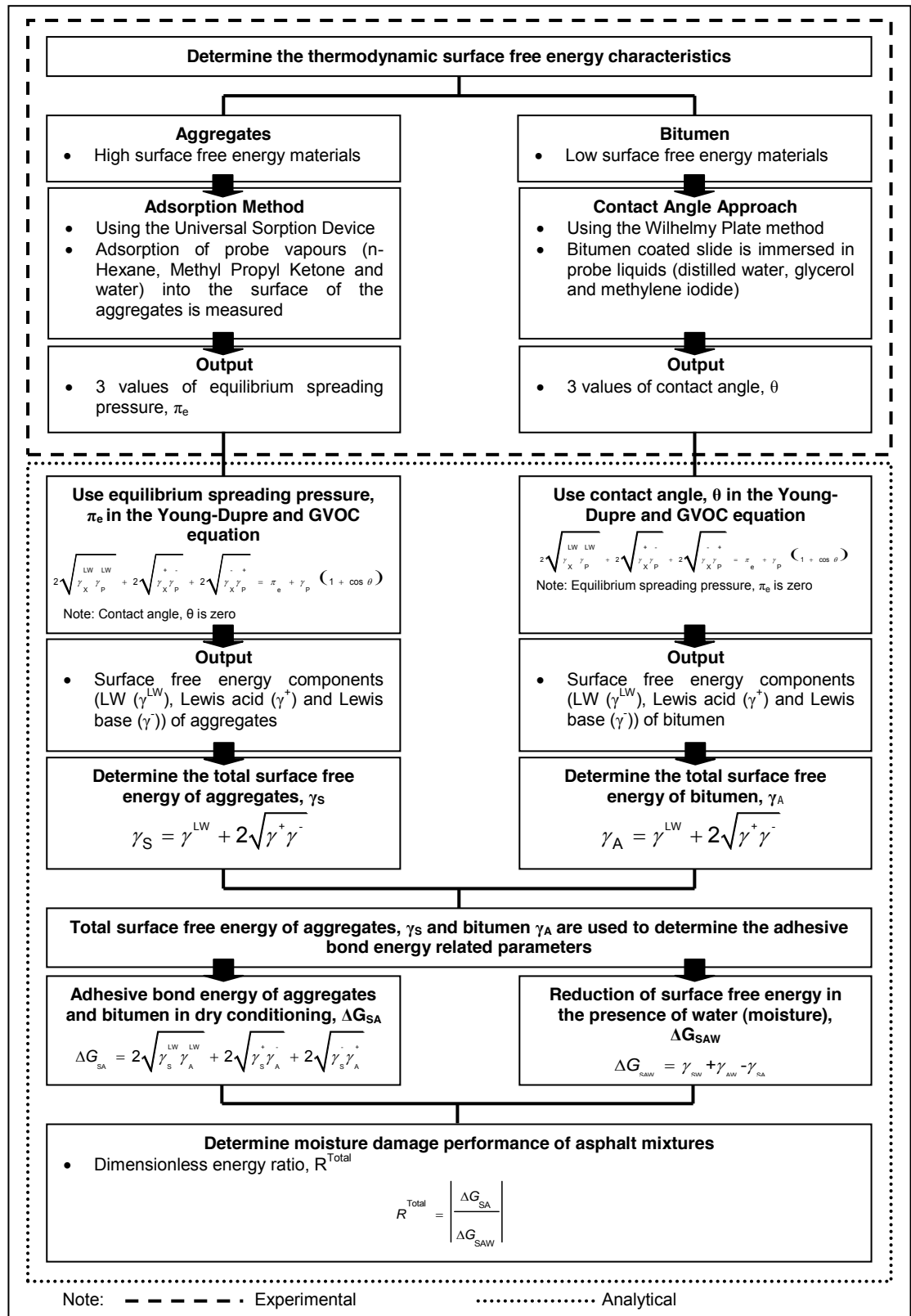
Figure 2.8 Procedures for measuring adhesive bond strength based on thermodynamic surface free energy (Source: Bhasin et al. 2006)
