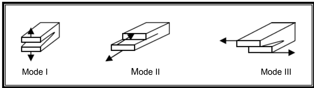
Figure 2.19 Mode of failure (Mode I, Mode II and Mode III)
