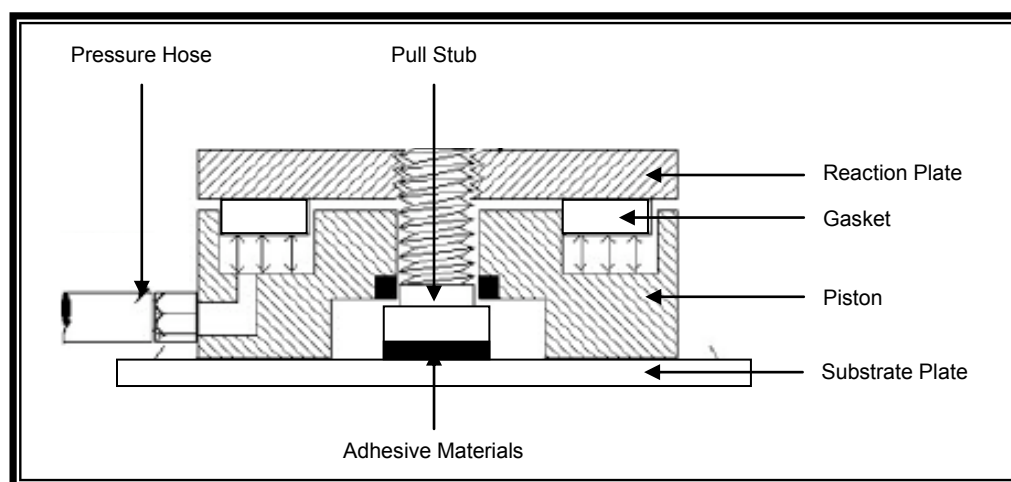
Figure 2.38 Schematic drawing of PATTI 110 (Source: Kanitpong & Bahia 2003)
