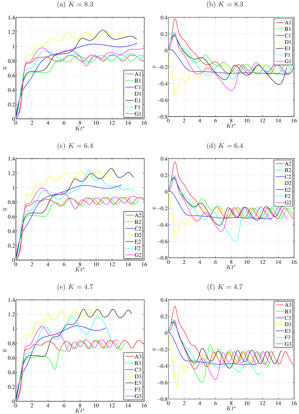
Figure 6.25: CFD-RBD predictions of horizontal along-wind velocity (left) and vertical velocity (right) of plates with varying initial angle of attack and in flow conditions of Tachikawa number; (a,b) K = 8.3 , (c,d) K = 6.4 and (e,f) and K = 4.7 .
