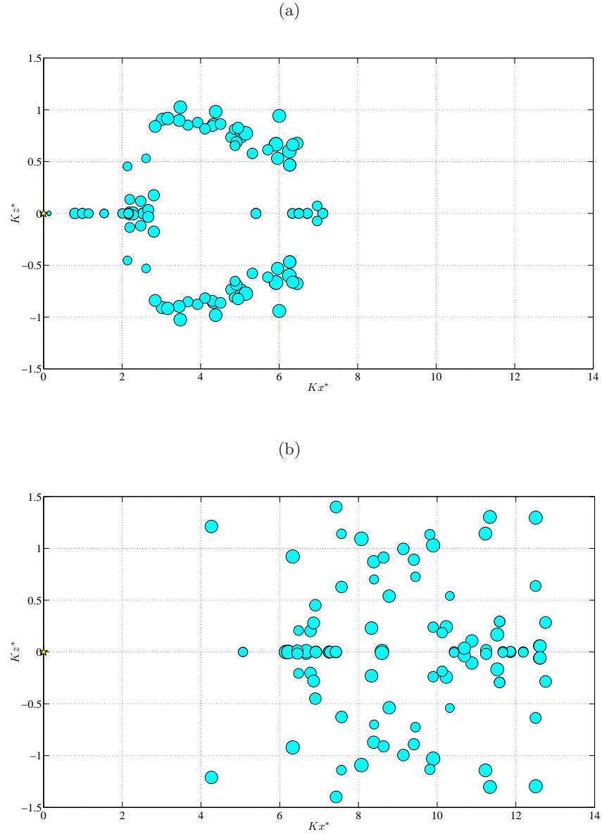
Figure 6.11: Scatter plot of debris impact location relative to the launch position (★) for (a) 3 m launch height and (b) 10 m launch height, with points scaled according to impact kinetic energy.
