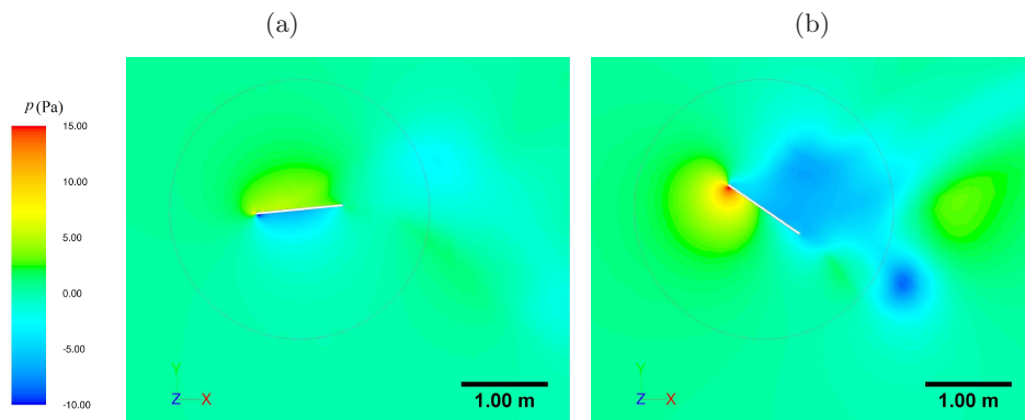
Figure 5.23: CFD predicted pressure field around a rotating plate with \overline{\omega} = 0.28 at (a) \alpha_z \approx 0^\circ , and (b) \alpha_z \approx 30^\circ .
