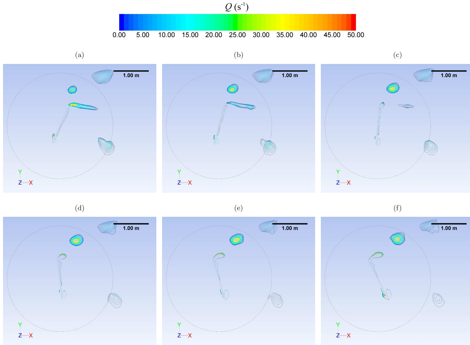
Figure 5.20: Q -value contours on a vertical plane through the centre of a post-autorotating plate of dimensionless rotational speed \bar{\omega} = 2.0 . Contours are taken at instantaneous angles of attack of (a) -60^\circ , (b) -80^\circ and (c) -100^\circ .
