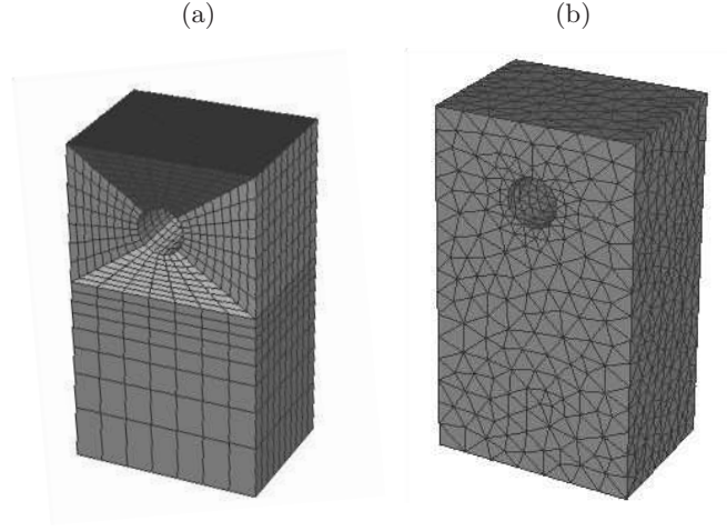
Figure A.1: (a) A structured mesh of hexahedral cells and (b) an unstructured mesh of tetrahedral cells.
