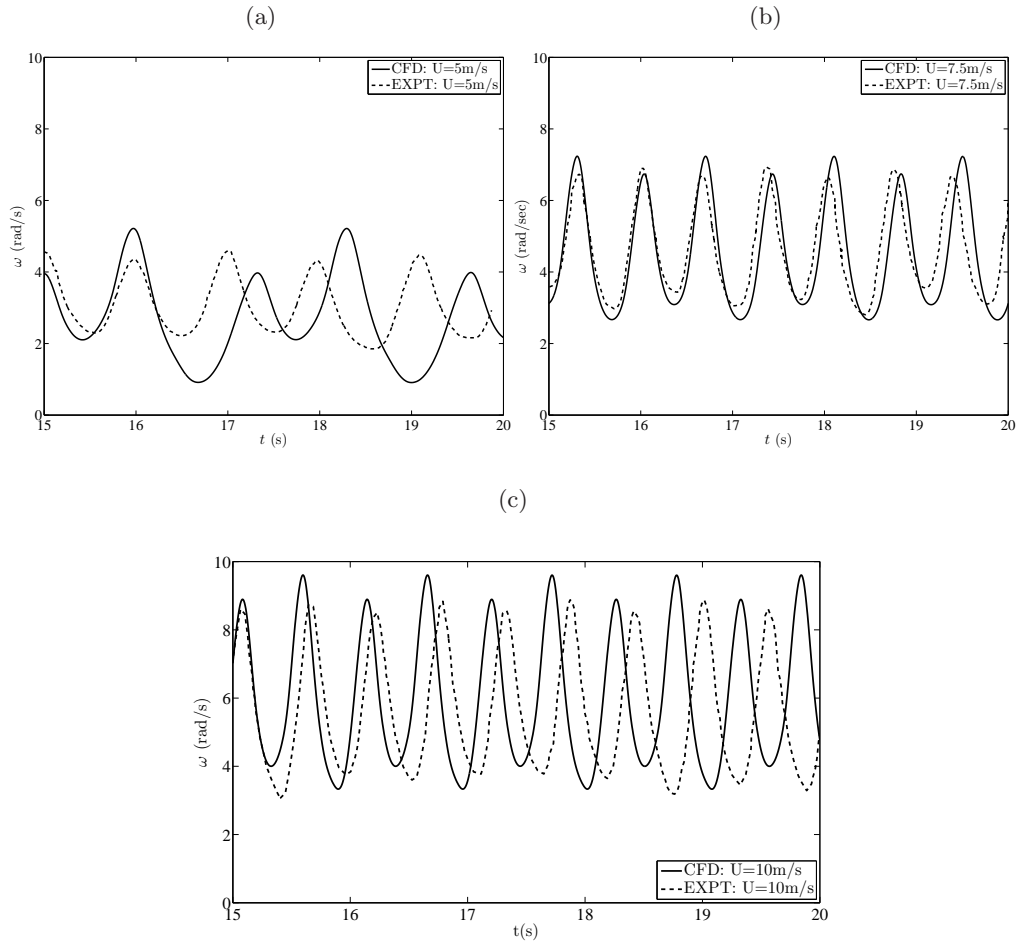
Figure 5.31: Auckland domain CFD-RBD predictions and experimental gyroscope measurements of rotational speed for a 1 m square flat plate in a uniform wind stream of (a) 5.0 m/s, (b) 7.5 m/s and (c) 10.0 m/s
