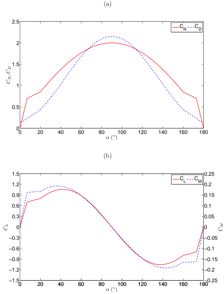
Figure 2.8: Steady-state curves showing the variation of (a) Normal Force and Drag coefficients, (b) Lift and Torque coefficient, with angle of attack for static square flat plates held in a uniform steady flow. Curves are computed using piece-wise linear approximations of C_N and x_cp curves from ESDU (1970).
