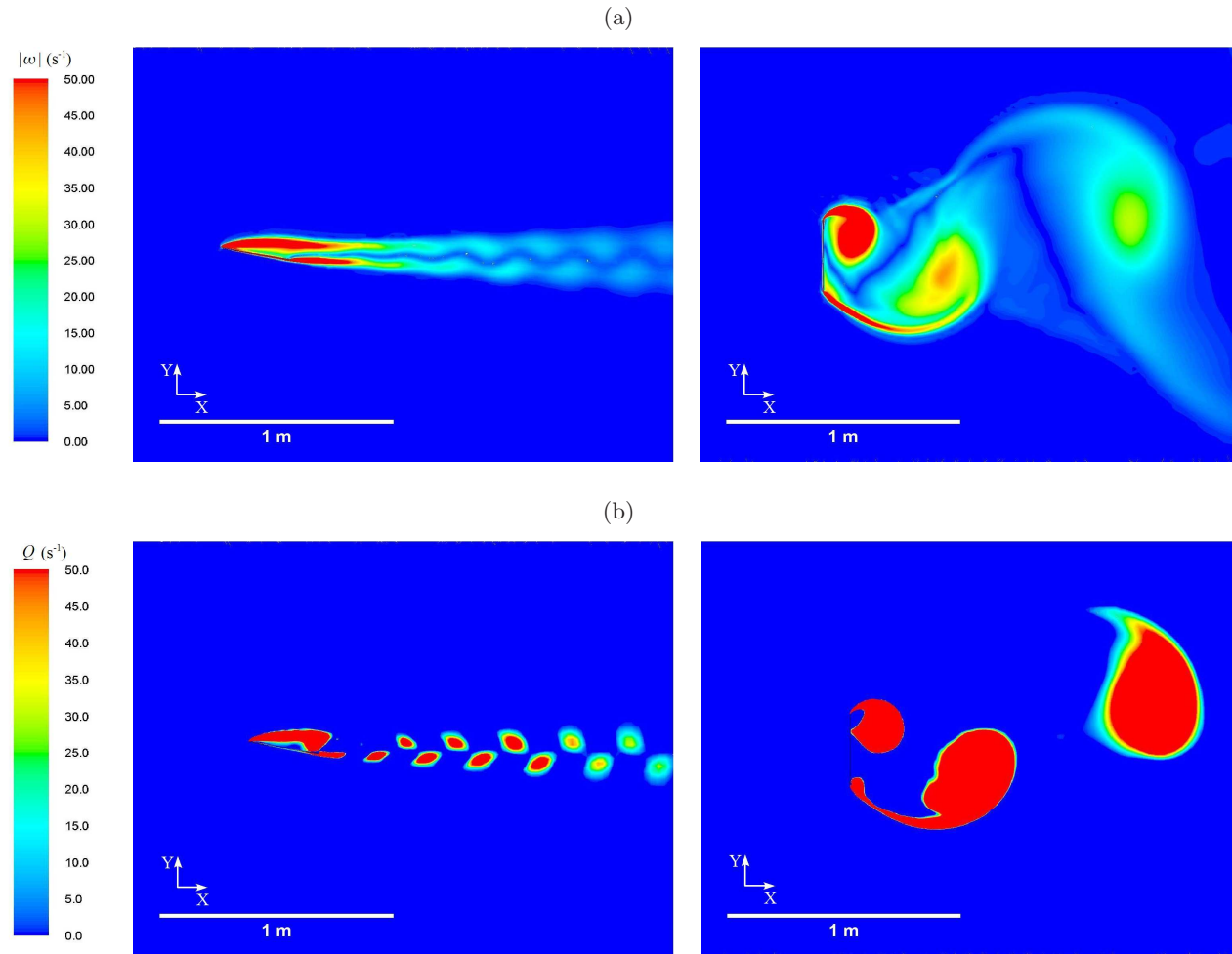
Figure 5.3: CFD predictions for (a) vorticity magnitude, |\omega| ( \text{s}^{-1} ) and (b) Q -criterion value, Q ( \text{s}^{-1} ), in the wake of a 2D static plate held at \alpha = 10^\circ (left) and \alpha = 90^\circ (right) in a uniform flow of \text{Re} = 5.46 \times 10^4 .
