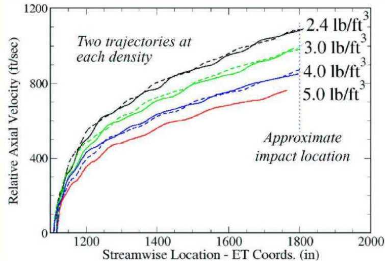
Figure 2.27: Axial velocities for debris pieces with volume of 704 cubic inches and different foam densities. Dotted and dashed line indicate different initial condition sets (Gomez et al., 2004).
