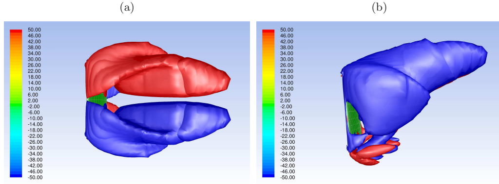
Figure 5.22: Iso-surfaces of positive and negative helicity showing the two counter-rotating tip vortices as regions of high helicity near the advancing edge for a plate rotating with \overline{\omega} = 0.28 . (a) Plan view and (b) side view.
