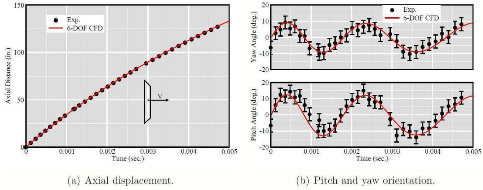
Figure 2.28: Comparison of free-flight and computed translation and rotation variations for un-tripped frustum trajectory obtained in the NASA Ames GDF. Initial Mach number is 2.74. Uncertainty approximated from visual inspection of reduced data. ( D/t = 5, \theta = 40^\circ ) (Gomez et al., 2004; Murman et al., 2005).
