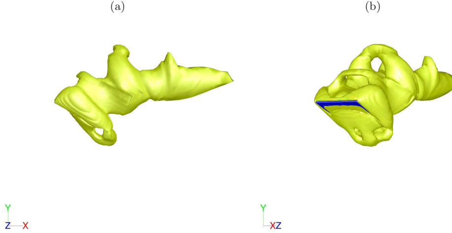
Figure 5.24: Iso-surfaces of Q = 10 showing flow structures in the wake and at the front face, near the retreating trailing edge, of a post-autorotational plate with \varpi = 2.0 . (a) Side view and (b) Isometric view.
