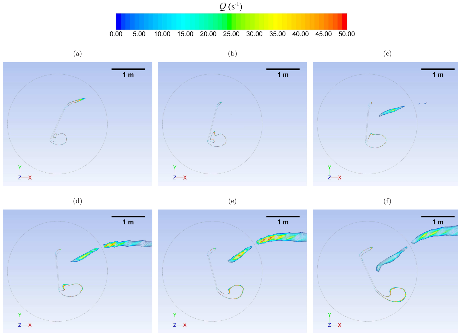
Figure 5.17: Q-value contours on a vertical plane through the centre of a pre-autorotating plate of dimensionless rotational speed \bar{\omega} = 0.28 . Contours are taken at instantaneous angles of attack of (a) -60^\circ , (b) -80^\circ and (c) -100^\circ .
