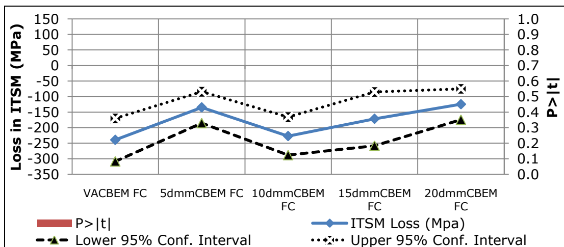
Figure 6.37: Loss in ITSM at Fully Cured Condition due to a 1% Rise in Air Void Content
