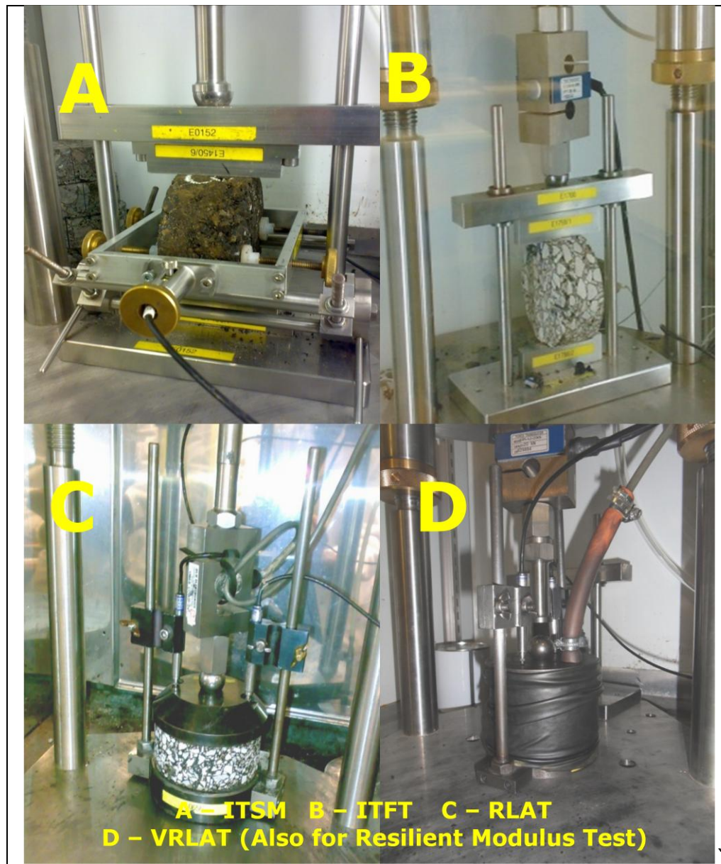
Figure 6.9: Different Modes of Testing in the NAT
