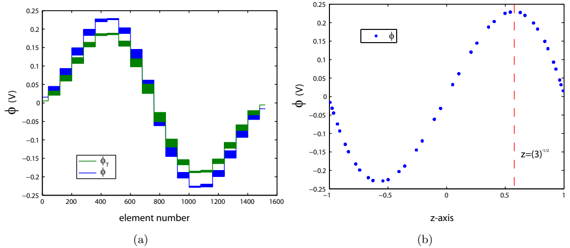
Figure 7.8: (a) Variation of the potential at the surface of a sphere meshed using 1520 elements rotating about the z-axis in a z-gradient; (b) variation of the numerically computed potential, \phi , with the z coordinate of the element for a sphere meshed using 1520 elements rotating about the z-axis in a z-gradient.
