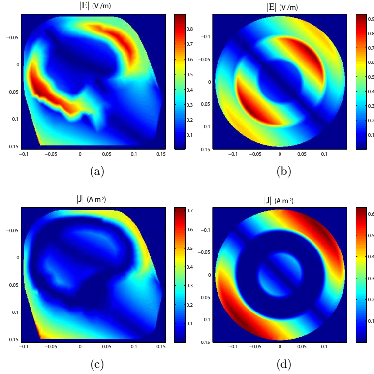
Figure 7.12: Three domain model rotating ( \Omega = 1 \text{ rad s}^{-1} ) in a uniform magnetic field ( \mathbf{B} = 7(\hat{\mathbf{i}} + \hat{\mathbf{j}}) ): (a) electric field modulus in the yz-plane for the system scalp-skull-brain; (b) electric field modulus in the yz-plane for a 3 concentric spheres system; (c) current density modulus in the yz-plane for the system scalp-skull-brain; (d) current density modulus in the yz-plane for a 3 concentric spheres system.
