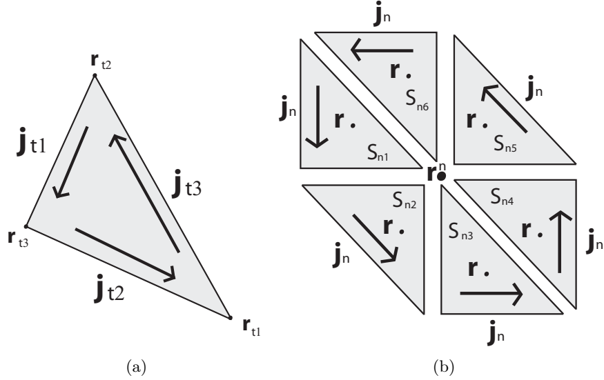
Figure 3.5: (a) Current basis vectors in one element; (b) Current basis vector associated to the n^{th} -node \mathbf{j}^n(\mathbf{r}) (its value depends on the particular element which \mathbf{r} lies in) .
