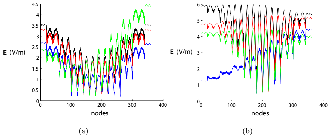
Figure 4.9: (a) E -field induced at the surface of a spherical conductor of radius 0.1 m described using a mesh of 360 elements and located at the coil centre by coil1(black), coil2(red), coil3(blue) and coil4(green);(b) E -field induced for the same sphere when placed at z=0.4 m ( G = 1\text{Tm}^{-1} , frequency = 500 Hz).
