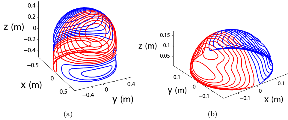
Figure 2.10: (a) Transverse dome and (b) hemispherical gradient coils.
