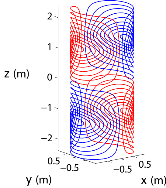
Figure 2.7: Transverse gradient coil designed using the target field method.
