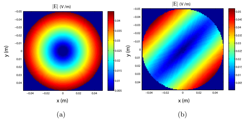
Figure 7.16: Electrostatic |\mathbf{E}| produced by the volume charges in an xy-plane inside the cylinder discretized into 1600 elements, rotating in a uniform magnetic field of 1T at a rate of 1 \text{ rad s}^{-1} (a) BEM computed electric field modulus produced by the charges using \mathbf{v} \times \mathbf{B} , (b) BEM computed electric field modulus produced by the charges using -(\mathbf{v} \cdot \nabla)\mathbf{A} .
