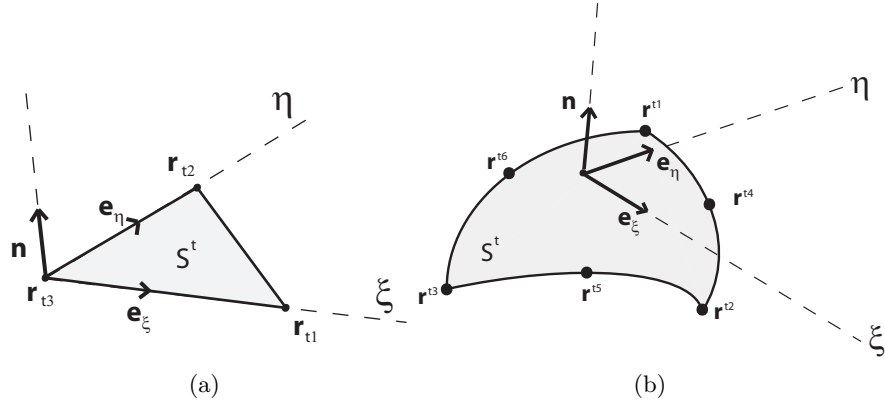
Figure 3.4: Coordinates system (\xi, \eta) .
