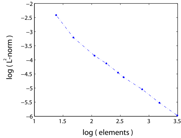
Figure 7.4: Convergence for the problem of a sphere shifted by 0.13m in the x-direction in a longitudinal field gradient in terms of the logarithm of the L^2 norm.
