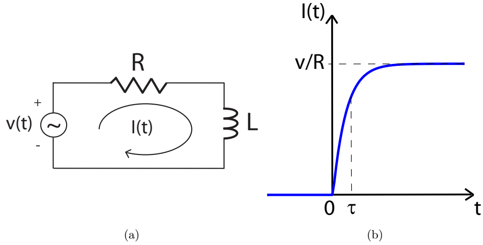
Figure 2.1: (a) RL-circuit ; (b) Evolution of the current intensity in a RL-circuit with the time .
