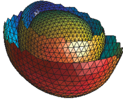
(b) Partial multi-domain showing meshed boundaries.
